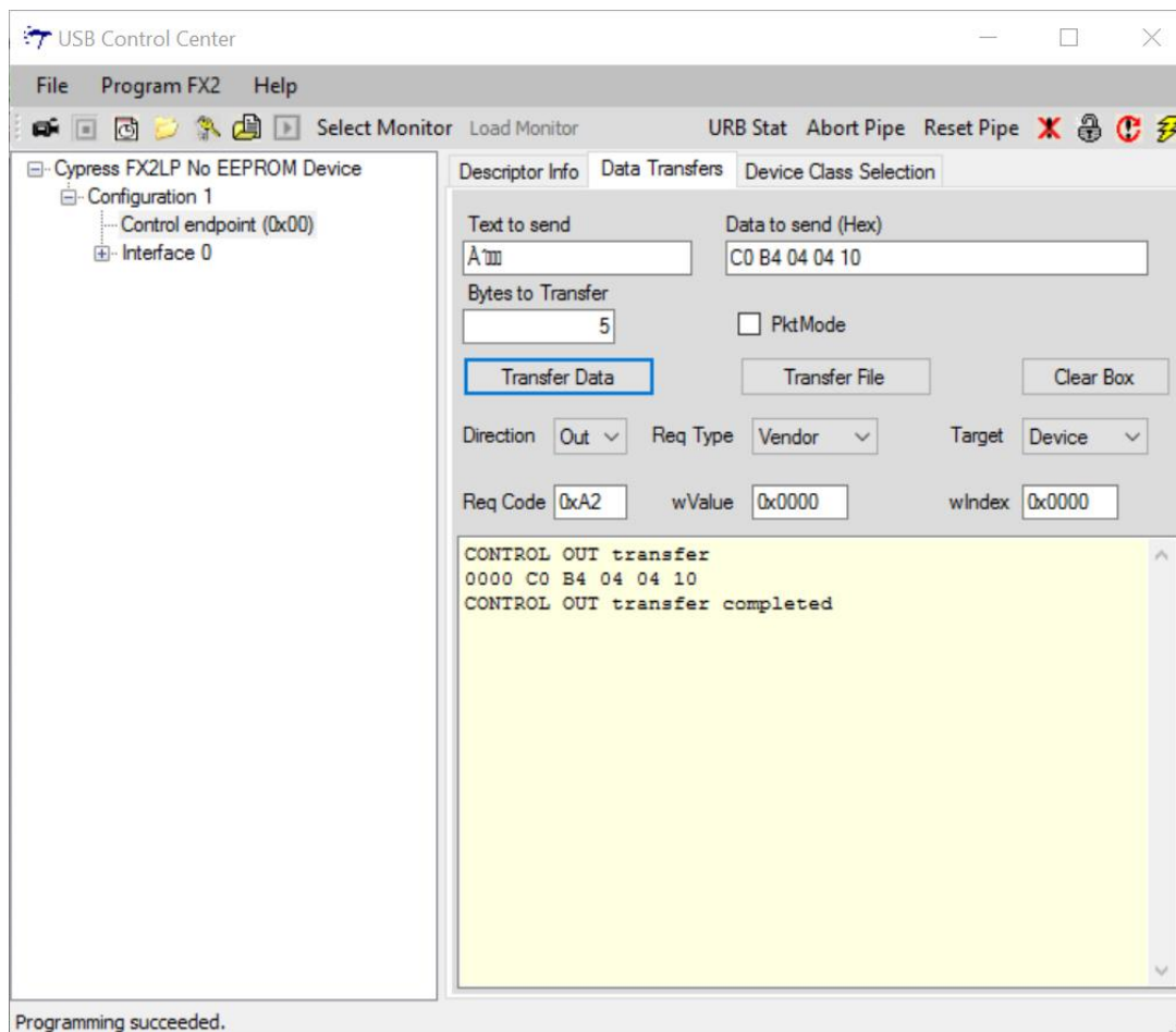
Figure 3. EEPROM Program
