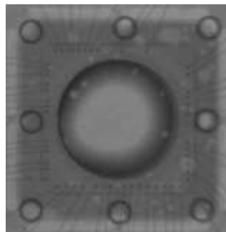
Figure 11. X-Ray of Moderate E-Pad Solder Connection
