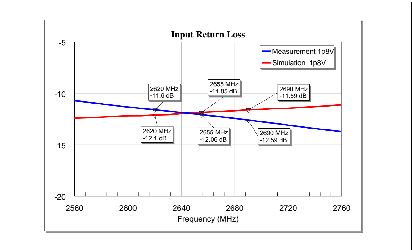
Figure 10 Input Matching of the BGA7H1N6 for LTE Band-7 Application at Vcc = 1.8 V
