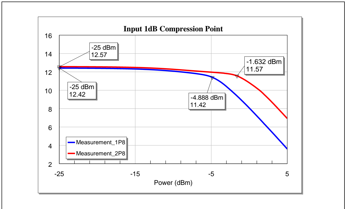
Figure 26 Input 1dB compression point of the BGA7H1N6 for LTE Band-7 Application
