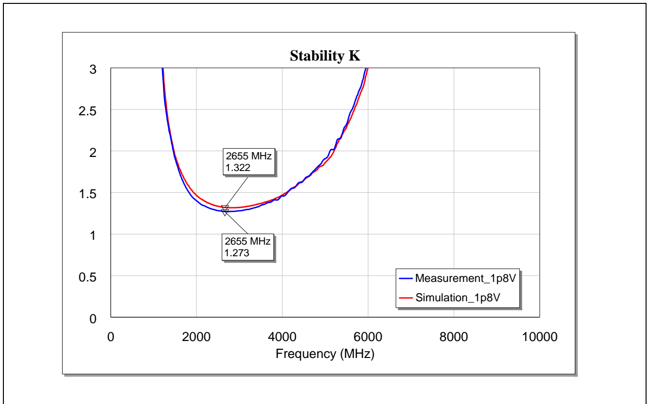
Figure 20 Stability K-factor of the BGA7H1N6 for LTE Band-7 Application at Vcc = 1.8 V
