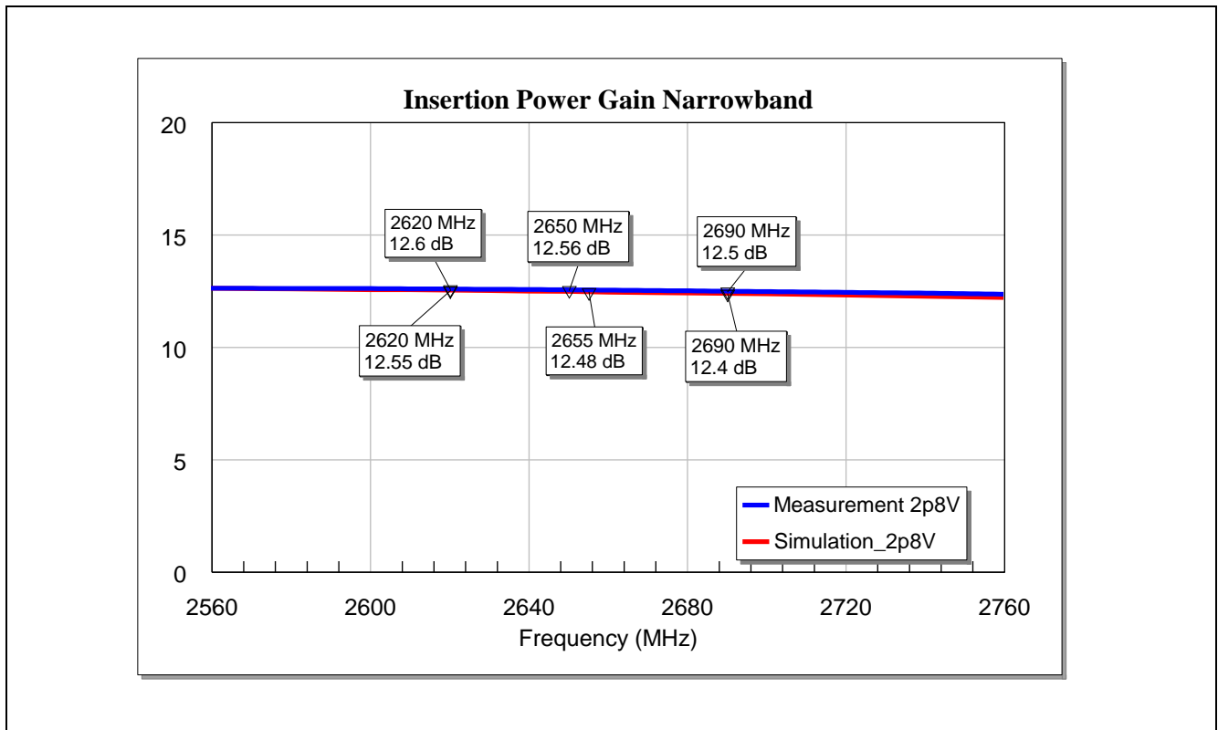
Figure 6 Insertion Power Gain (Narrowband) of the BGA7H1N6 for LTE Band-7 at Vcc = 2.8 V
