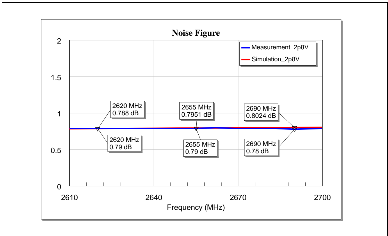
Figure 9 Noise Figure of the BGA7H1N6 for LTE Band-7 Application at Vcc = 2.8 V
