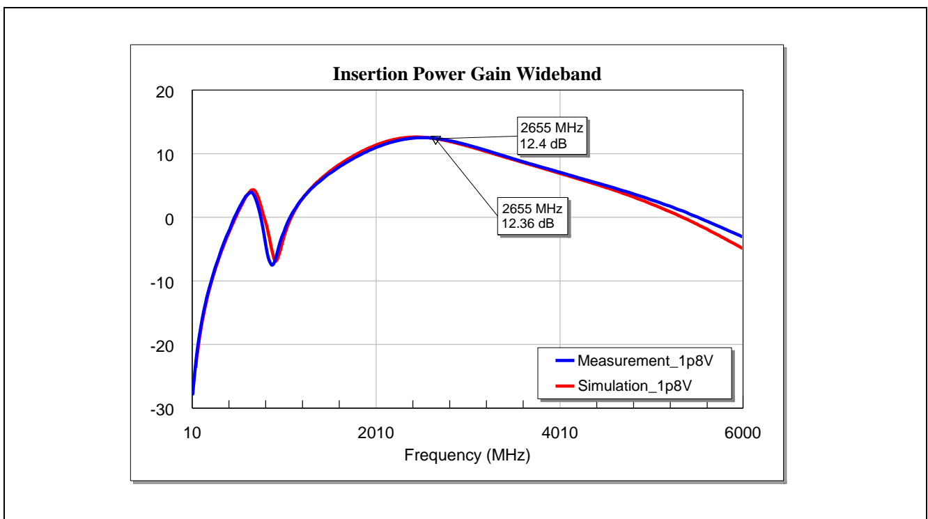
Figure 5 Insertion Power Gain (Wideband) of the BGA7H1N6 for LTE Band-7 at Vcc = 1.8 V
