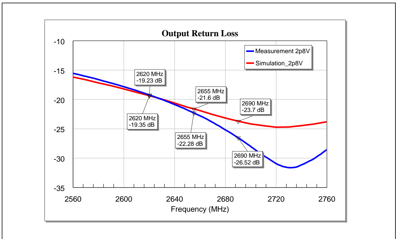
Figure 15 Output Matching of the BGA7H1N6 for LTE Band-7 Application at Vcc = 2.8 V
