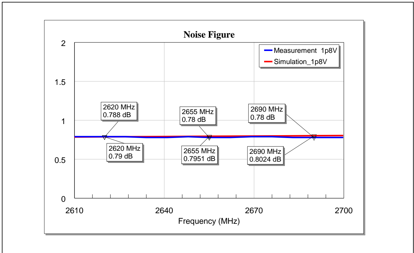
Figure 8 Noise Figure of the BGA7H1N6 for LTE Band-7 Application at Vcc = 1.8 V
