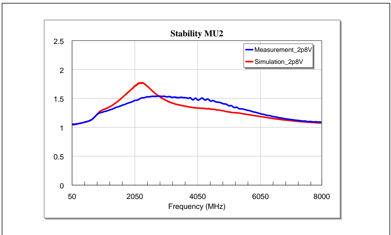
Figure 25 Stability Mu2-factor of the BGA7H1N6 for LTE Band-7 Application at Vcc = 2.8 V
