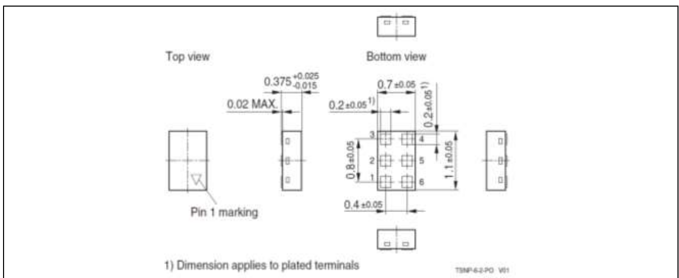
Figure 2 Package and pin connections of BGA7H1N6
