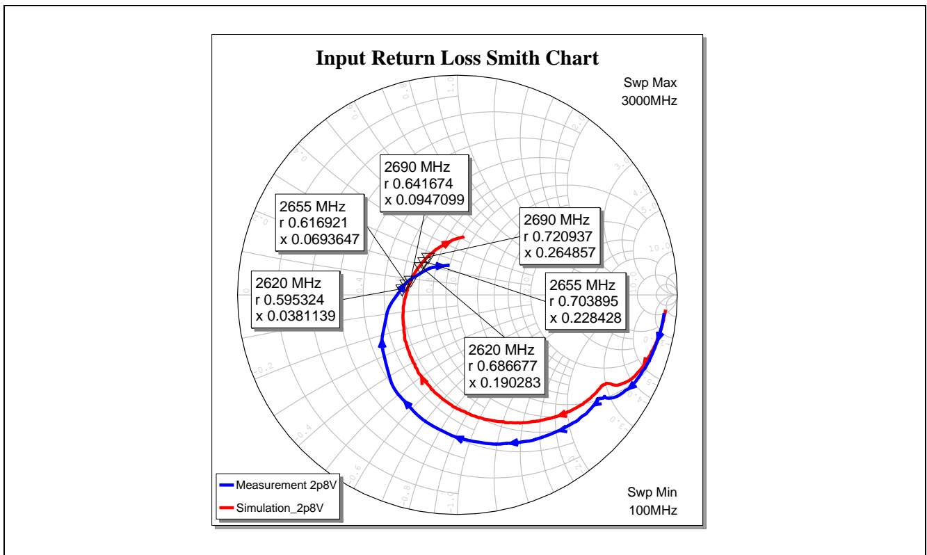
Figure 13 Input Matching (Smith Chart) of the BGA7H1N6 for LTE Band-7 Application at Vcc = 2.8 V
