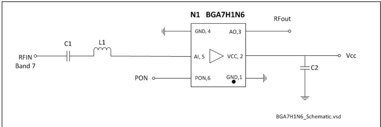
Figure 3 Schematics of the BGA7H1N6 Application Circuit
