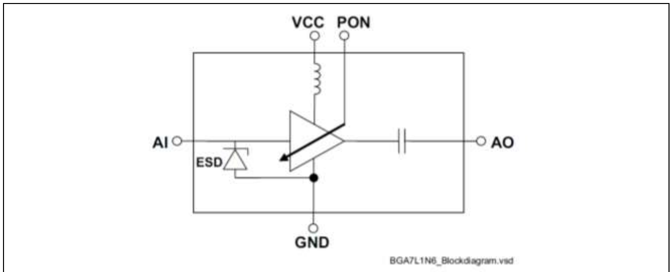
Figure 1 Equivalent Circuit of BGA7H1N6
