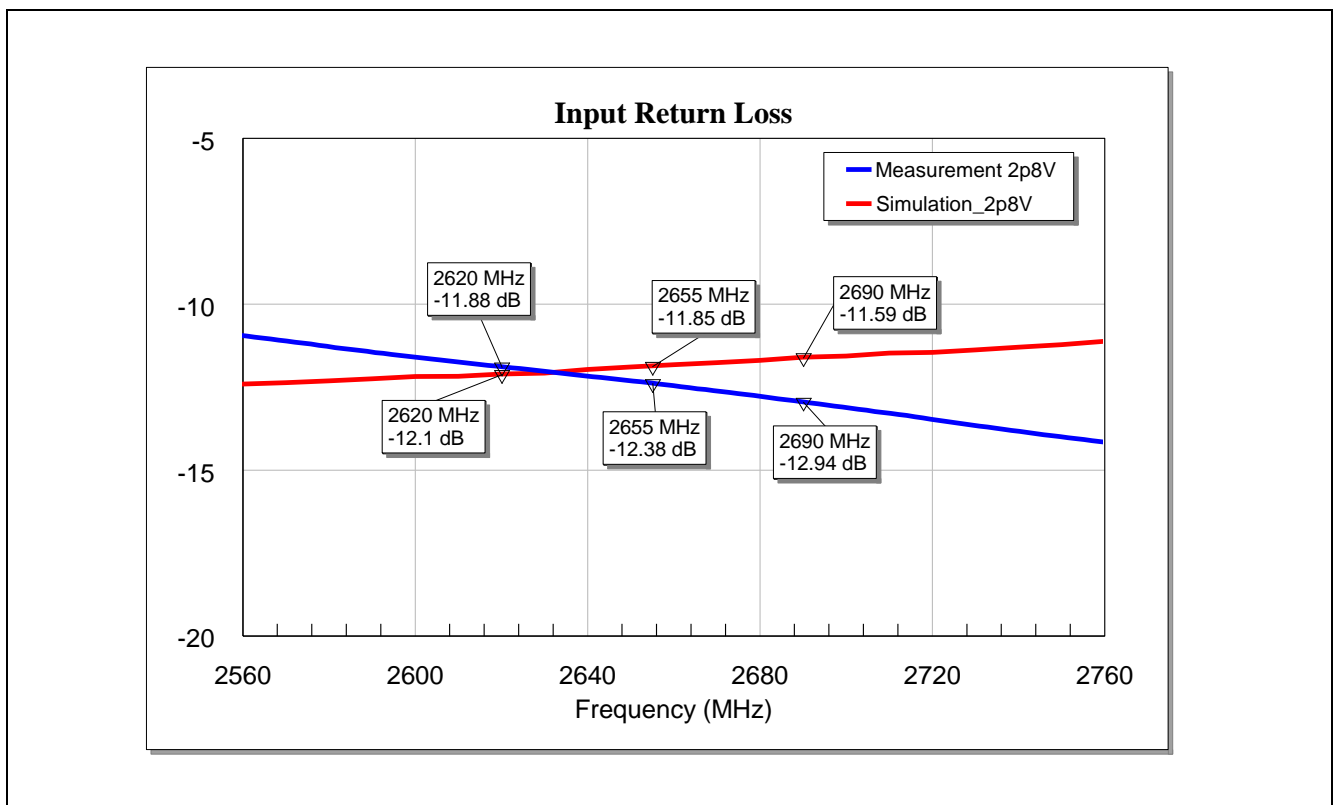
Figure 11 Input Matching of the BGA7H1N6 for LTE Band-7 Application at Vcc = 2.8 V
