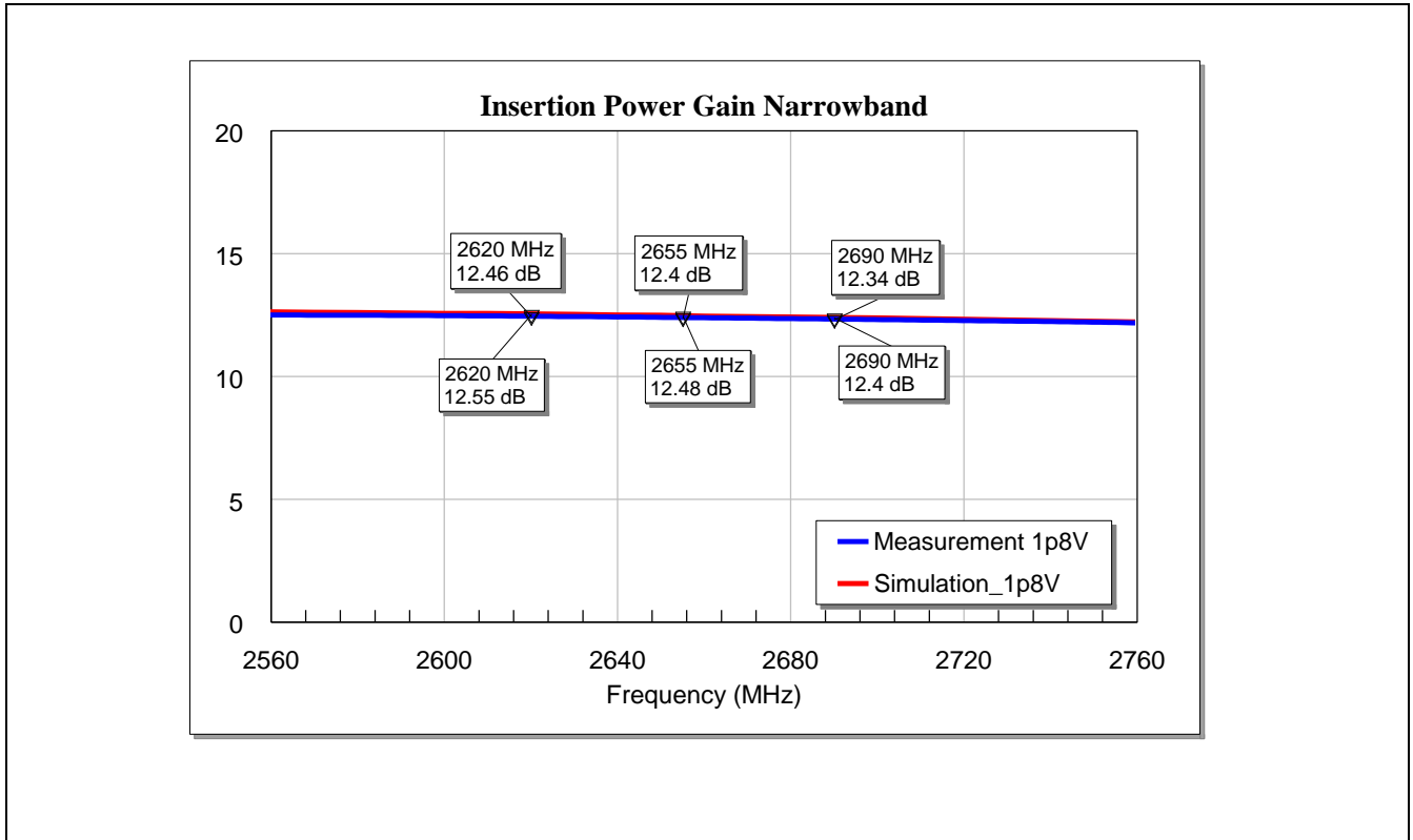
Figure 4 Insertion Power Gain (Narrowband) of the BGA7H1N6 for LTE Band-7 at Vcc = 1.8 V
