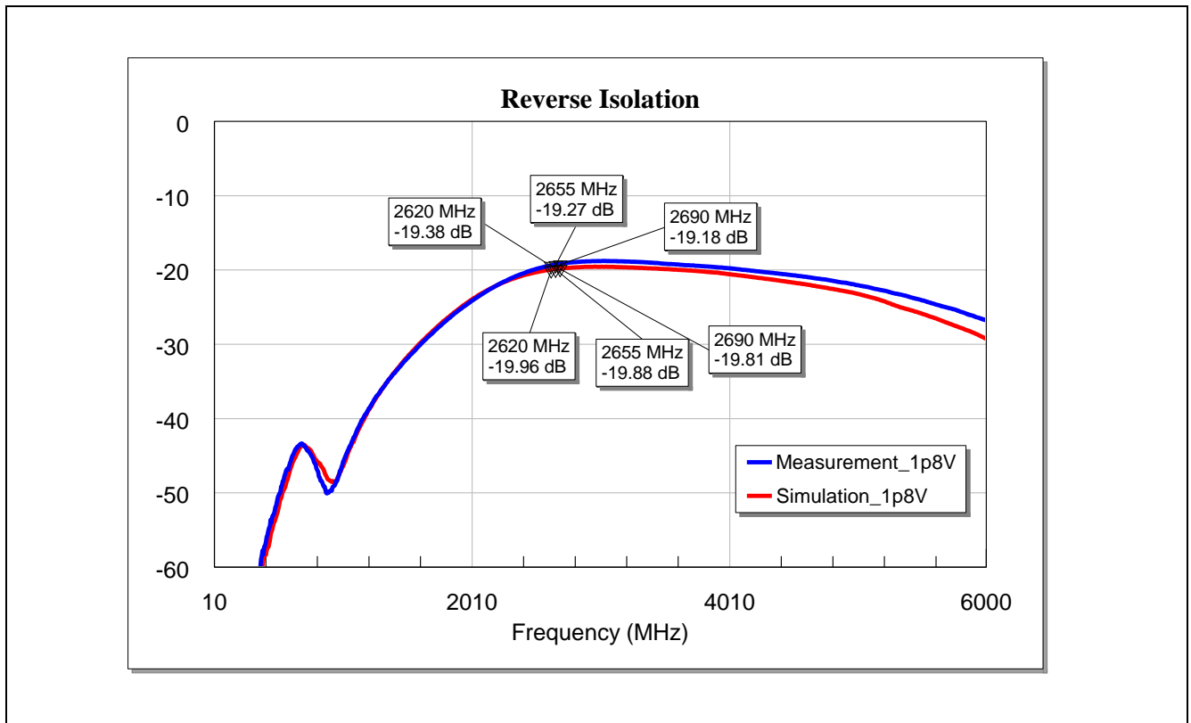
Figure 18 Reverse Isolation of the BGA7H1N6 for LTE Band-7 Application at Vcc = 1.8 V
