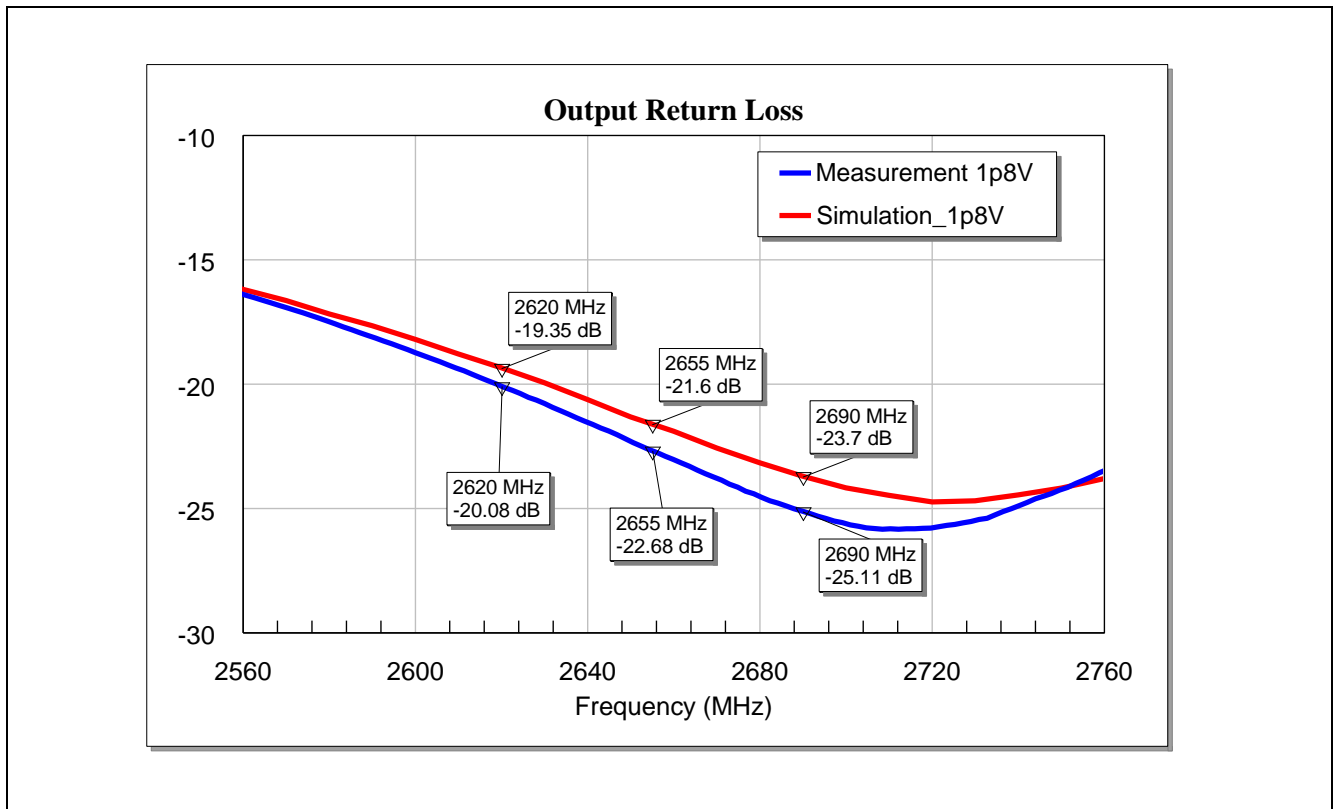
Figure 14 Output Matching of the BGA7H1N6 for LTE Band-7 Application at Vcc = 1.8 V
