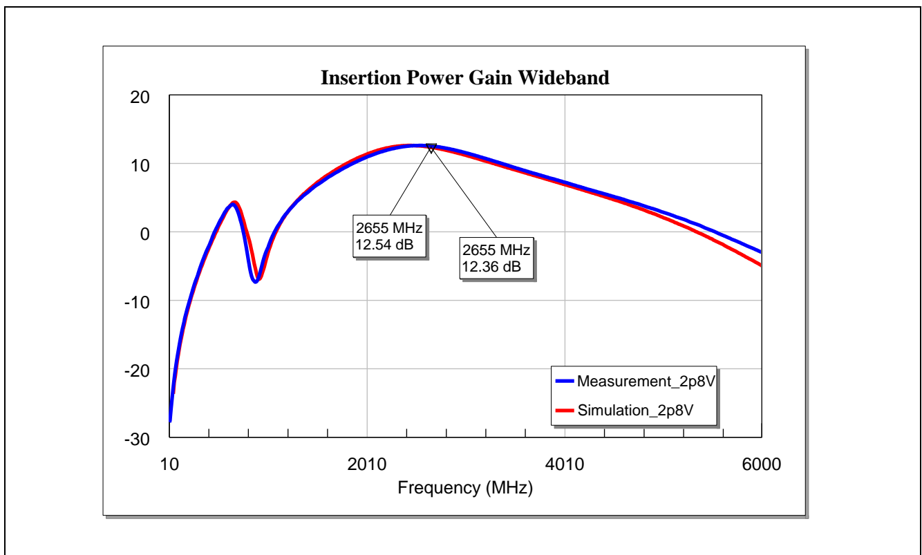
Figure 7 Insertion Power Gain (Wideband) of the BGA7H1N6 for LTE Band-7 at Vcc = 2.8 V
