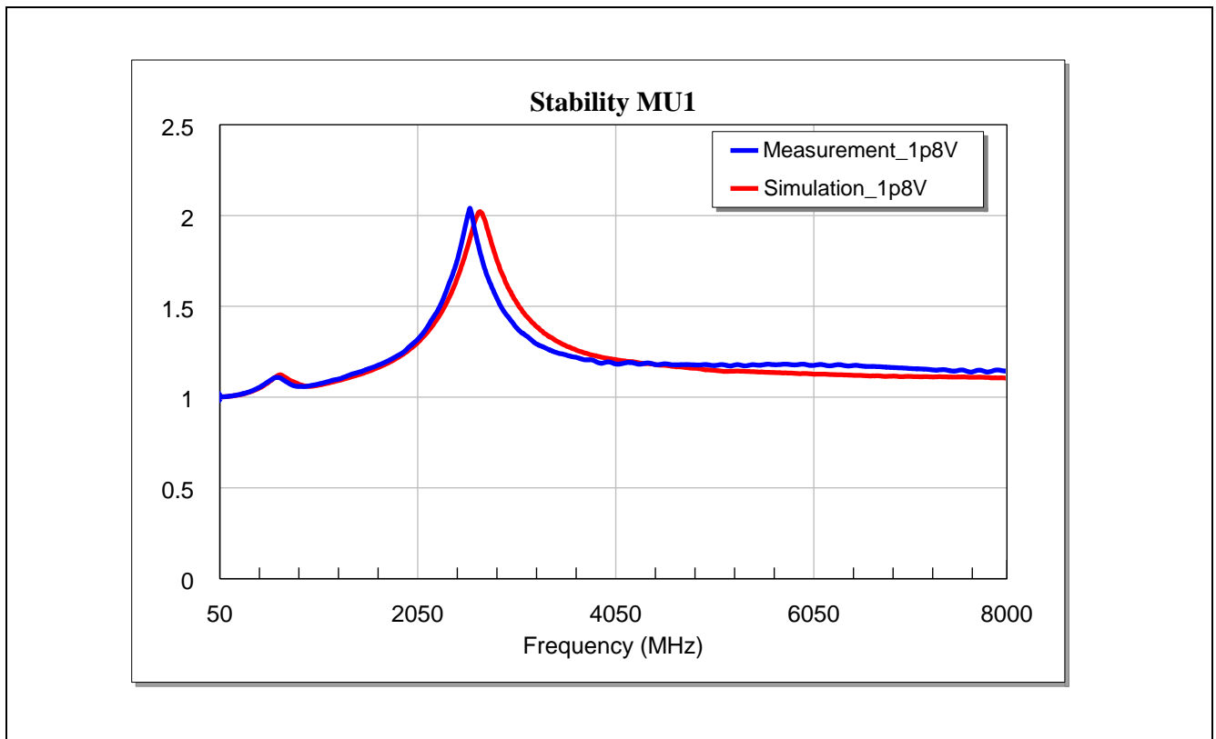
Figure 22 Stability Mu1-factor of the BGA7H1N6 for LTE Band-7 Application at Vcc = 1.8 V
