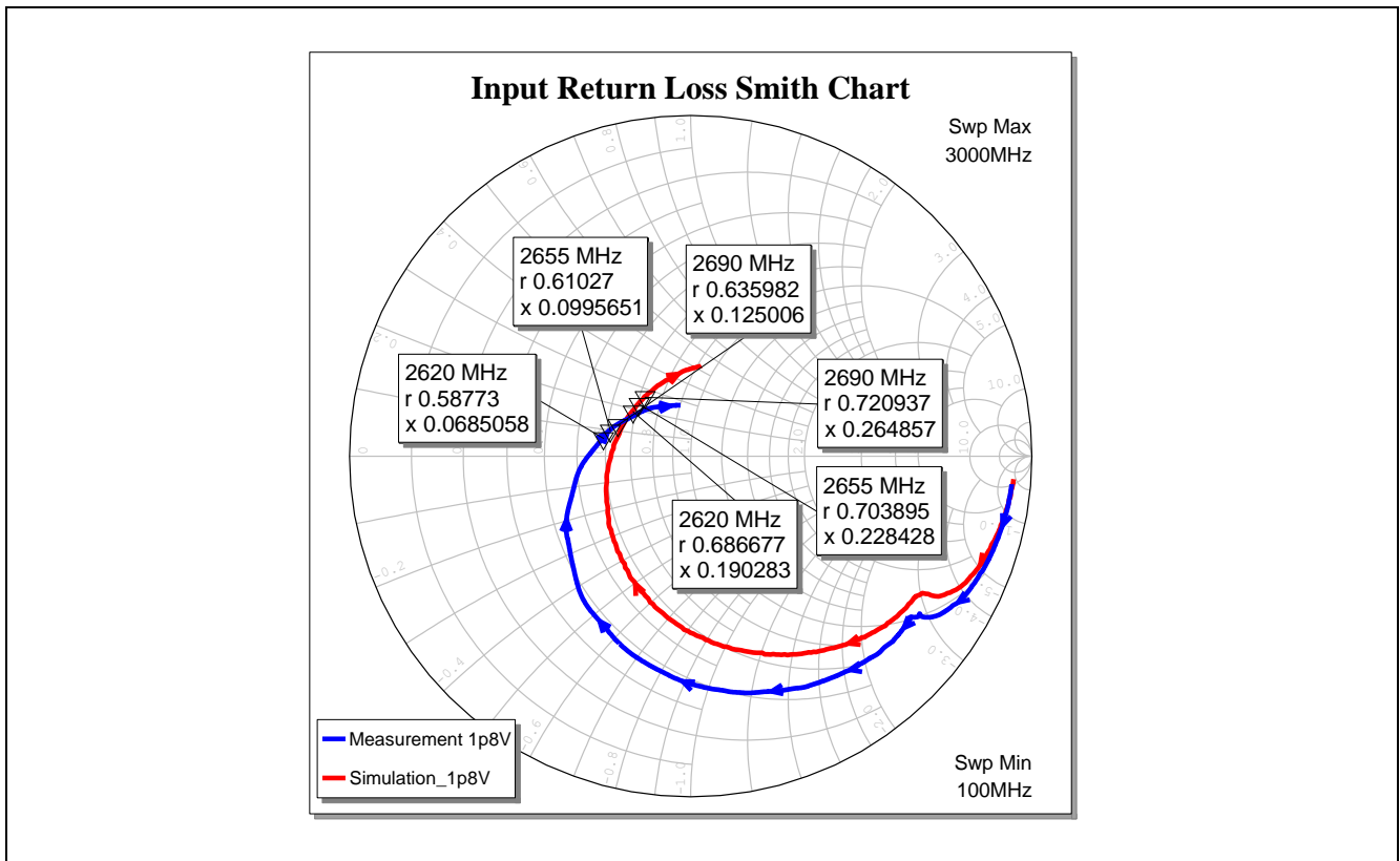
Figure 12 Input Matching (Smith Chart) of the BGA7H1N6 for LTE Band-7 Application at Vcc = 1.8 V
