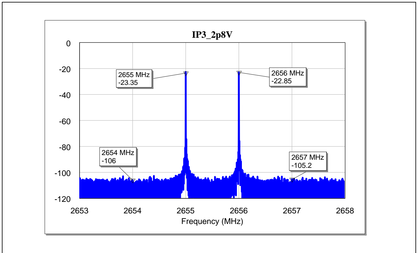
Figure 28 Input 3 rd interception point of the BGA7H1N6 for LTE Band-7 Application at Vcc=2.8 V
