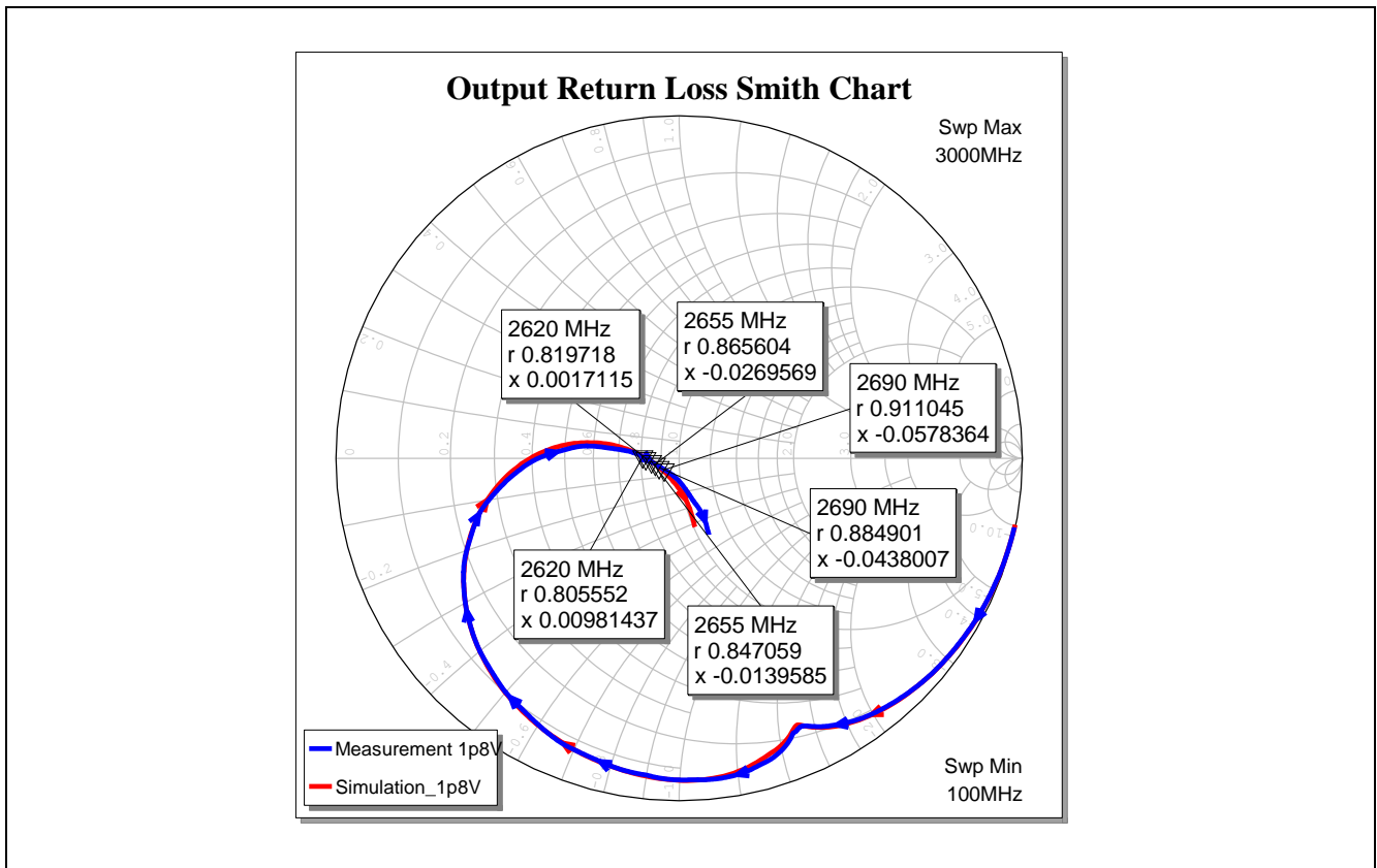
Figure 16 Output Matching (Smith Chart) of the BGA7H1N6 for LTE Band-7 Application at Vcc = 1.8 V
