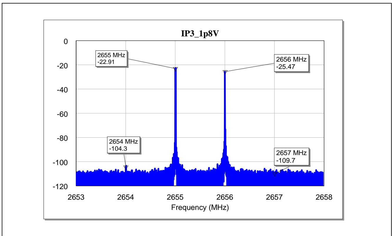
Figure 27 Input 3 rd interception point of the BGA7H1N6 for LTE Band-7 Application at Vcc=1.8 V
