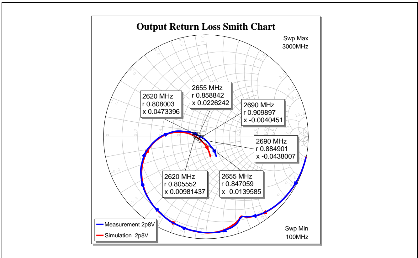
Figure 17 Output Matching (Smith Chart) of the BGA7H1N6 for LTE Band-7 Application at Vcc = 2.8 V
