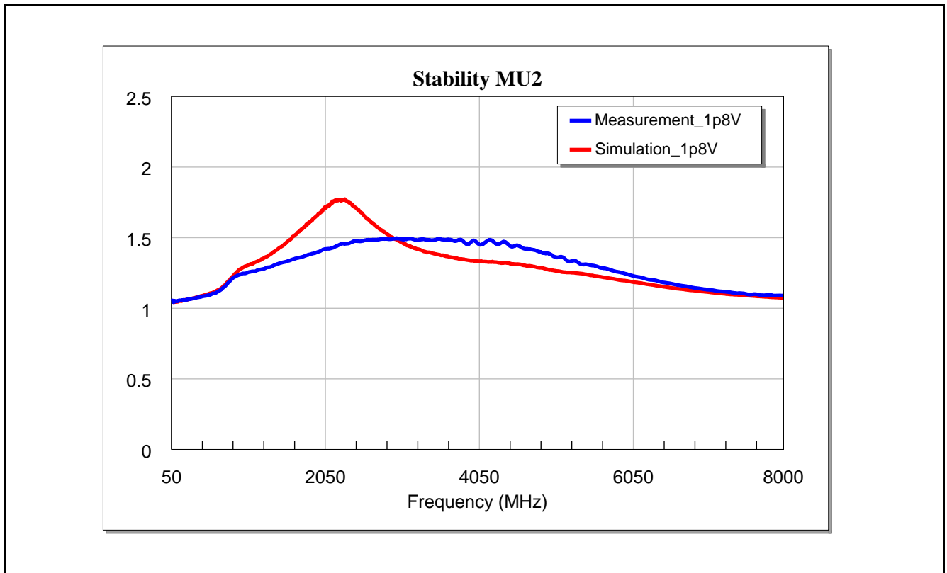
Figure 24 Stability Mu2-factor of the BGA7H1N6 for LTE Band-7 Application at Vcc = 1.8 V
