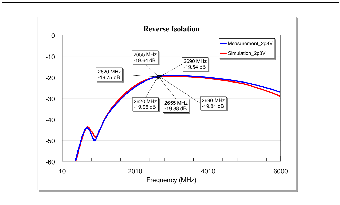
Figure 19 Reverse Isolation of the BGA7H1N6 for LTE Band-7 Application at Vcc = 2.8 V
