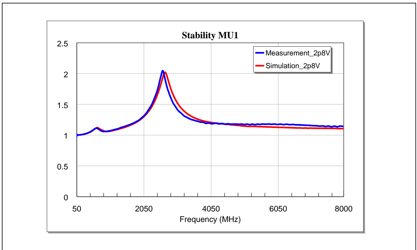
Figure 23 Stability Mu1-factor of the BGA7H1N6 for LTE Band-7 Application at Vcc = 2.8 V
