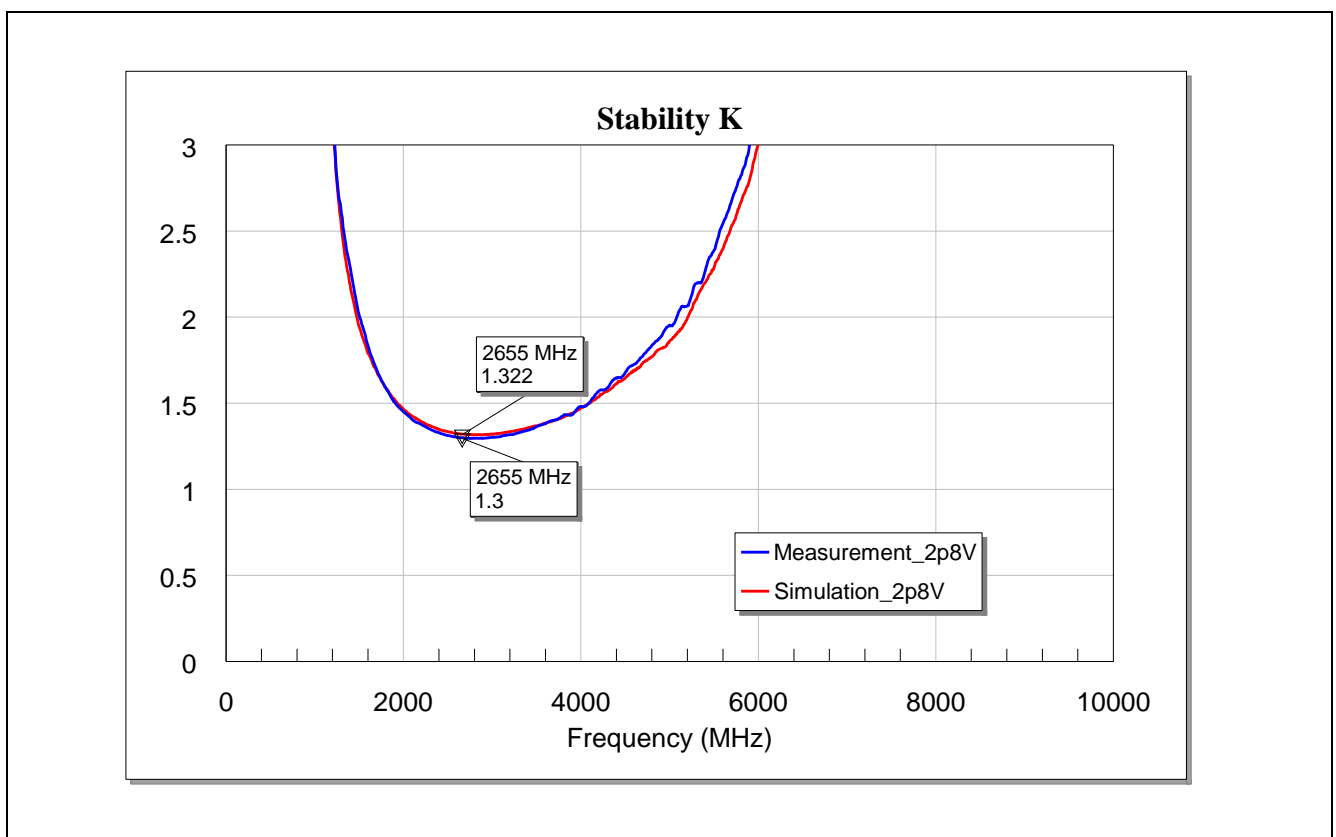
Figure 21 Stability K-factor of the BGA7H1N6 for LTE Band-7 Application at Vcc = 2.8 V
