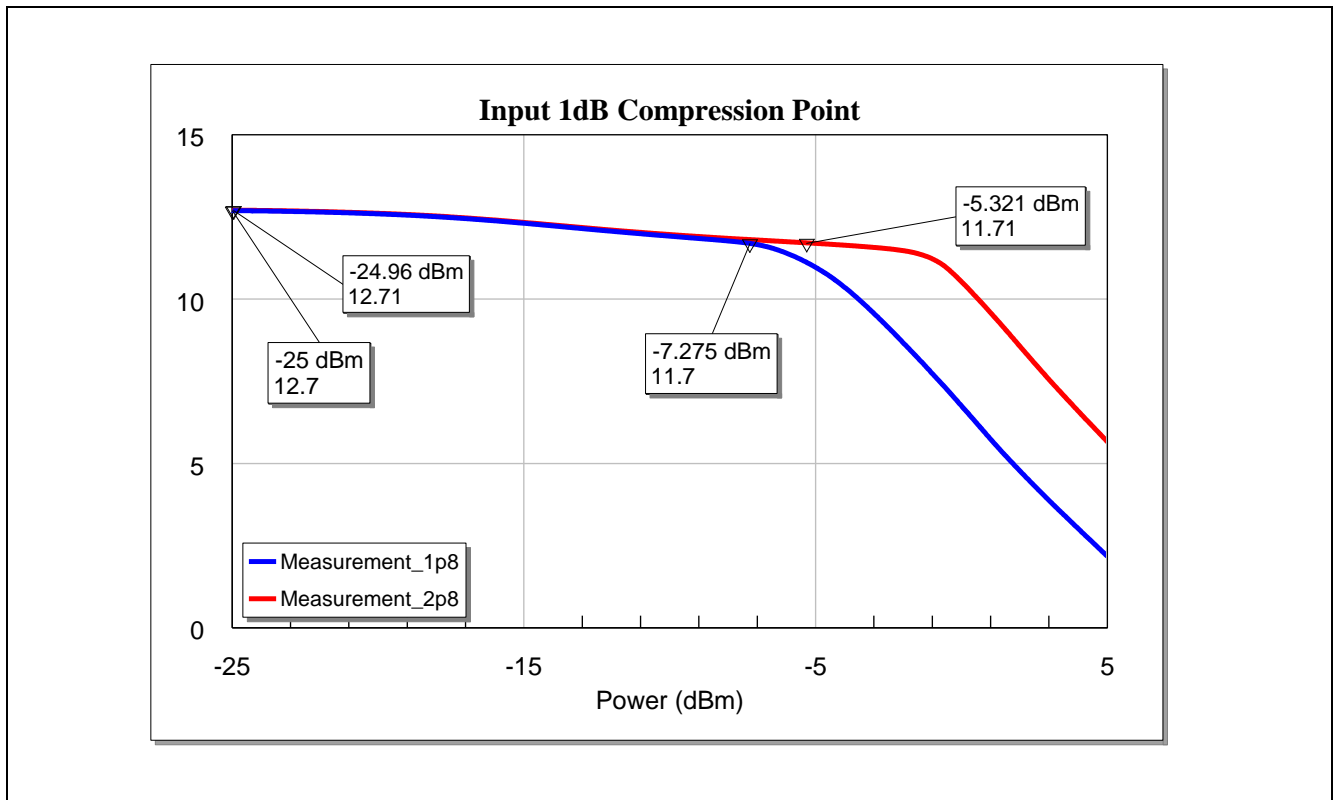
Figure 26 Input 1dB compression point of the BGA7L1N6 for LTE Band-26 Application
