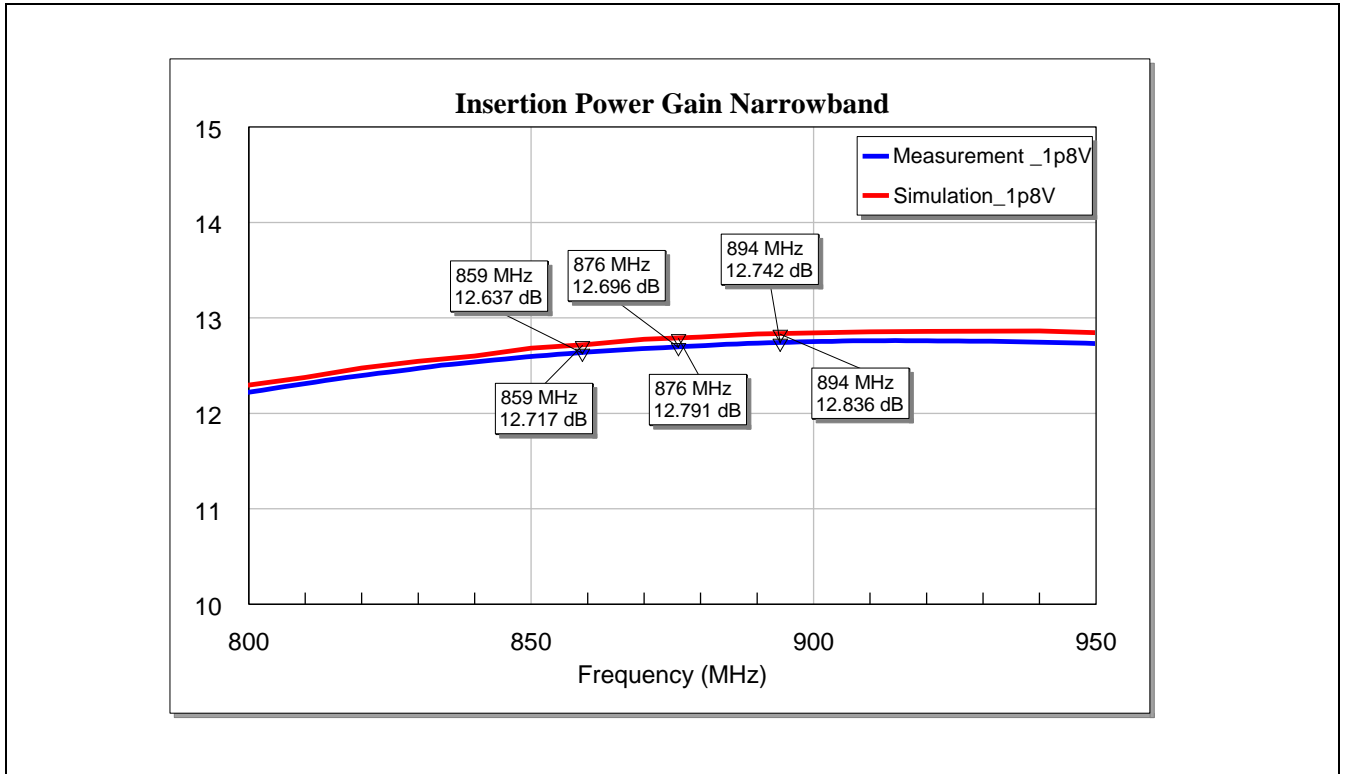
Figure 4 Insertion Power Gain (Narrowband) of the BGA7L1N6 for LTE Band-26 at Vcc = 1.8 V
