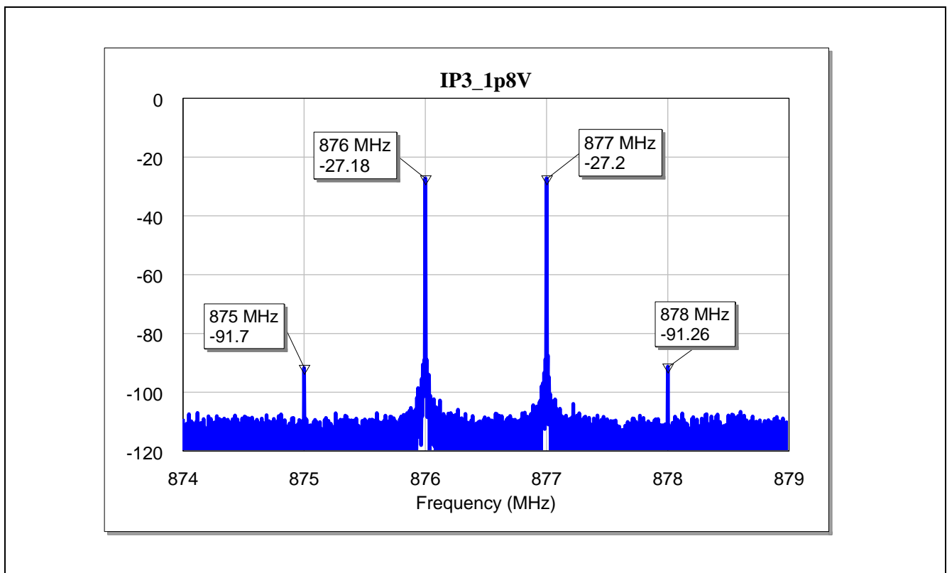
Figure 27 Input 3 rd interception point of the BGA7L1N6 for LTE Band-26 Application at Vcc=1.8 V
