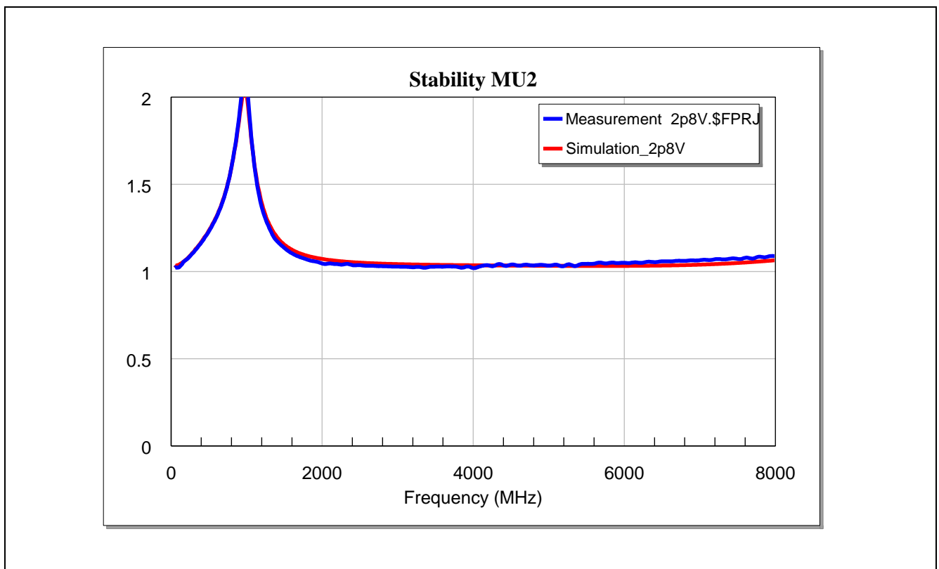
Figure 25 Stability Mu2-factor of the BGA7L1N6 for LTE Band-26 Application at Vcc = 2.8 V
