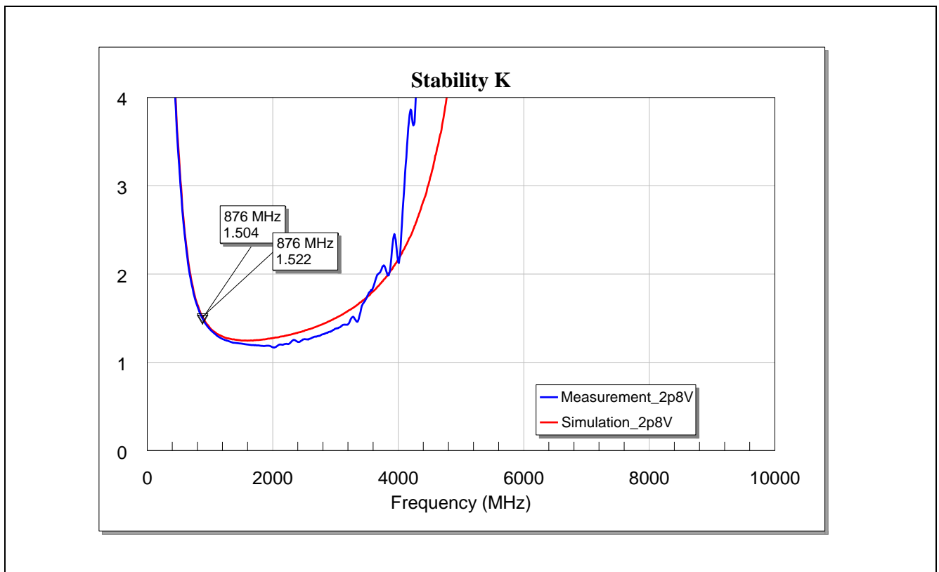
Figure 21 Stability K-factor of the BGA7L1N6 for LTE Band-26 Application at Vcc = 2.8 V
