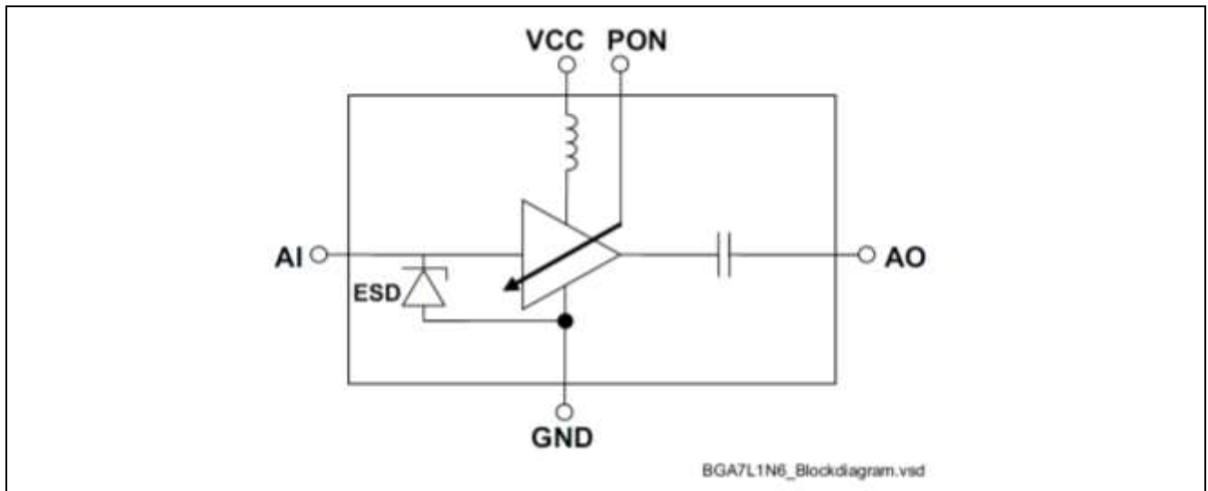
Figure 1 Equivalent Circuit of BGA7L1N6
