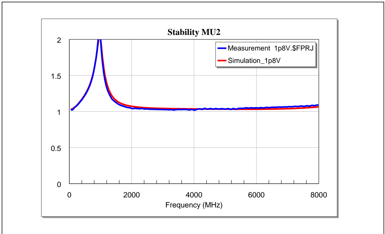
Figure 24 Stability Mu2-factor of the BGA7L1N6 for LTE Band-26 Application at Vcc = 1.8 V
