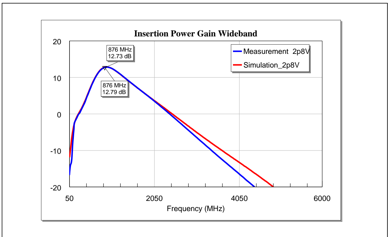
Figure 7 Insertion Power Gain (Wideband) of the BGA7L1N6 for LTE Band-26 at V_{cc} = 2.8\text{ V}
