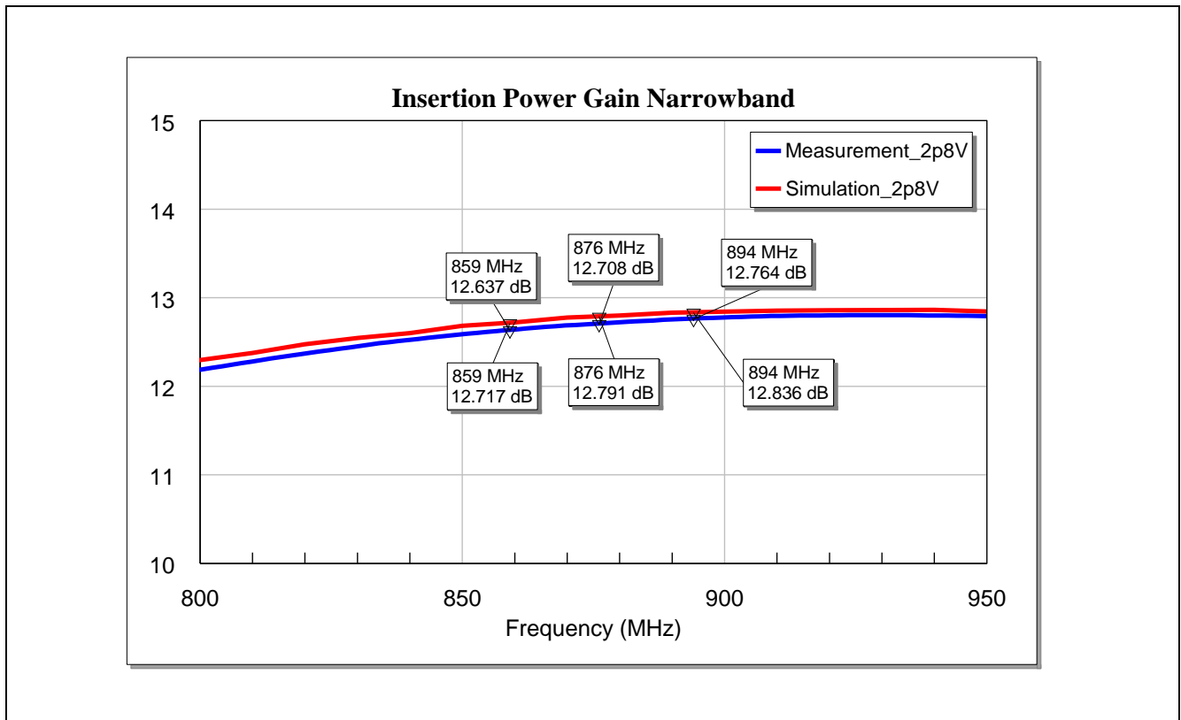
Figure 6 Insertion Power Gain (Narrowband) of the BGA7L1N6 for LTE Band-26 at V_{cc} = 2.8\text{ V}
