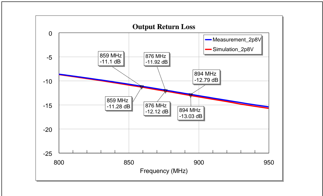
Figure 14 Output Matching of the BGA7L1N6 for LTE Band-26 Application at Vcc = 1.8 V
