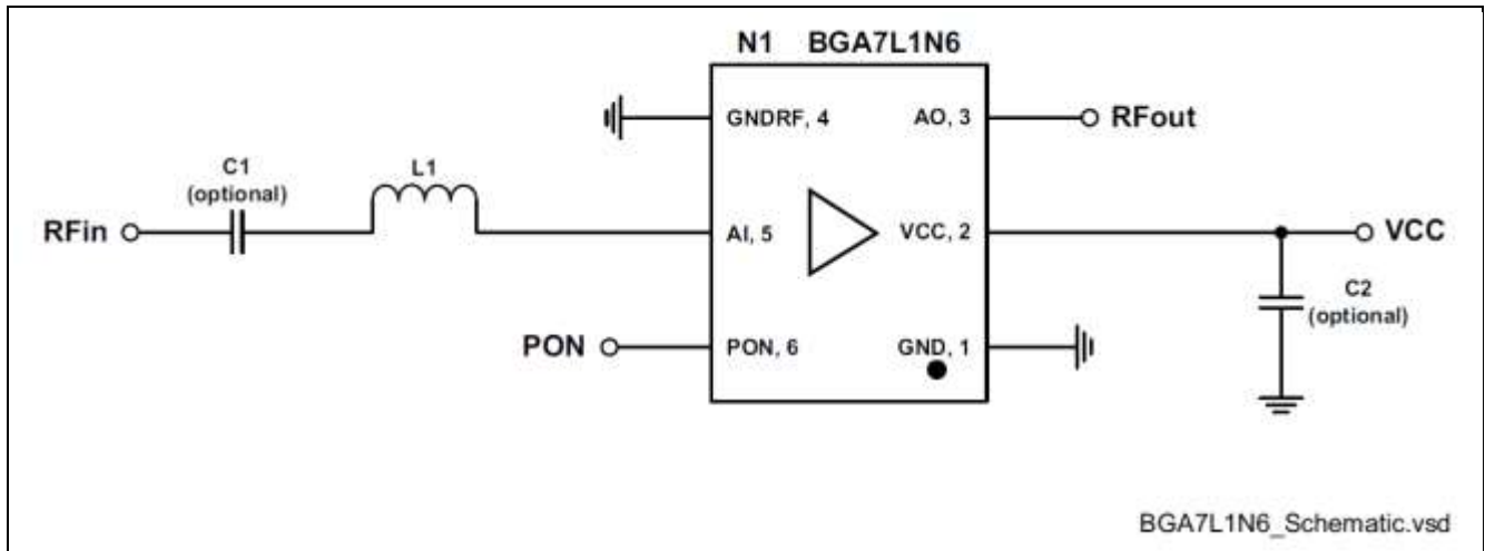
Figure 3 Schematics of the BGA7L1N6 Application Circuit
