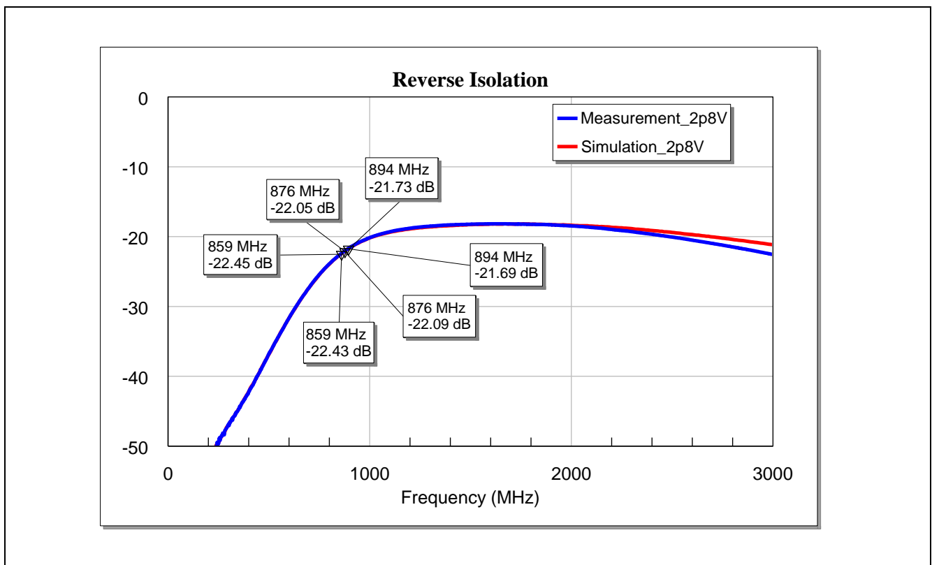
Figure 19 Reverse Isolation of the BGA7L1N6 for LTE Band-26 Application at Vcc = 2.8 V
