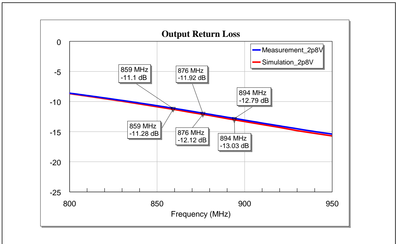
Figure 15 Output Matching of the BGA7L1N6 for LTE Band-26 Application at Vcc = 2.8 V
