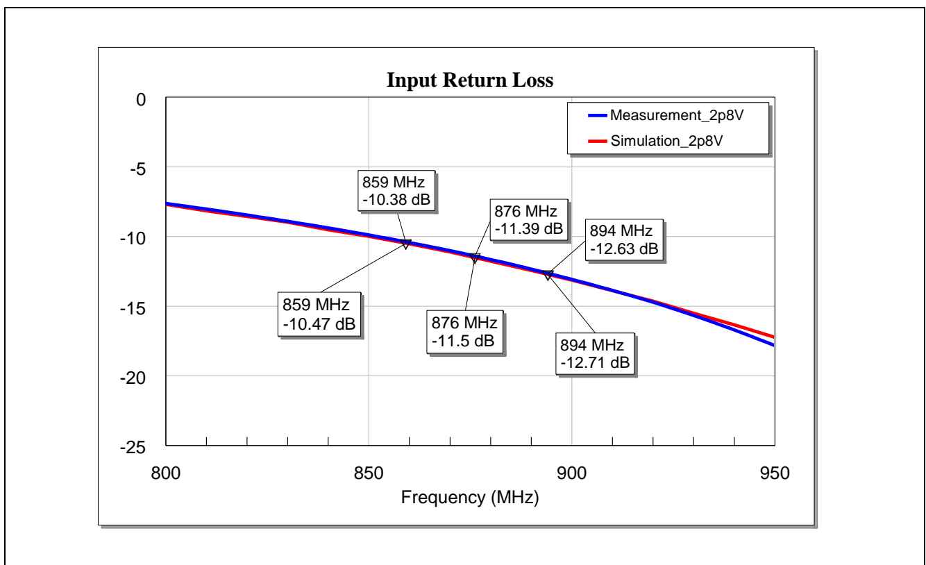
Figure 11 Input Matching of the BGA7L1N6 for LTE Band-26 Application at Vcc = 2.8 V
