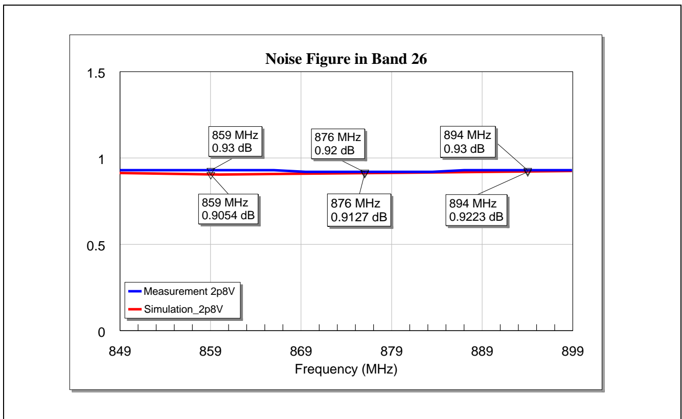
Figure 9 Noise Figure of the BGA7L1N6 for LTE Band-26 Application at Vcc = 2.8 V
