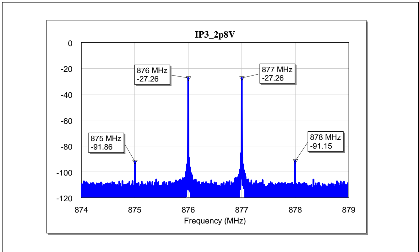
Figure 28 Input 3 rd interception point of the BGA7L1N6 for LTE Band-26 Application at Vcc=2.8 V
