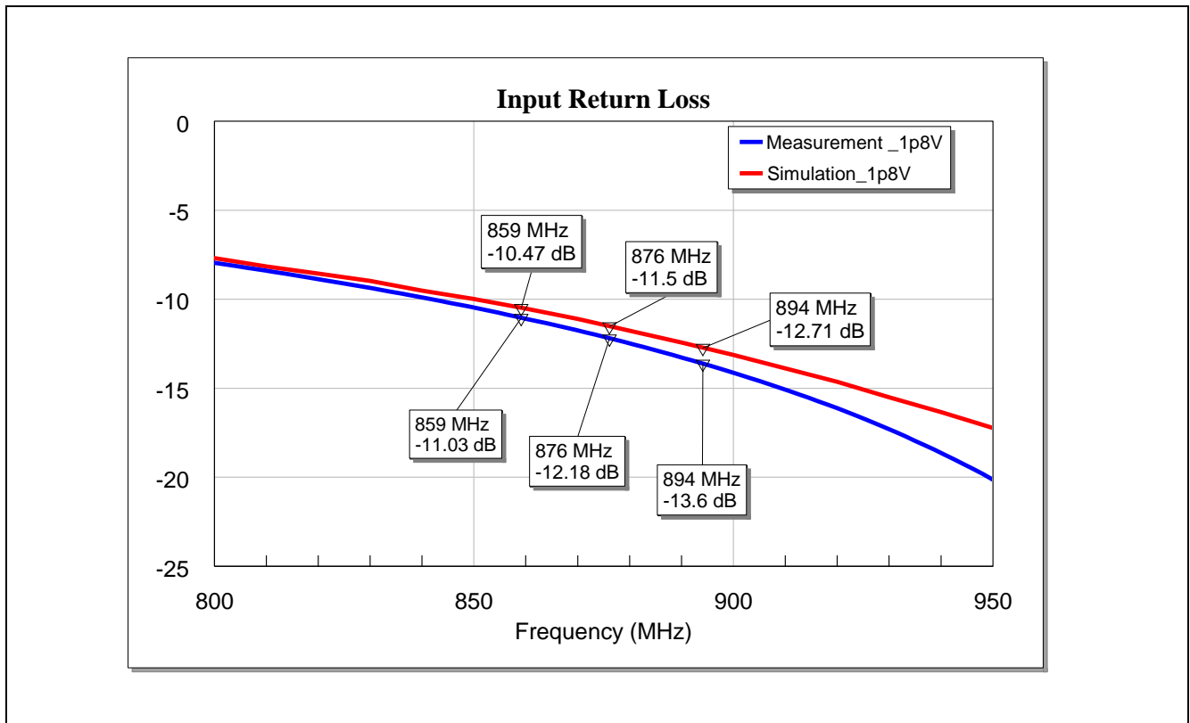
Figure 10 Input Matching of the BGA7L1N6 for LTE Band-26 Application at Vcc = 1.8 V
