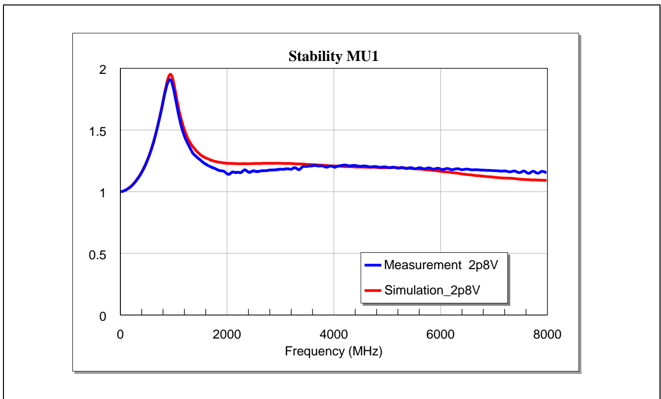
Figure 23 Stability Mu1-factor of the BGA7L1N6 for LTE Band-26 Application at Vcc = 2.8 V
