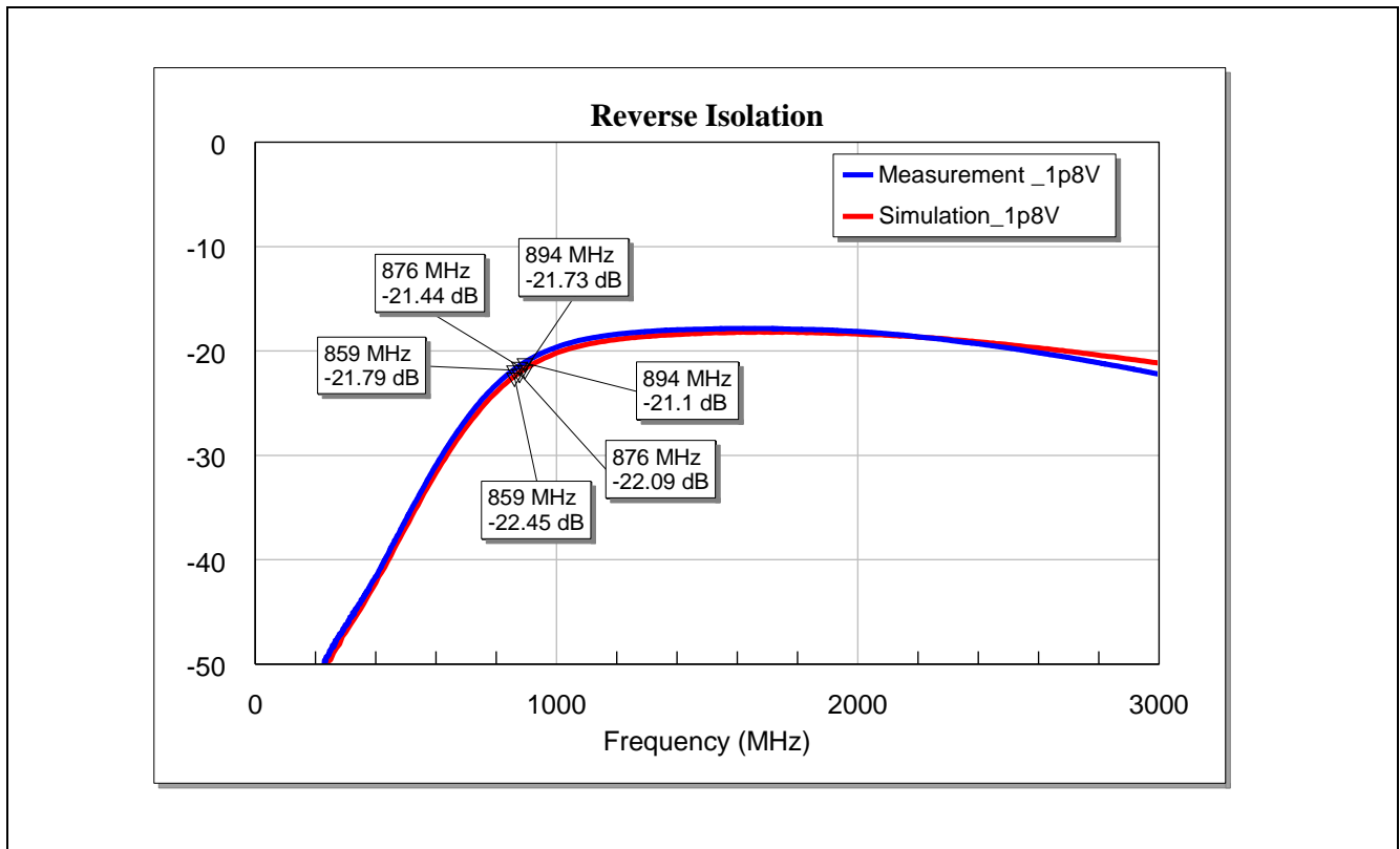
Figure 18 Reverse Isolation of the BGA7L1N6 for LTE Band-26 Application at Vcc = 1.8 V
