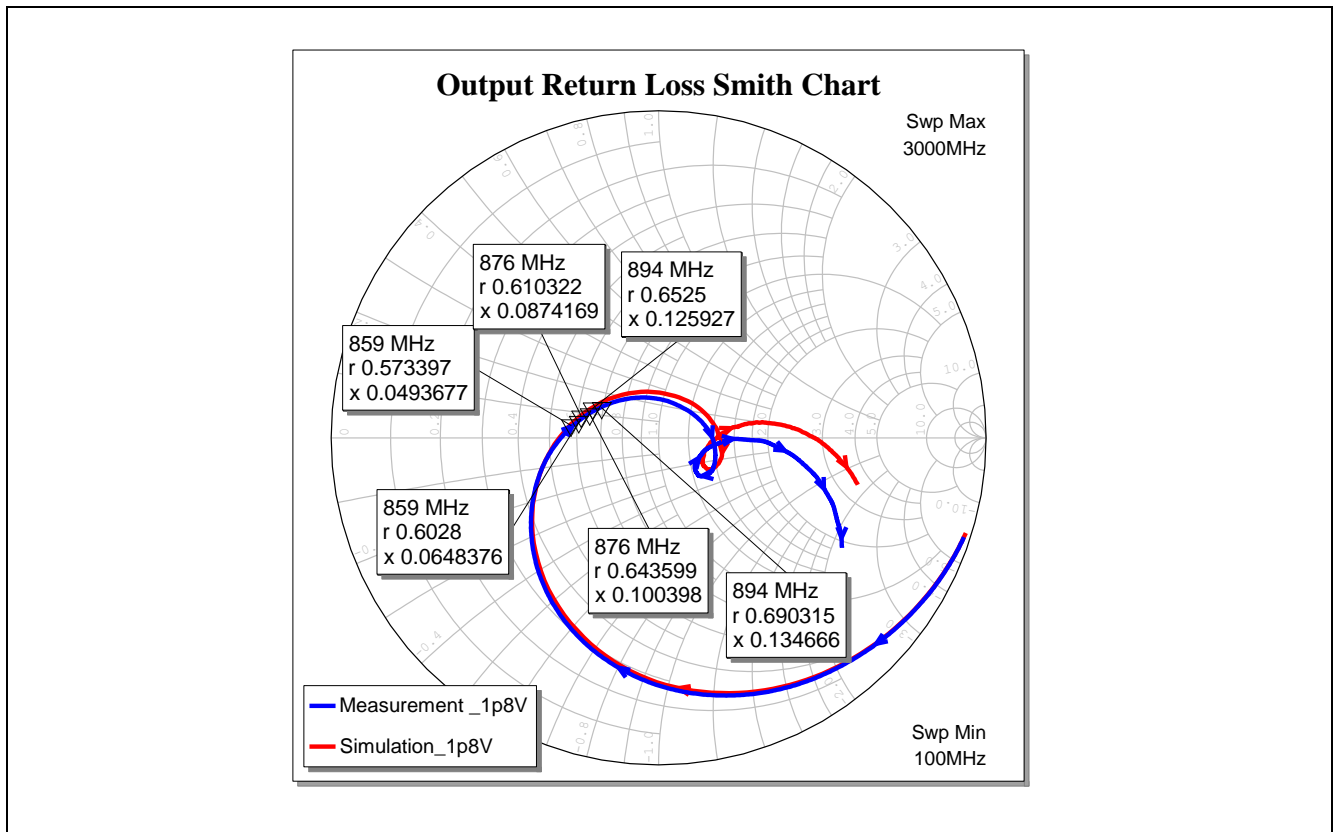
Figure 16 Output Matching (Smith Chart) of the BGA7L1N6 for LTE Band-26 Application at Vcc = 1.8 V
