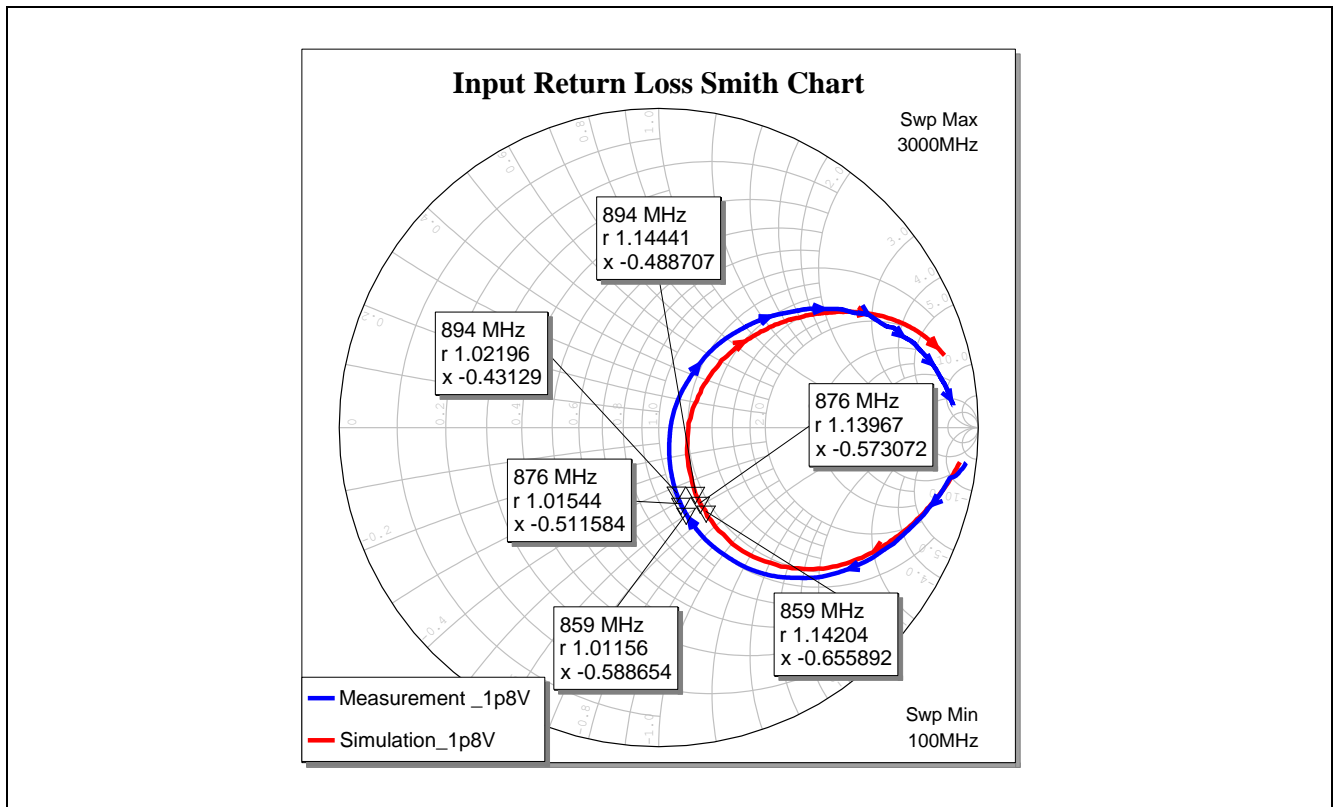
Figure 12 Input Matching (Smith Chart) of the BGA7L1N6 for LTE Band-26 Application at Vcc = 1.8 V
