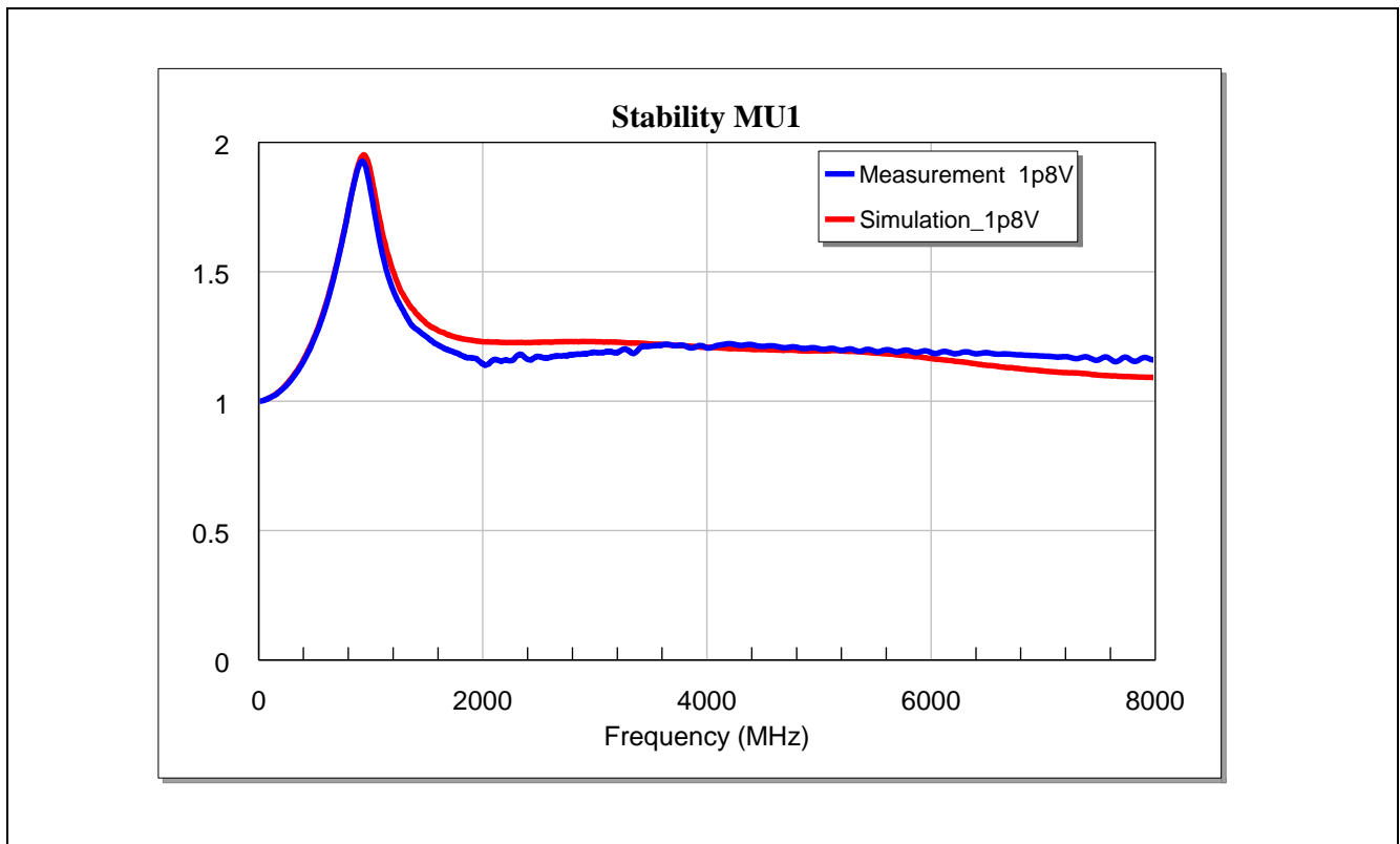
Figure 22 Stability Mu1-factor of the BGA7L1N6 for LTE Band-26 Application at Vcc = 1.8 V
