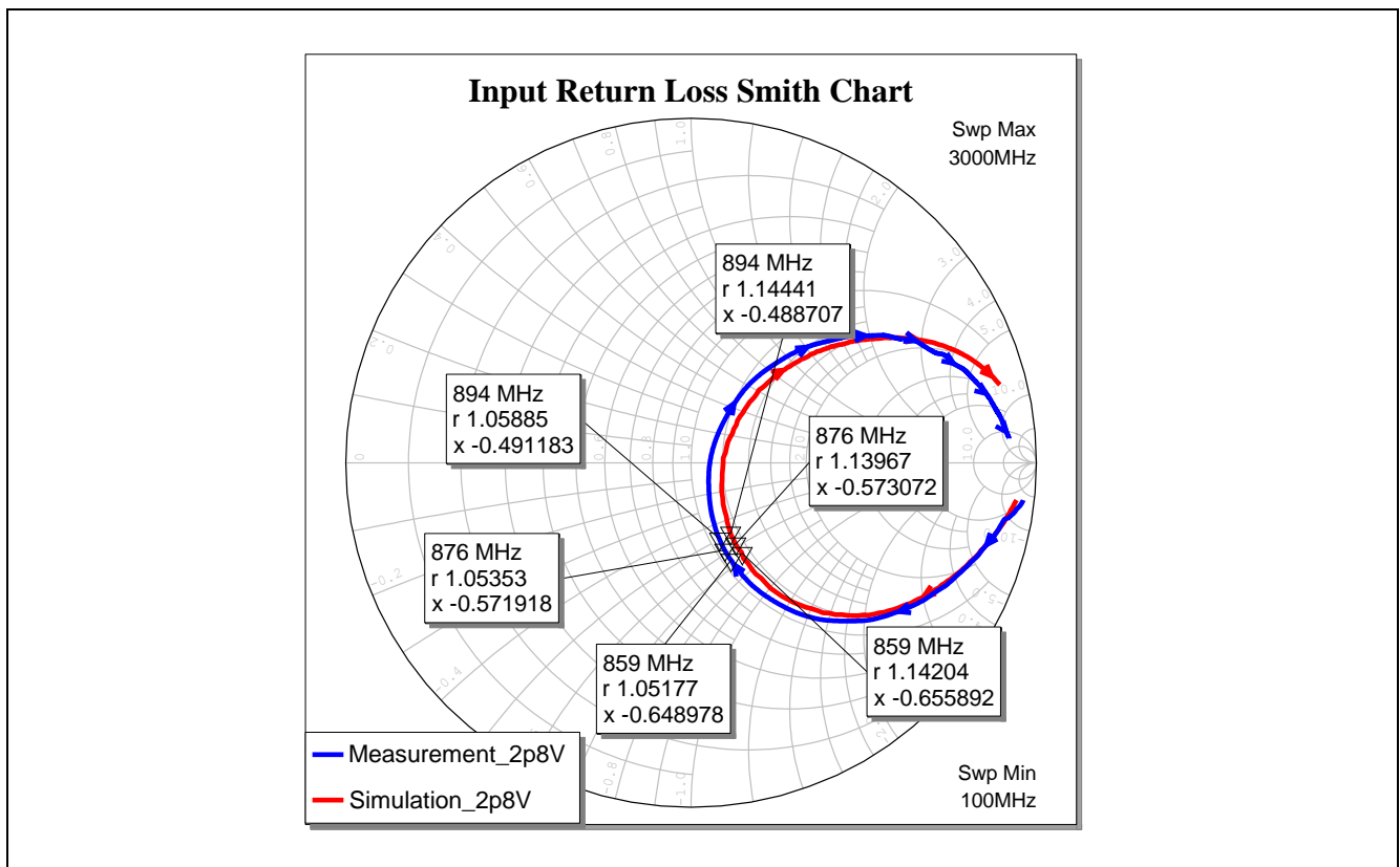
Figure 13 Input Matching (Smith Chart) of the BGA7L1N6 for LTE Band-26 Application at Vcc = 2.8 V
