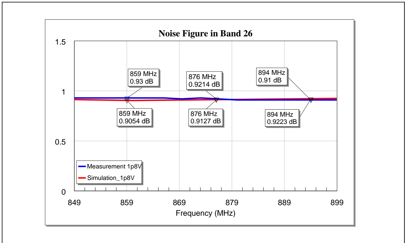
Figure 8 Noise Figure of the BGA7L1N6 for LTE Band-26 Application at Vcc = 1.8 V
