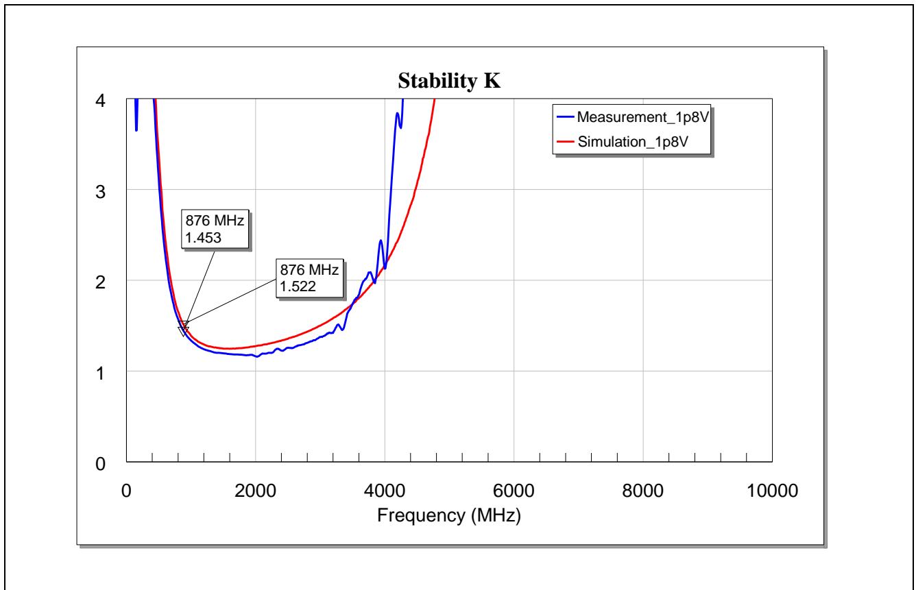
Figure 20 Stability K-factor of the BGA7L1N6 for LTE Band-26 Application at Vcc = 1.8 V
