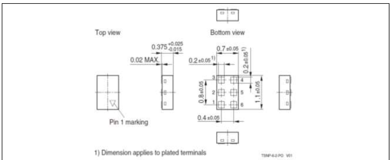
Figure 2 Package and pin connections of BGA7L1N6
