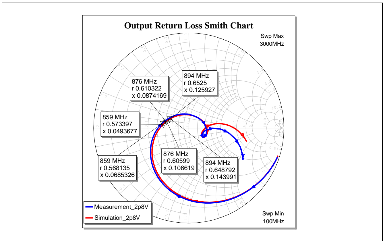
Figure 17 Output Matching (Smith Chart) of the BGA7L1N6 for LTE Band-26 Application at Vcc = 2.8 V
