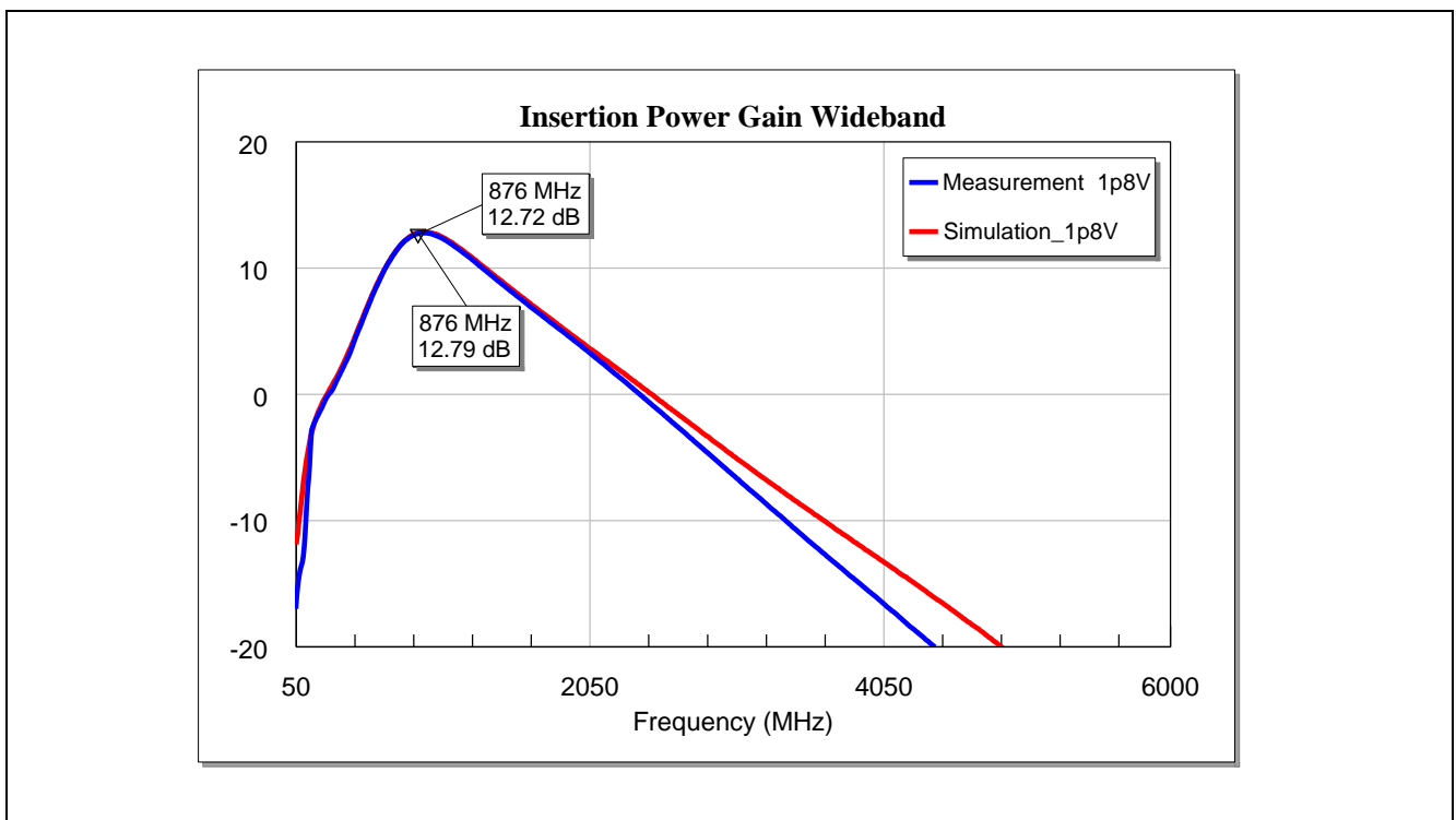
Figure 5 Insertion Power Gain (Wideband) of the BGA7L1N6 for LTE Band-26 at Vcc = 1.8 V
