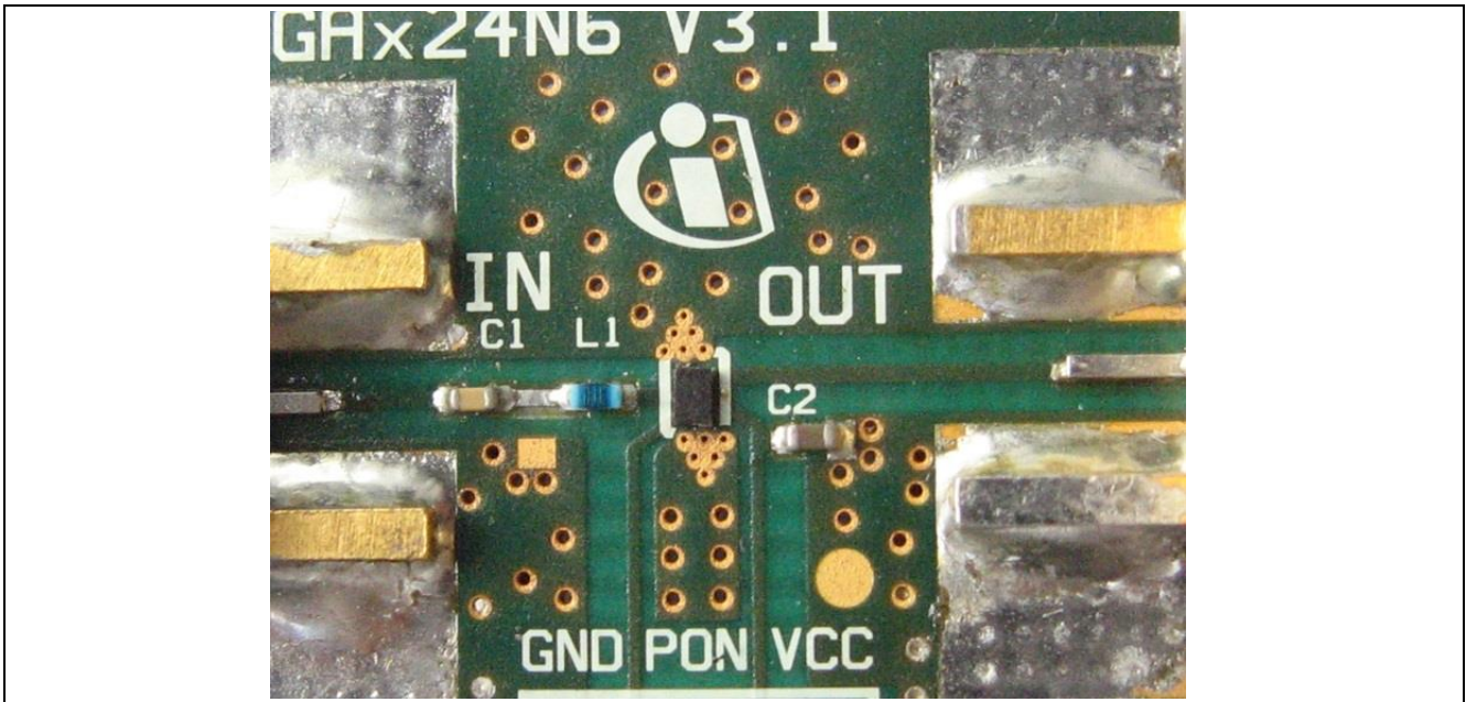
Figure 23 Photo Picture of Evaluation Board (overview)
