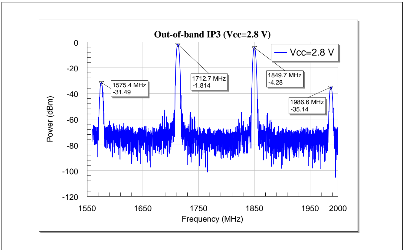
Figure 20 Out-of-band IP3 of the BGA524N6 as LNA for GNSS applications (2.8V)
