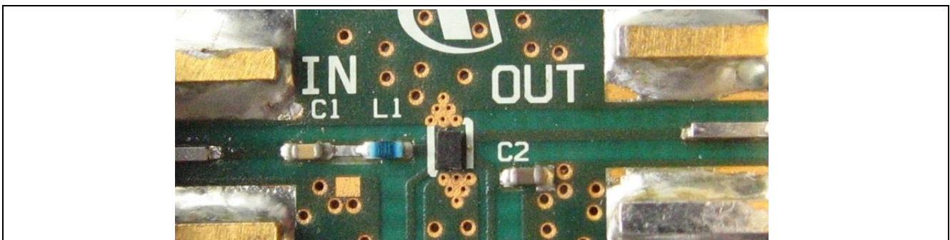
Figure 24 Photo Picture of Evaluation Board (detailed view)
