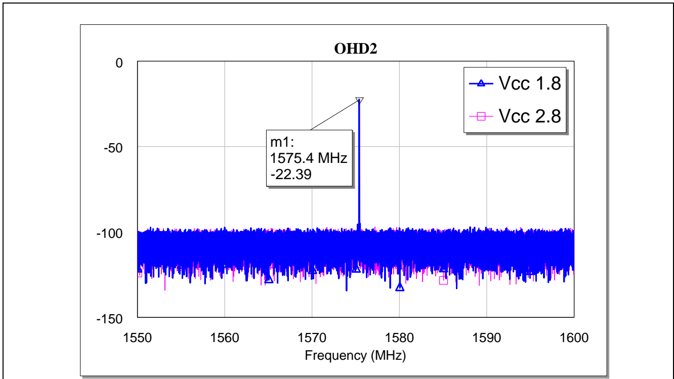
Figure 21 LTE Band 13 Second Harmonic Interference of the BGA524N6 as LNA for GNSS applications (LNA output referred)
