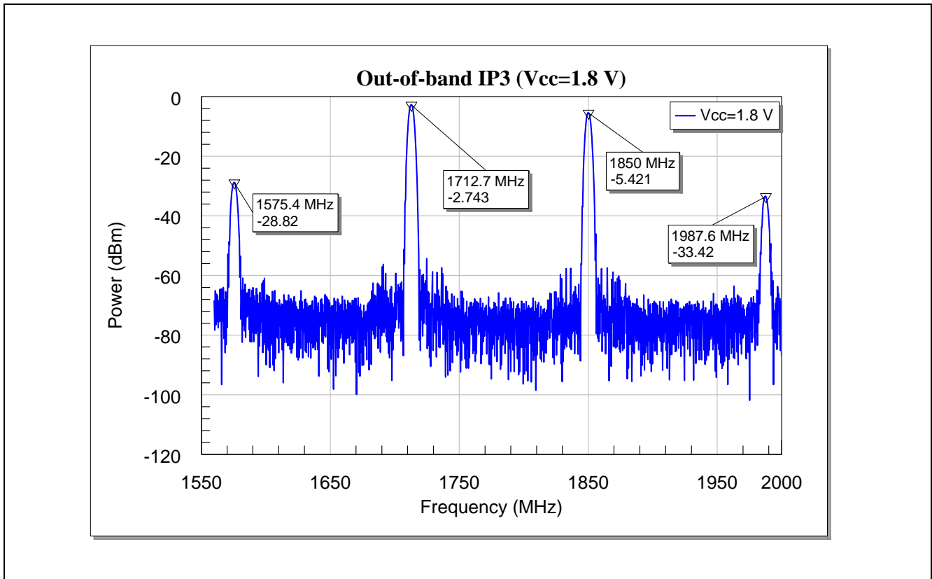
Figure 19 Out-of-band IP3 of the BGA524N6 as LNA for GNSS applications (1.8V)
