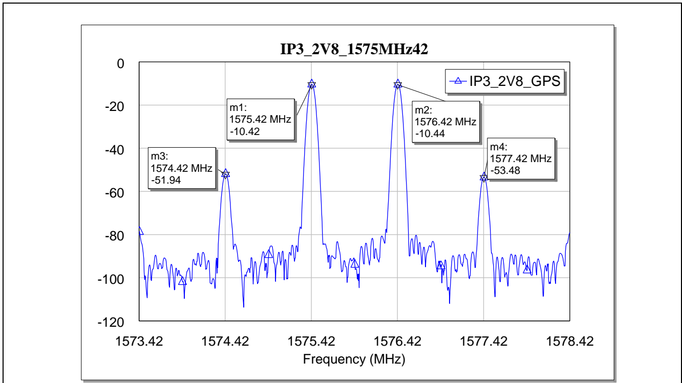
Figure 18 Output IP3 of the BGA524N6 as LNA for GNSS applications (2.8V)
