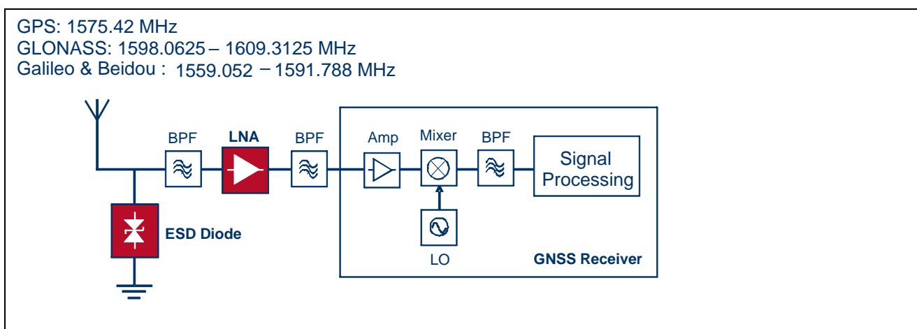
Figure 1 Application Diagram: Receiver Frontend the Global Navigation Satellite System With LNAs and Filter
