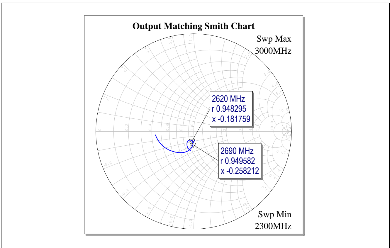
Figure 9 Output Matching (Smith Chart) of the BFQ790 for Band-7 Applications
