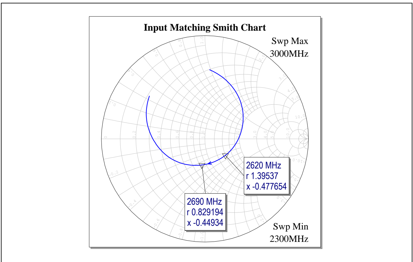
Figure 7 Input Matching (Smith Chart) of the BFQ790 for Band-7 Applications
