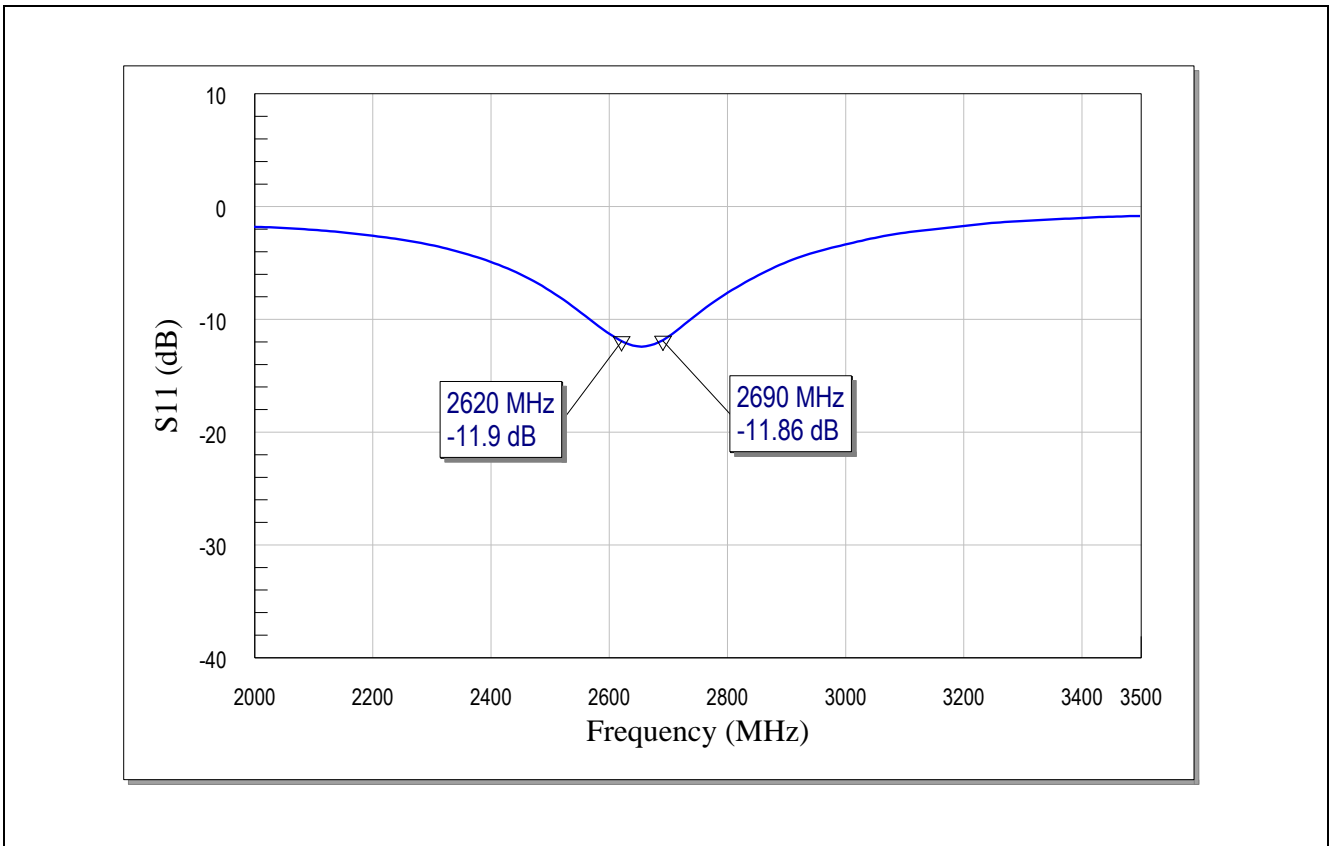
Figure 6 Input Matching of the BFQ790 for Band-7 Applications
