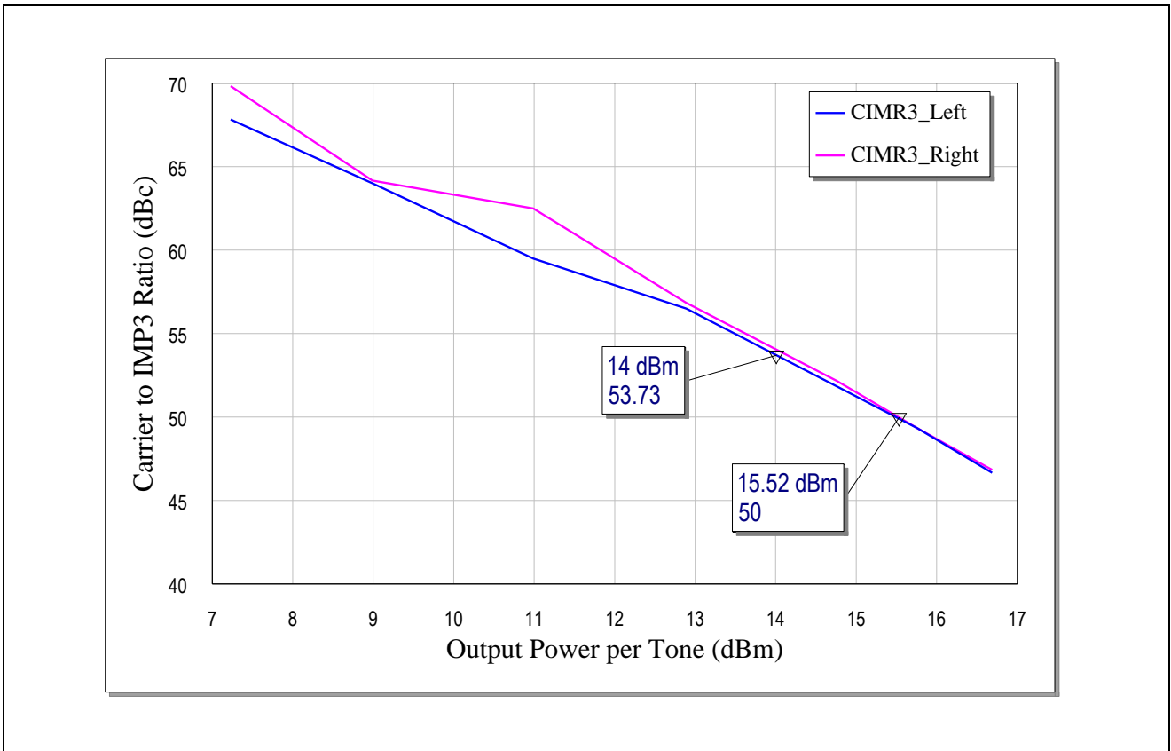
Figure 12 Carrier to IM3 Ratio of the BFQ790 for Band-7 Applications
