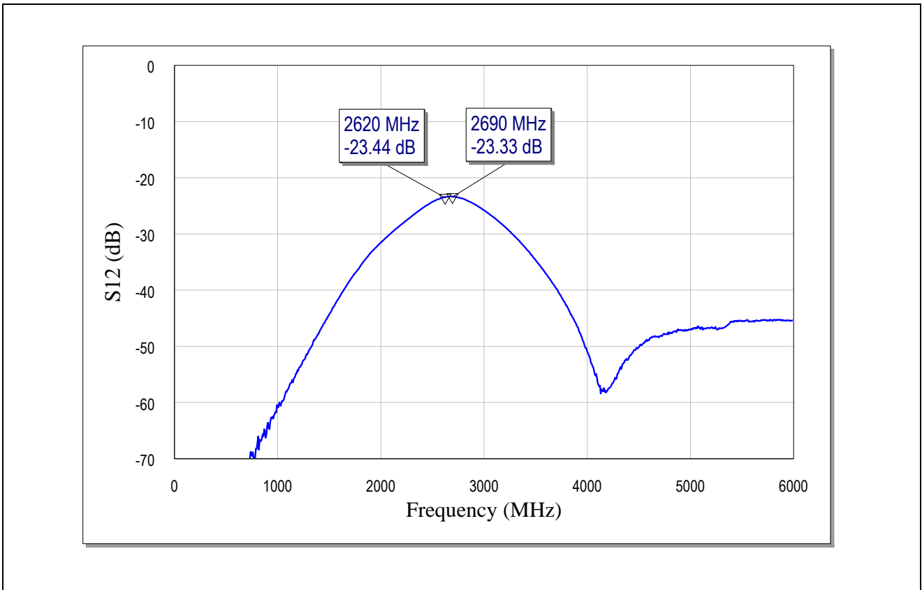
Figure 10 Reverse Isolation of the BFQ790 for Band-7 Applications
