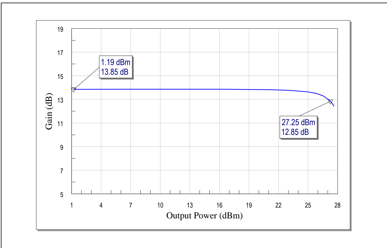
Figure 11 Output 1dB Compression Point of the BFQ790 for Band-7 Applications
