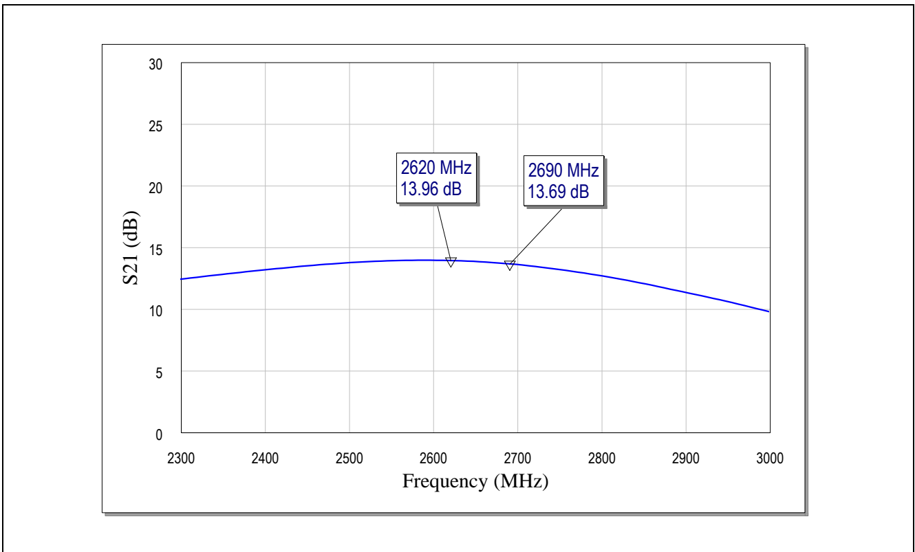
Figure 5 Narrowband Insertion Power Gain of the BFQ790 for Band-7 Applications
