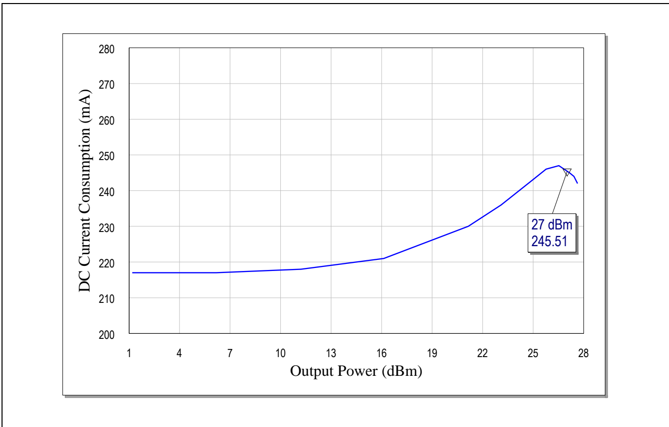
Figure 13 DC Current Consumption versus Output Power of the BFQ790 for Band-7 Applications
