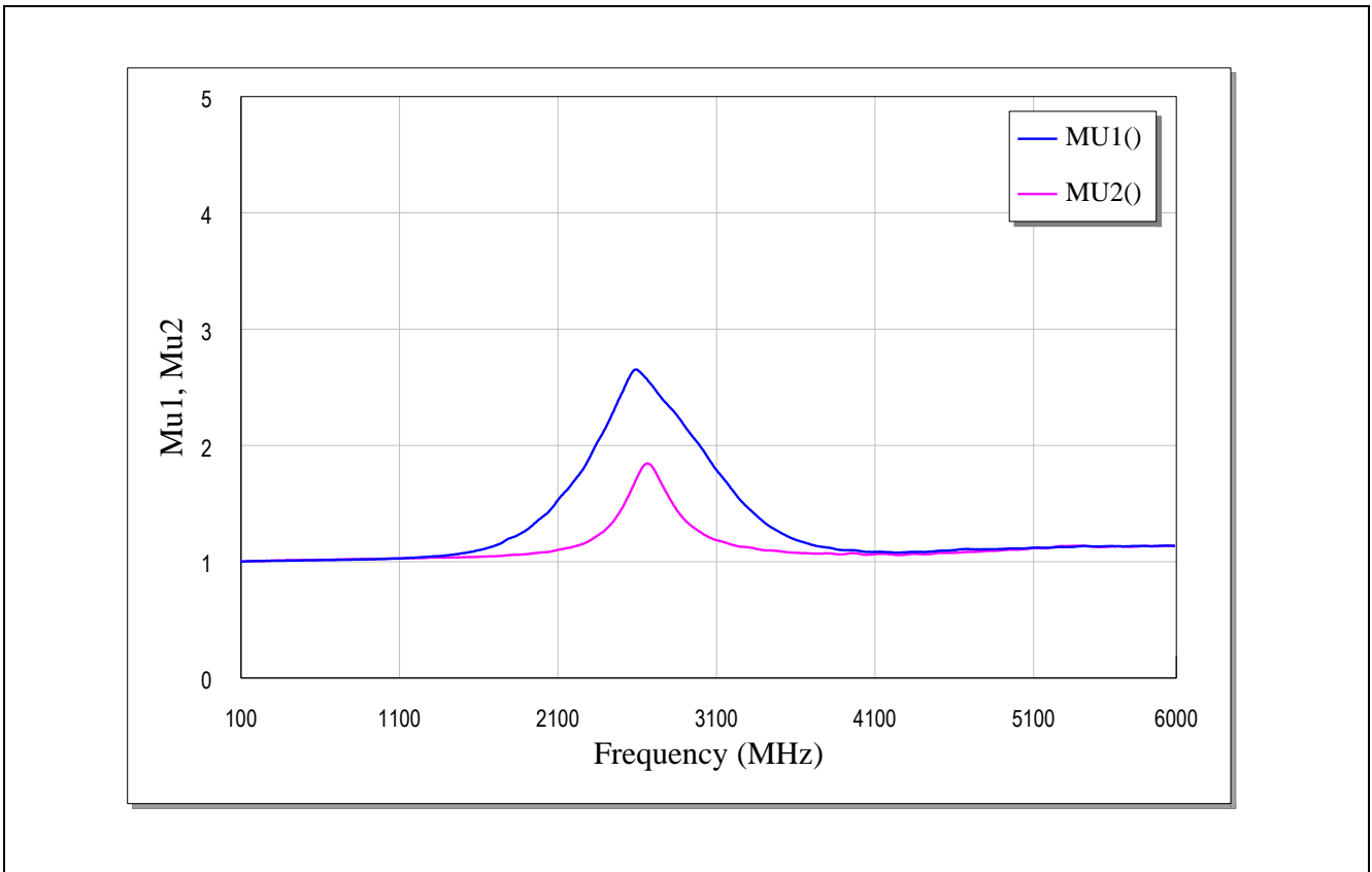
Figure 14 Stability Mu1, Mu2-factors of the BFQ790 for Band-7 Applications
