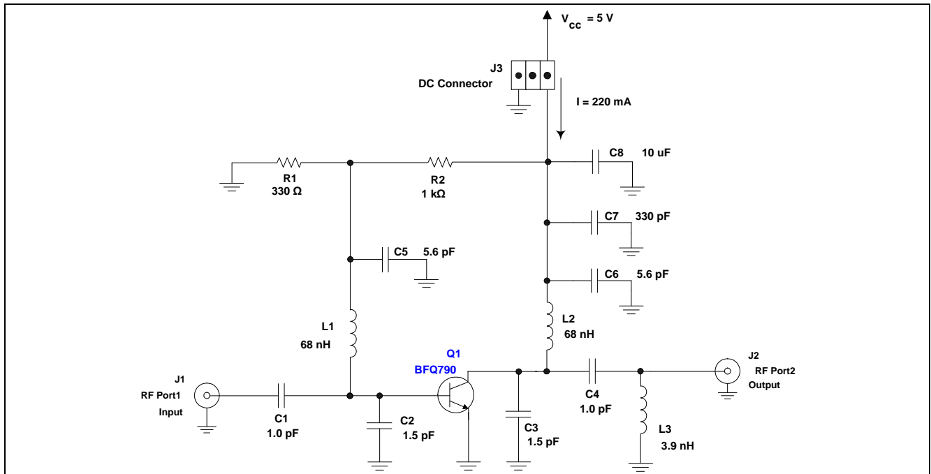
Figure 3 Schematics of the BFQ790 Application Circuit for LTE Band-7 (2620 - 2690 MHz)
