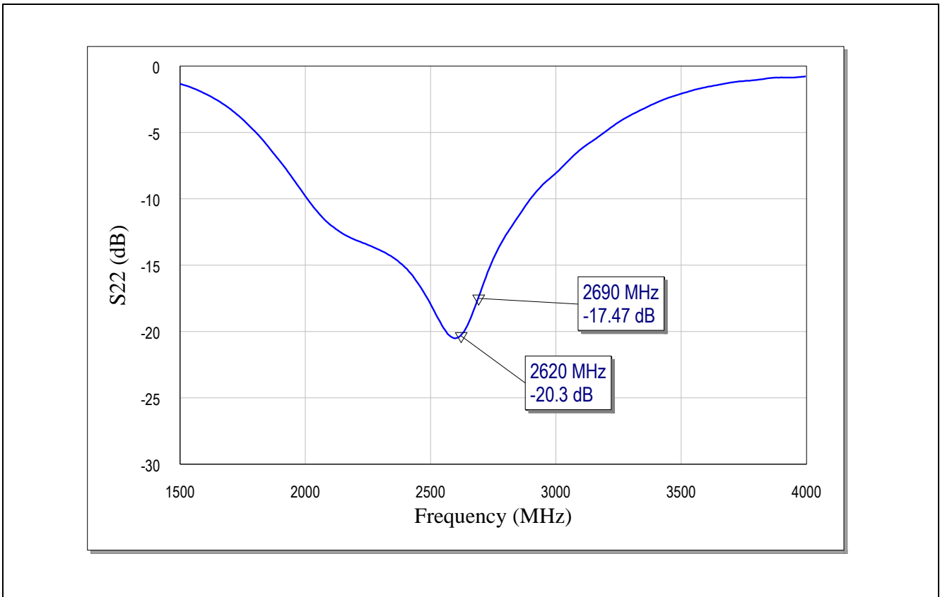
Figure 8 Output Matching of the BFQ790 for Band-7 Applications
