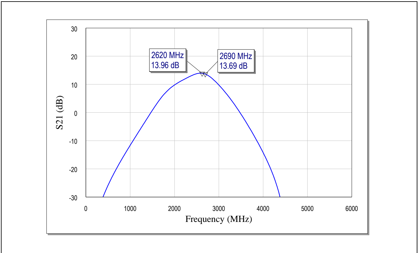
Figure 4 Wideband Insertion Power Gain of the BFQ790 for Band-7 Applications
