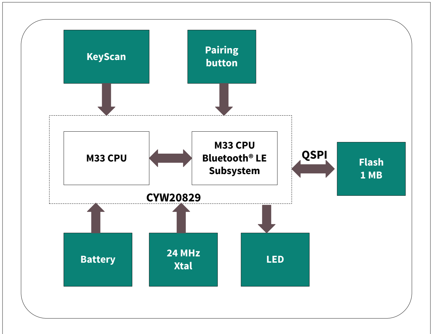
Figure 1 Keyboard application block diagram
