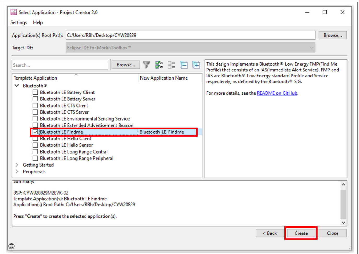
Figure 10 Import Bluetooth® LE Find Me code example
