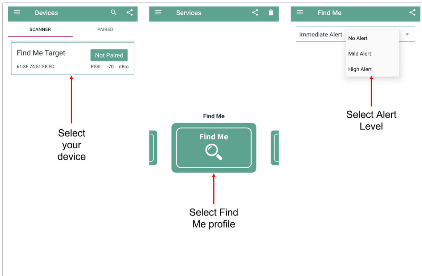
Figure 33 Testing with the AIROC™ Bluetooth® Connect app on Android
