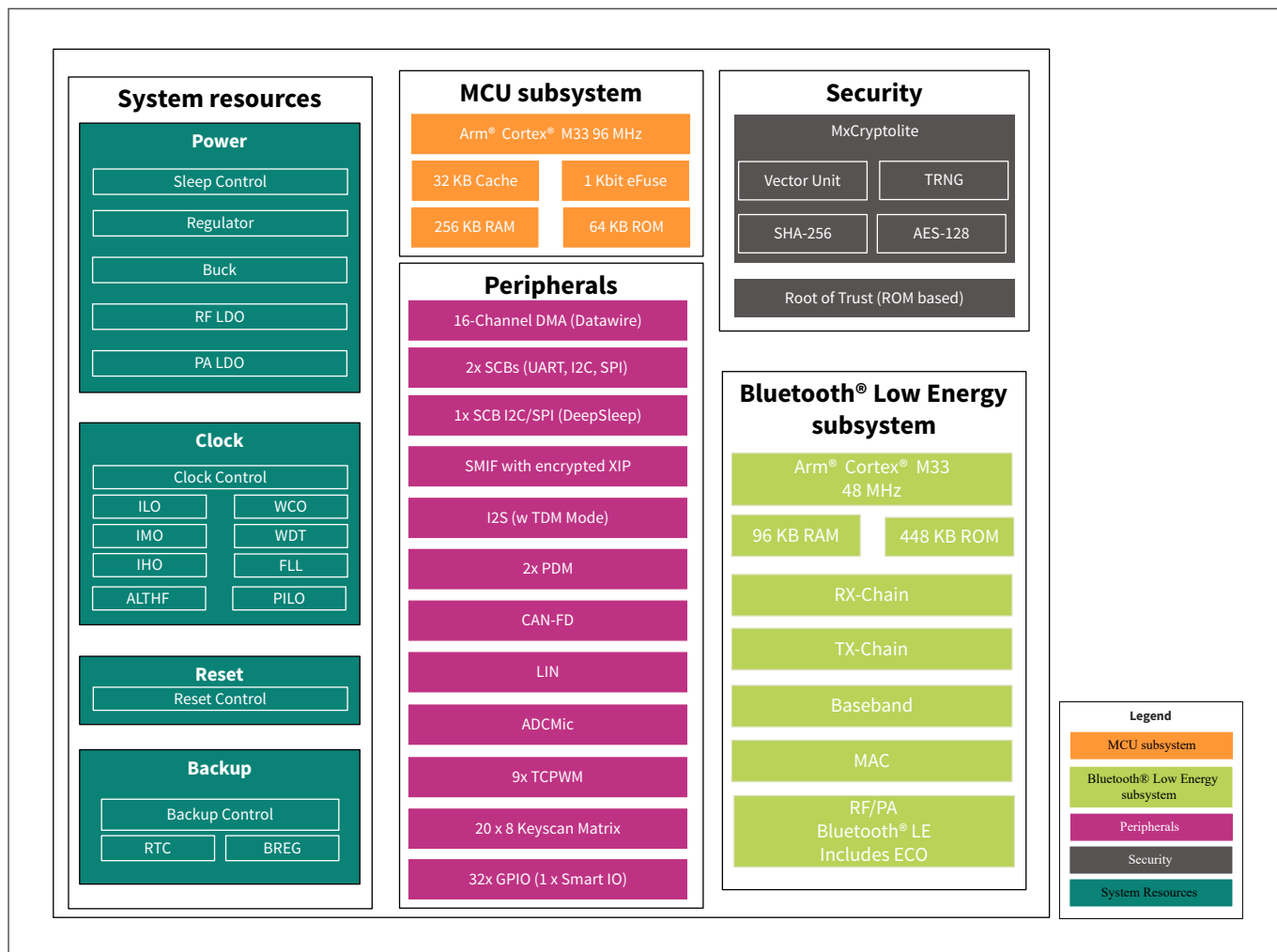
Figure 4 CYW20829 MCU with Bluetooth® LE connectivity block diagram
