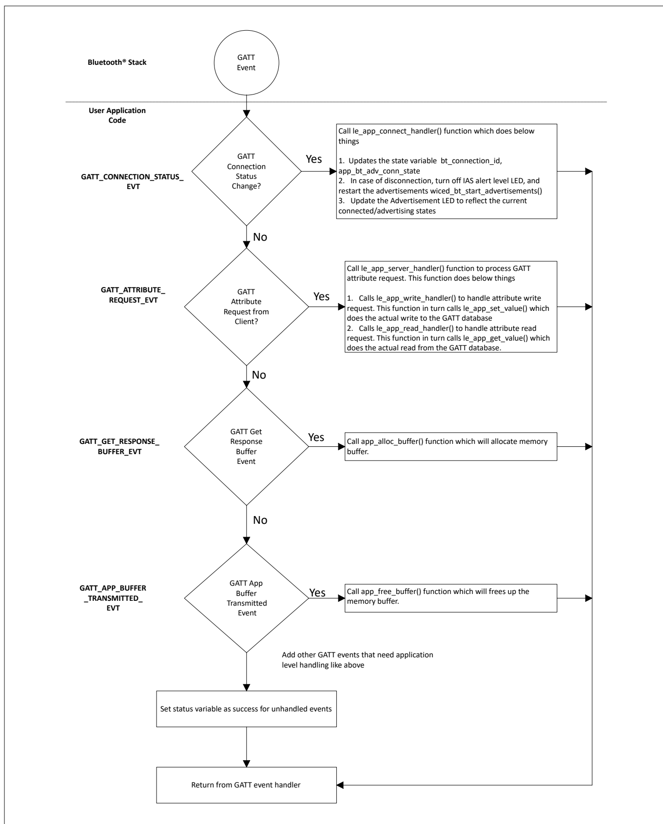
Figure 29 GATT event handler
