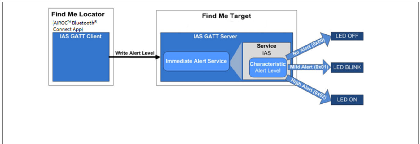
Figure 6 Find Me Profile (FMP) application using CYW20829 MCU
