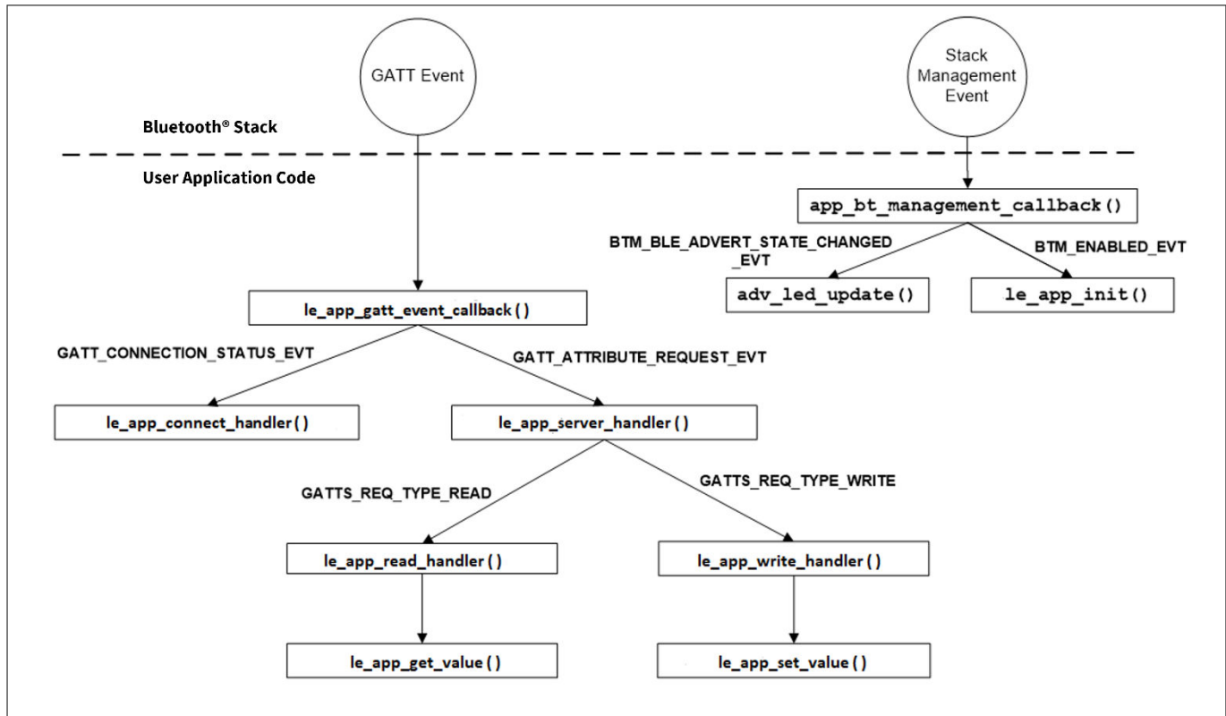
Figure 30 Bluetooth® stack events function call chart
