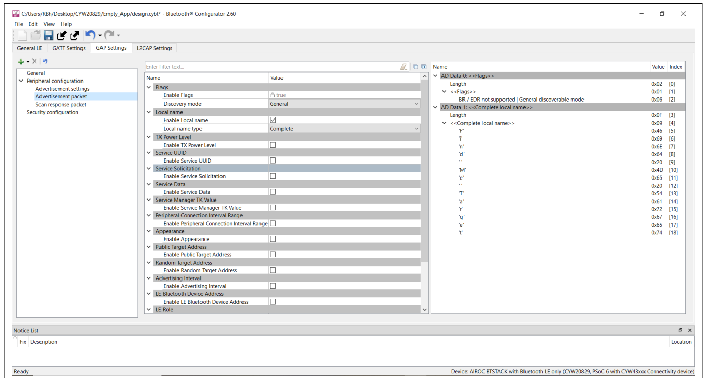
Figure 26 GAP advertisement packet settings
