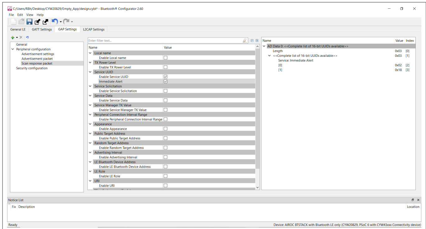
Figure 27 GAP scan response packet settings
