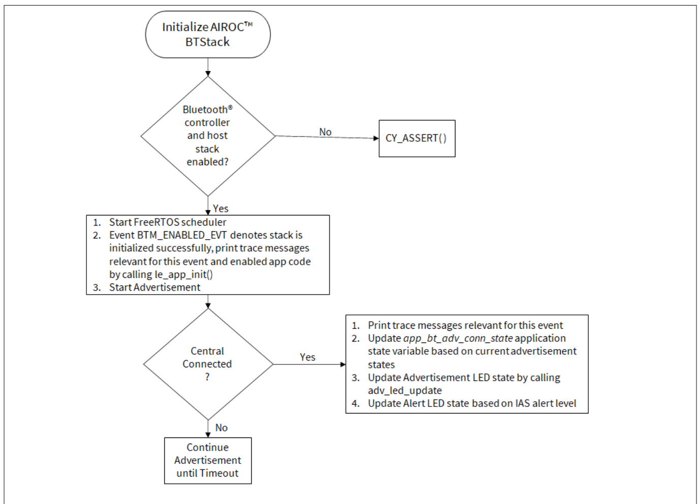
Figure 28 Bluetooth® stack management event handler function flow
