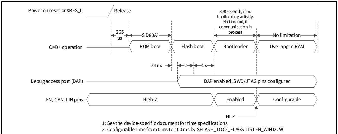
Figure 4 Startup timing
