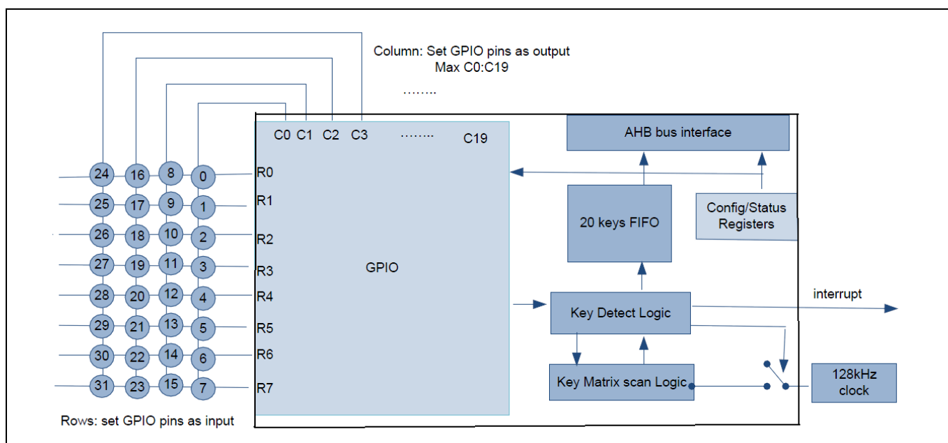
Figure 4 Keyboard scanner for CYW20819/CYW20820
