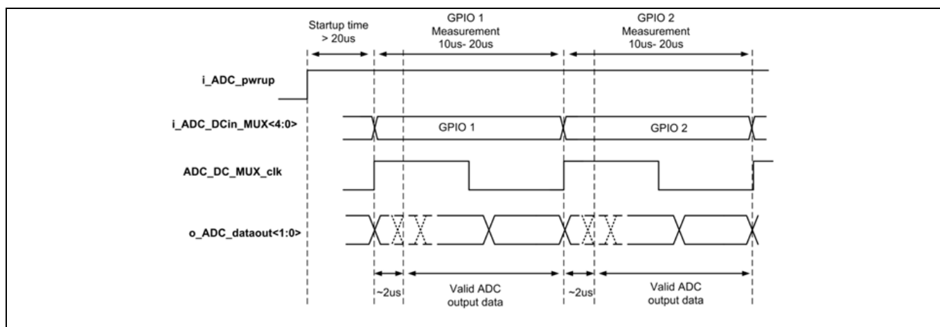
Figure 2 Mux clocking and timing diagram of ADC
