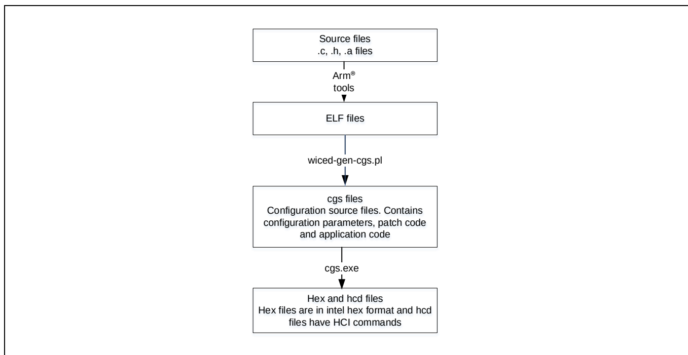
Figure 7 File formats
