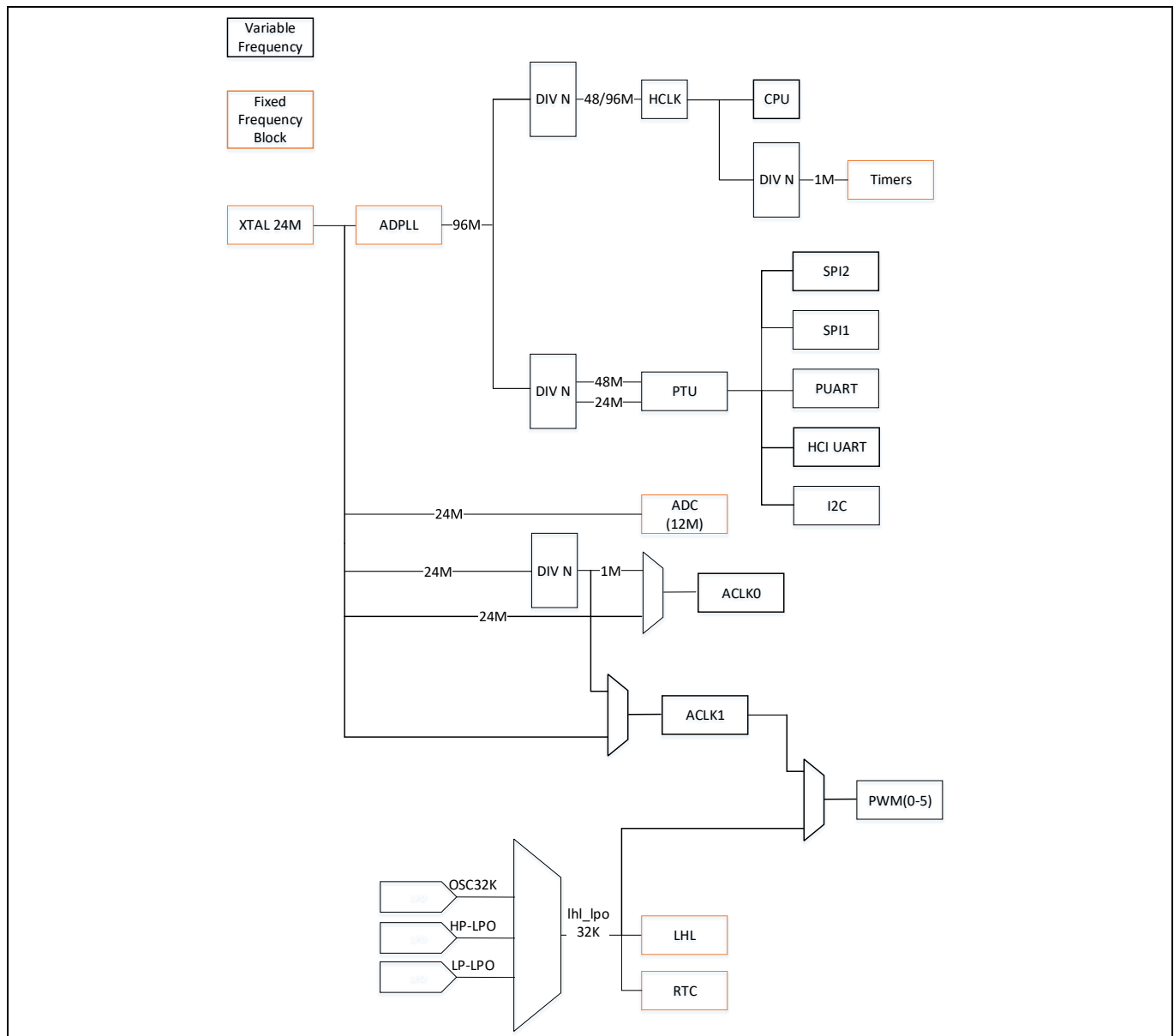
Figure 3 Clock diagram of CYW20819/CYW20820
