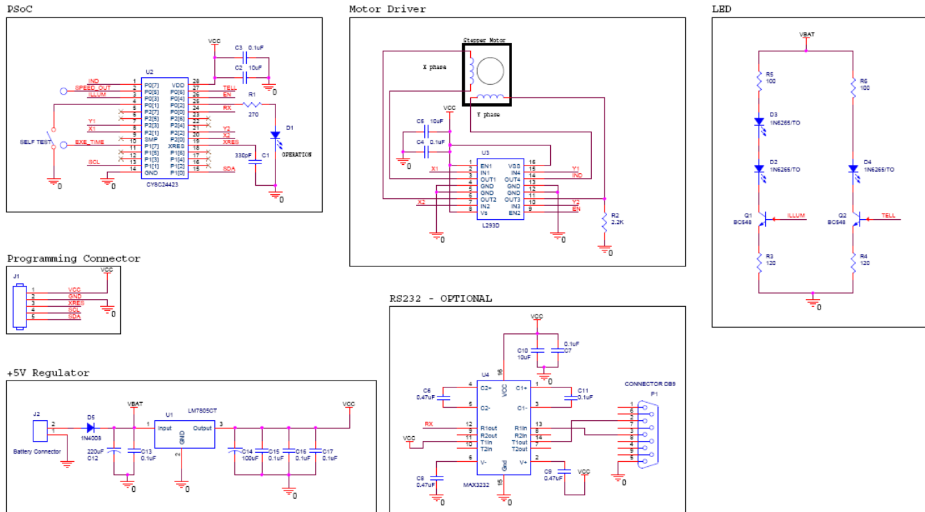
Figure 10. Driver Schematic
