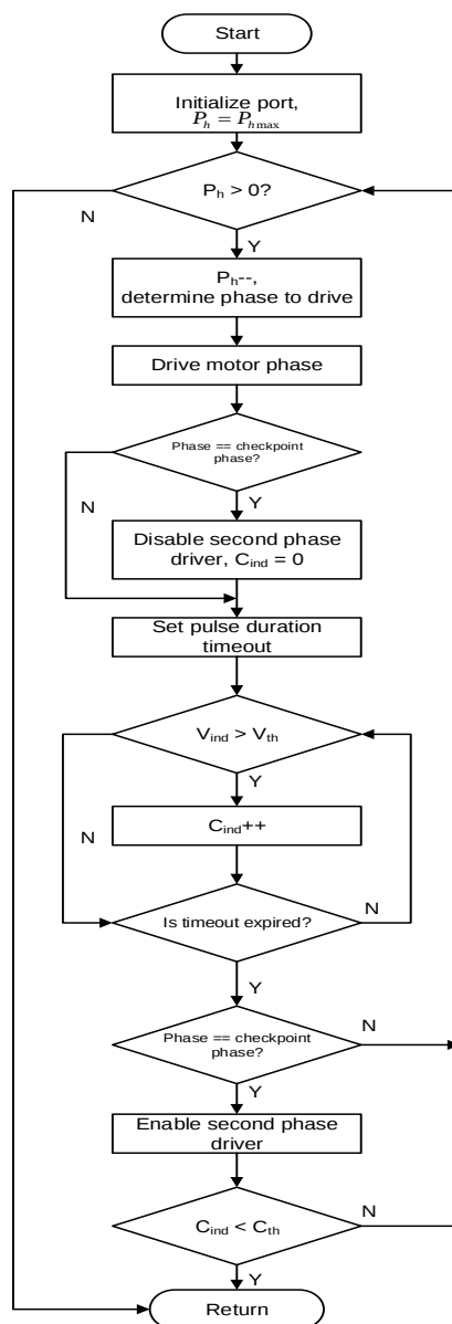
Figure 7. Pointer Synchronization Mechanism
