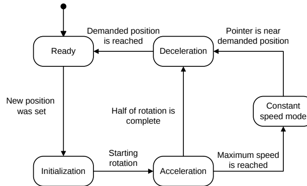
Figure 3. Speed Control Module State
