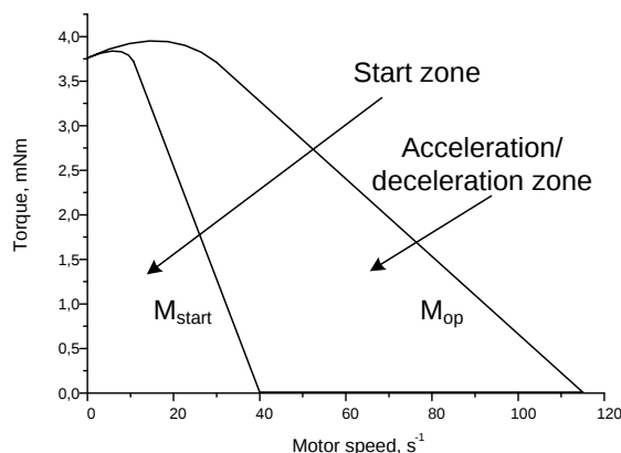
Figure 1. Stepper Motor Torque vs. Motor Speed
