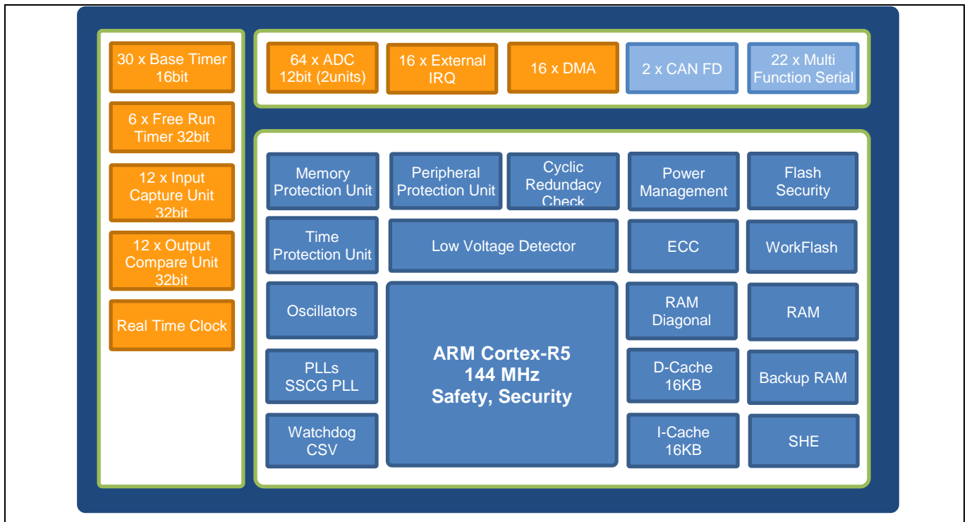
Figure 1 Traveo™ Family S6J3110 series block diagram
