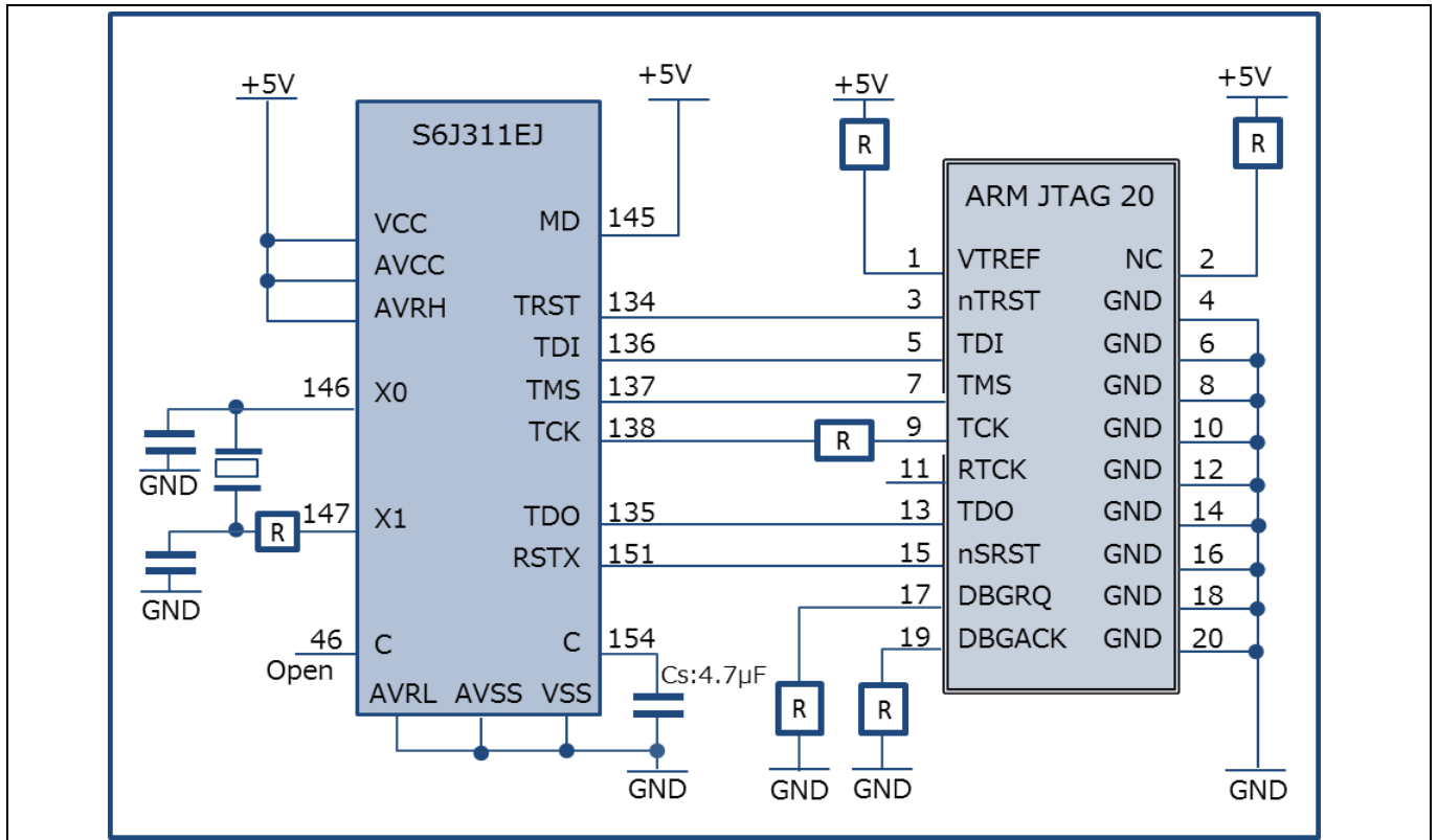
Figure 2 S6J311EJ basic connection diagram with Arm JTAG 20
