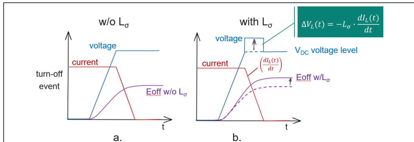
Figure 26 a. A simplified example of an ideal turn-off event without the influence of L_\sigma b. A simplified example of a turn-off event with the influence of L_\sigma
