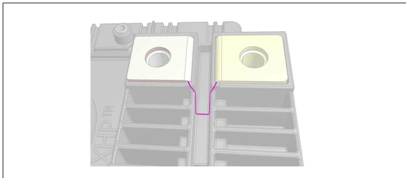
Figure 8 XHP™ 2 creepage distances between power terminal 1; 2 and power terminal 6; 7
