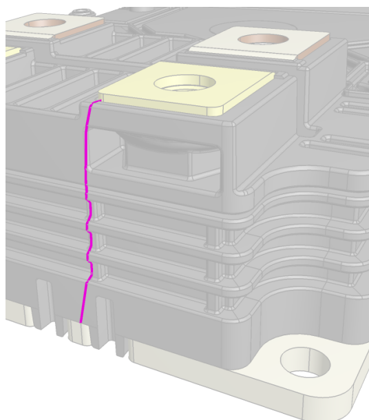
Figure 10 Creepage distance between power terminal 1; 2 and base plate in an XHP™ 2 module
