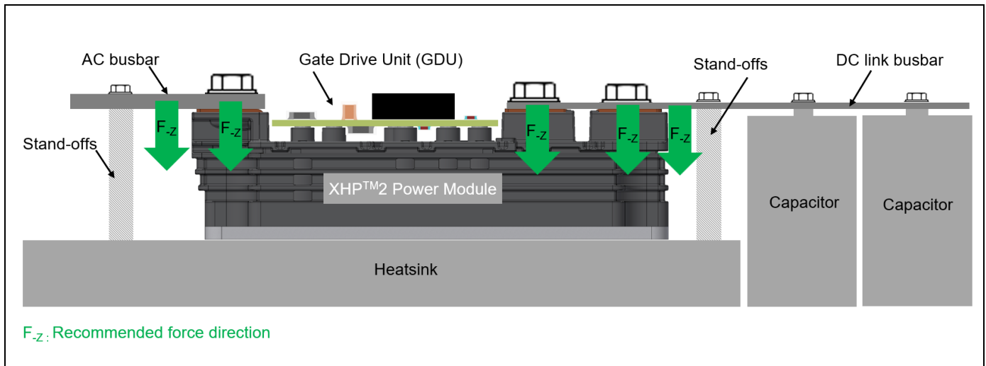
Figure 22 Simplified representation of a configuration with a proposed strain-relief method
