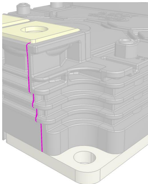
Figure 11 Creepage distance between power terminal 3; 5 and base plate in an XHP™ 2 module
