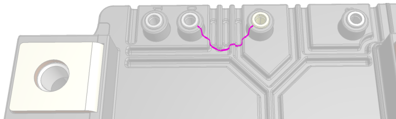
Figure 14 Creepage distance between Aux terminal 9 and Aux terminal 10 in an XHP™ 2 module
