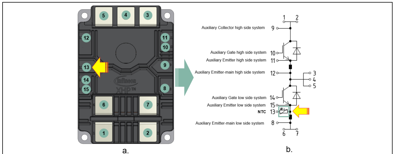
Figure 32 a. Typical module auxiliary connector positions b. Simplified GDU auxiliary connection with dedicated thermistor position
