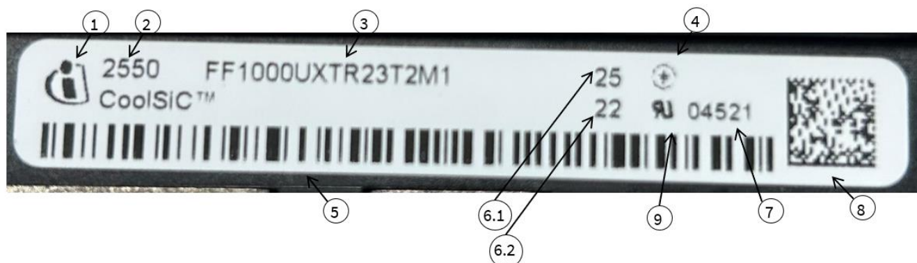
Figure 5 Exemplary XHP™ 2 product label for CoolSiC™ modules
