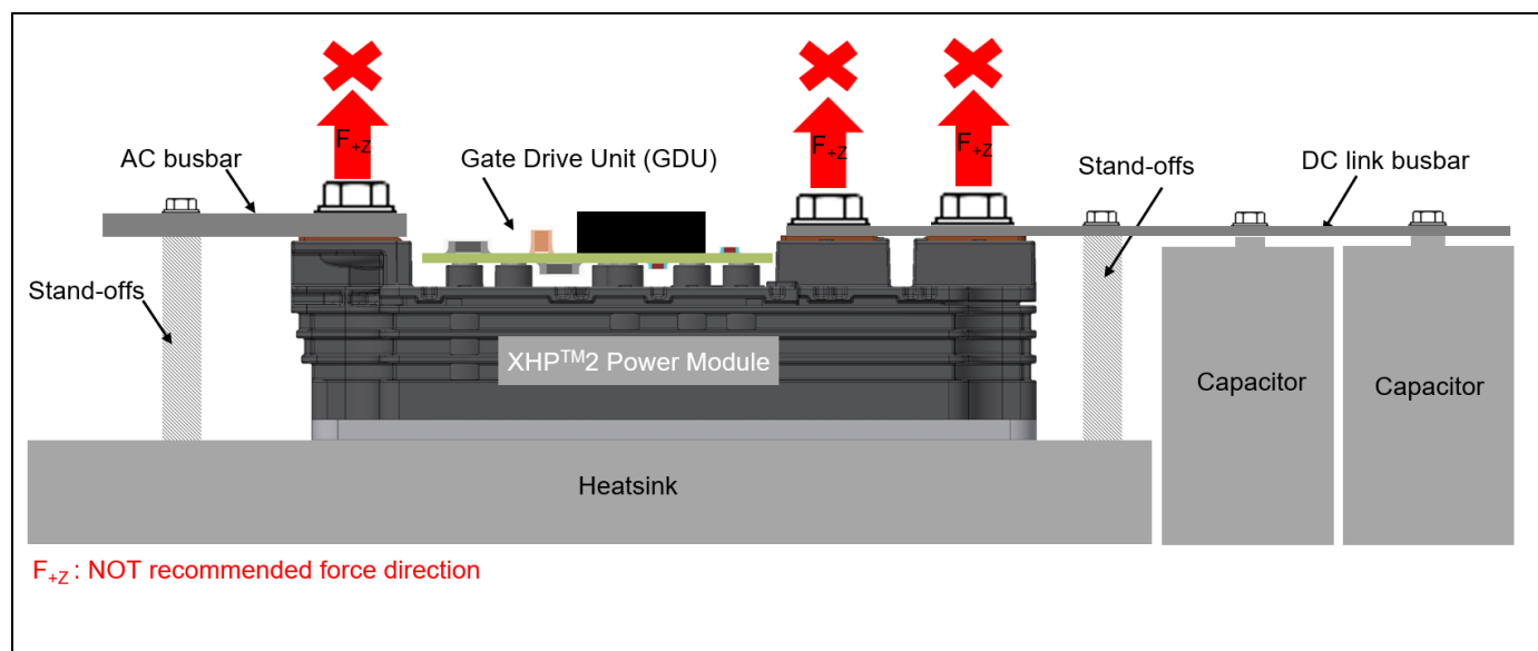
Figure 23 Simplified representation of a configuration that is NOT recommended
