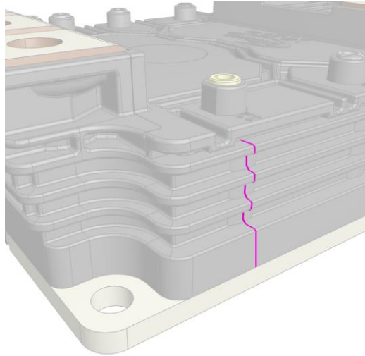
Figure 13 Creepage distance between Aux terminal 12 and the module base plate in an XHP™ 2 module
