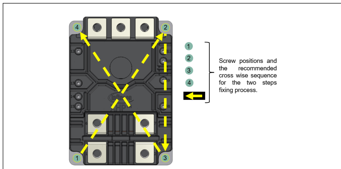
Figure 18 Exemplary crosswise tightening sequence for the XHP™ 2 modules
