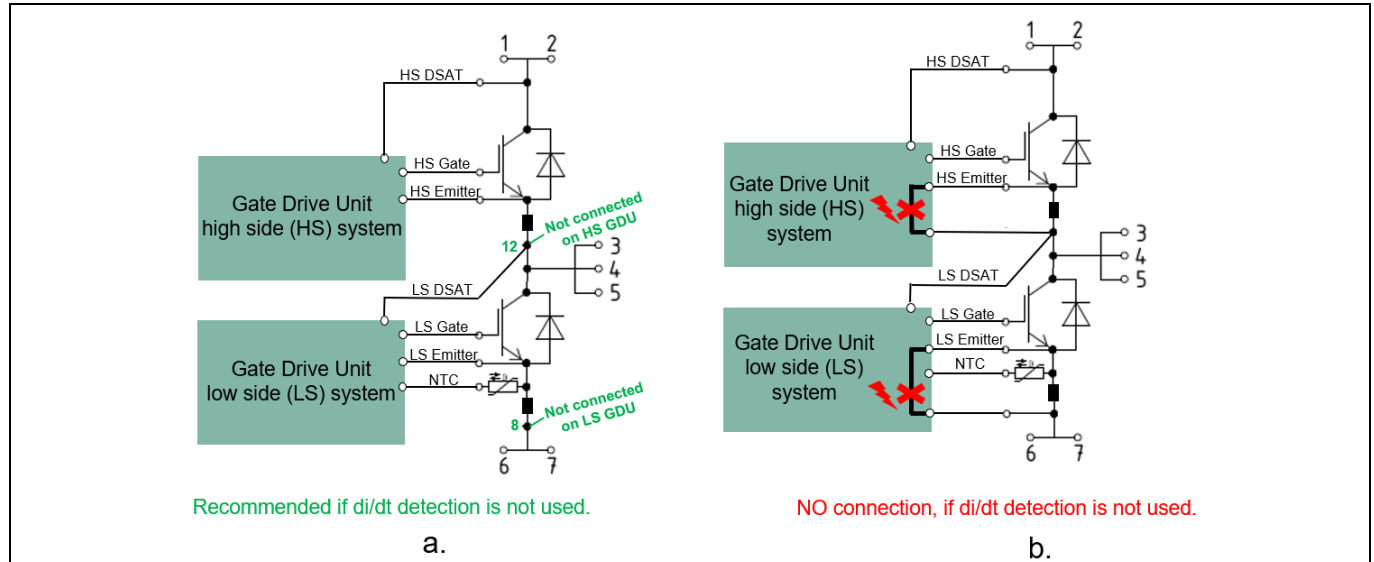
Figure 31 Simplified GDU auxiliary connection assignment and recommendation if di/dt detection is not used
