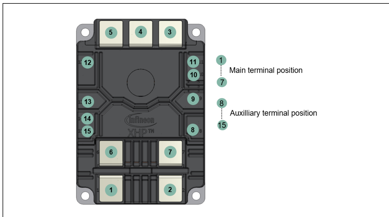
Figure 7 XHP™ 2 module terminal position
