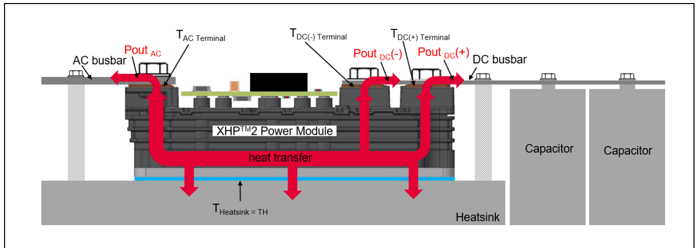
Figure 19 Simplified heat transfer to the XHP™ 2 power terminal during operation
