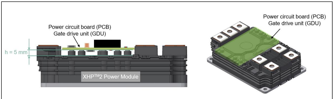
Figure 28 Simplified representation of the XHP2 module for the gate drive unit (GDU)
