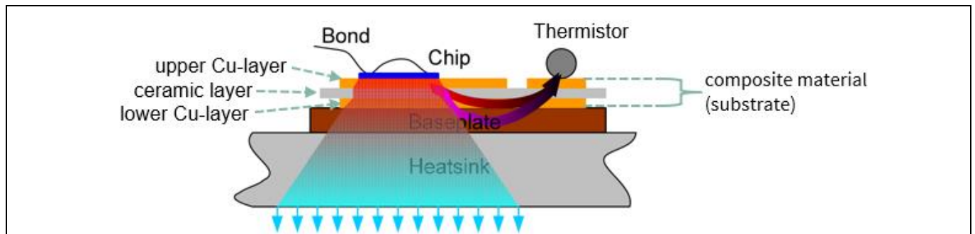
Figure 33 Flow of thermal energy inside a power electronic module
