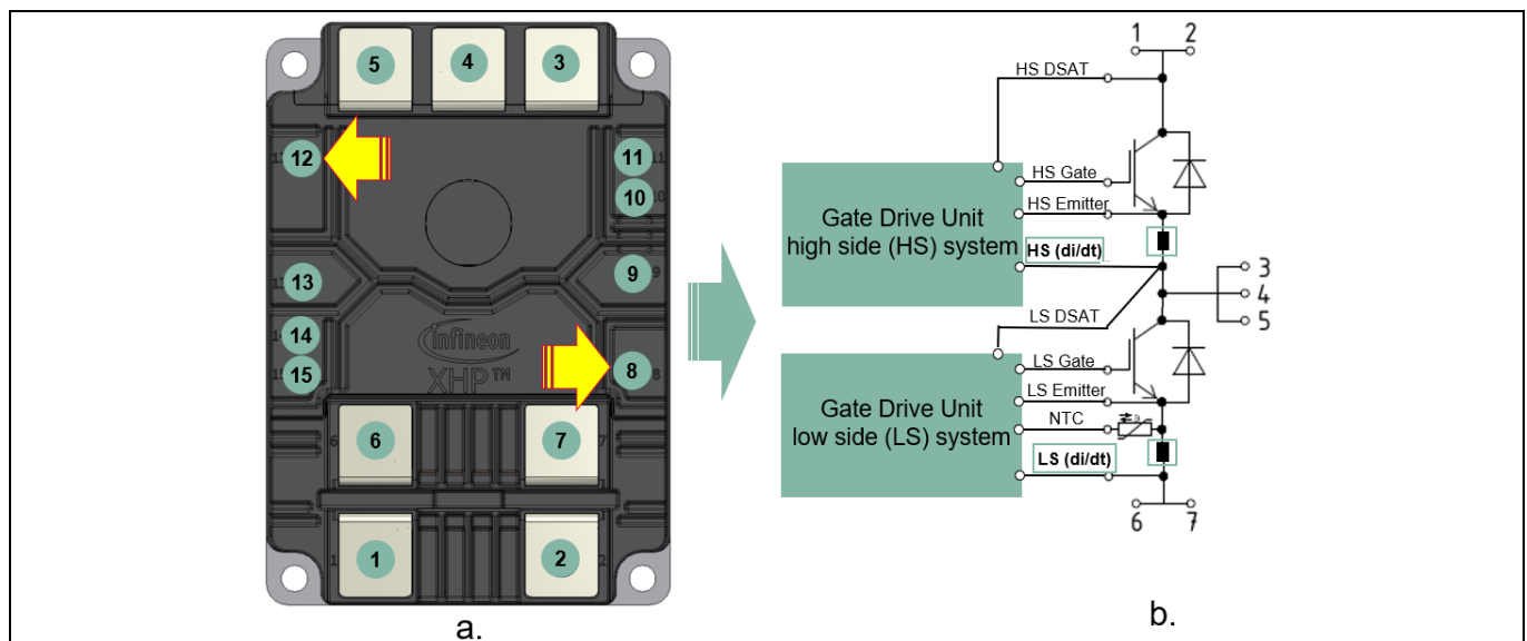
Figure 30 a. Typical module auxiliary connector positions b. Simplified GDU auxiliary connection with a dedicated (di/dt) detection connection for advanced gate driver design
