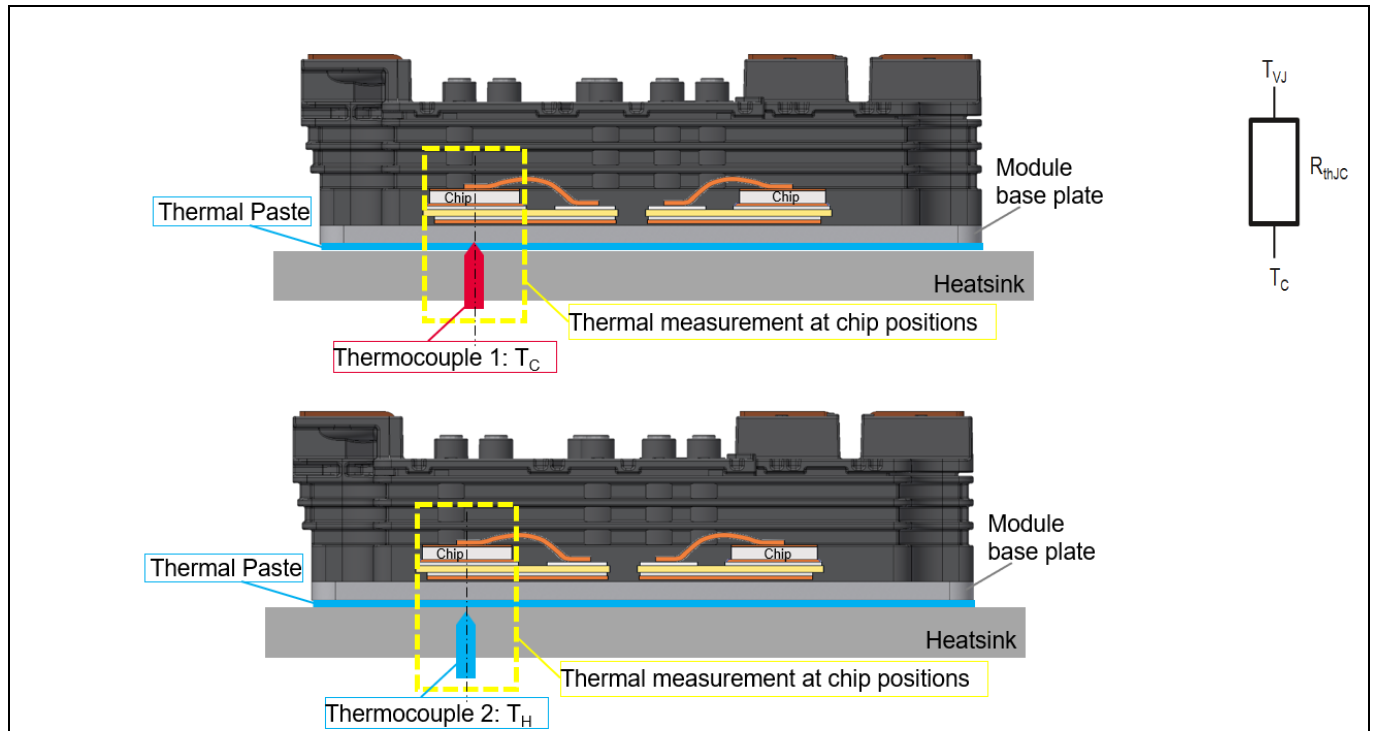
Figure 34 A simplified example of a temperature measurement setup using:
