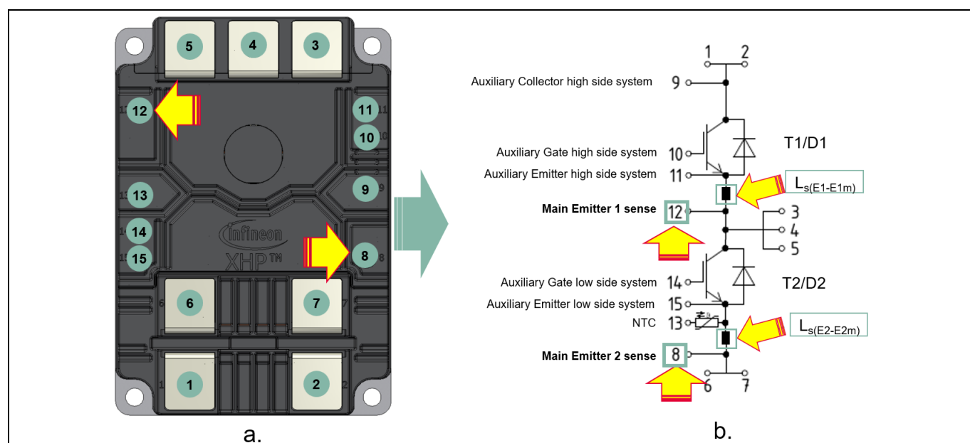
Figure 29 a. Typical auxiliary connector positions b. Typically auxiliary connection assignment with a main emitter sense equivalent circuit
