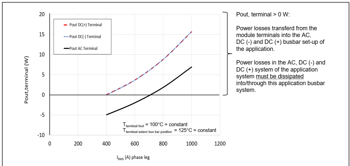
Figure 20 Simulation results of an XHP™ 2 power terminal losses under various current conditions
