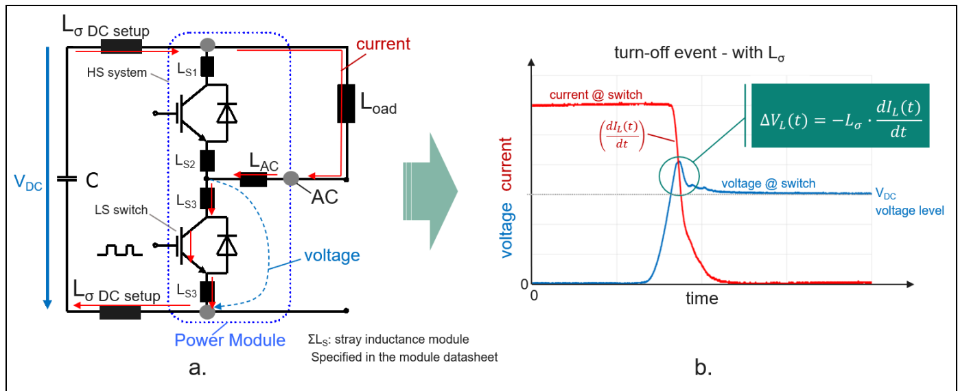
Figure 6 a. Simplified equivalent circuit diagram of a power module in a test setup b. Simplified example of a turn-off event with the overvoltage influences due to L_\sigma
