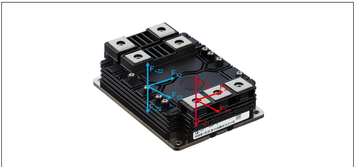
Figure 21 Direction of the maximum permissible force during the assembly process at the XHP™ 2 module terminals
