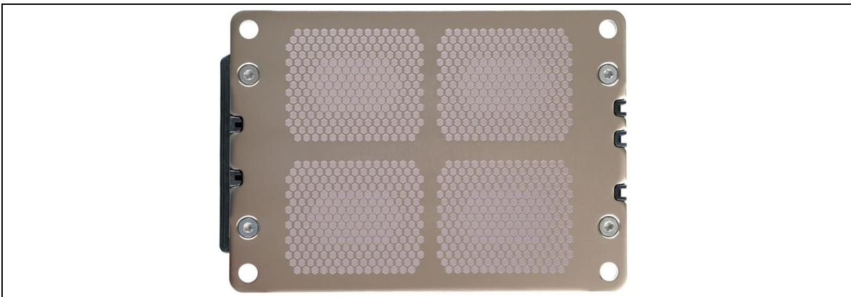
Figure 16 Exemplary XHP™ 2 power module with Infineon's pre-applied thermal interface material
