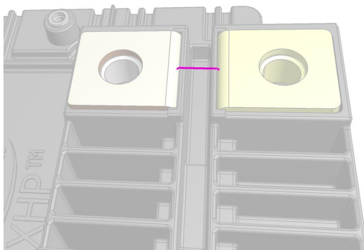
Figure 9 Clearance distance between power terminal 1; 2 and power terminal 6; 7 in an XHP™ 2 module
