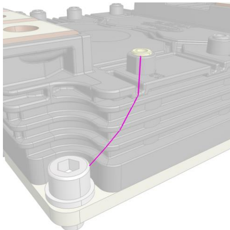
Figure 15 Clearance distance between a PCB and screw
