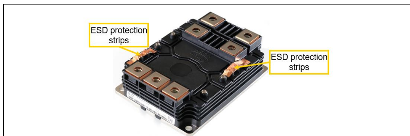
Figure 27 XHP™ 2 package ESD protection strips
