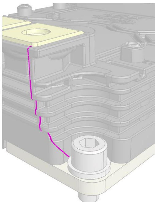
Figure 12 Creepage distance between power terminal 3; 5 and module mounting screw in an XHP™ 2 module
