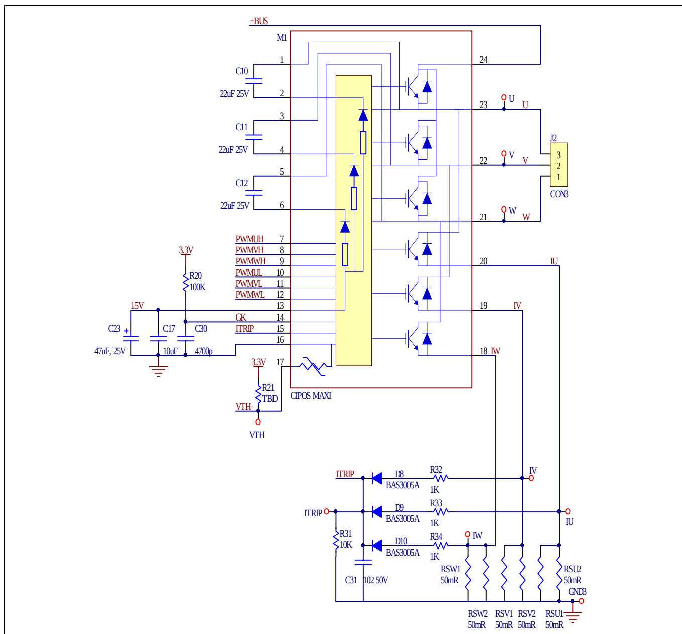
Figure 22 Schematic of the 3-phase inverter section using CIPOS™ Maxi IPM on EVAL-M1-IM818-A
