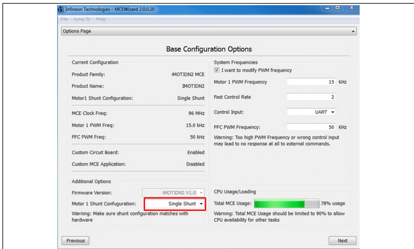
Figure 11 Shunt Configuration
