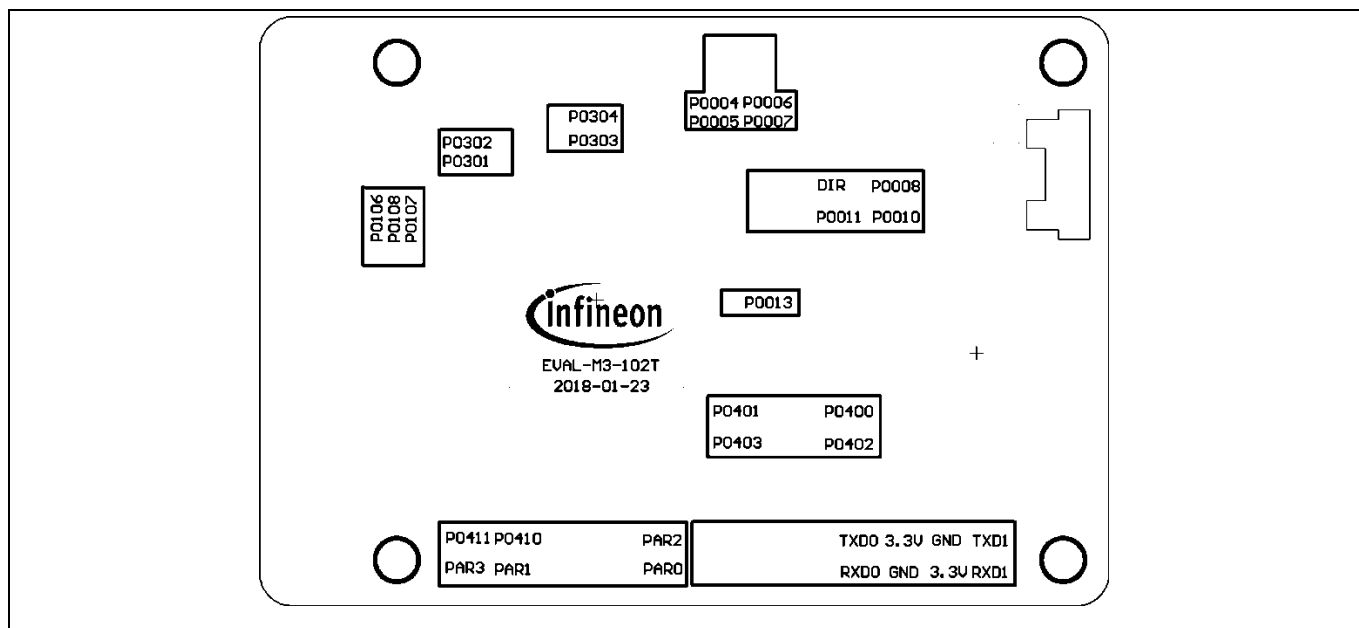
Figure 34 Bottom overlay print of the EVAL-M3-102T evaluation board
