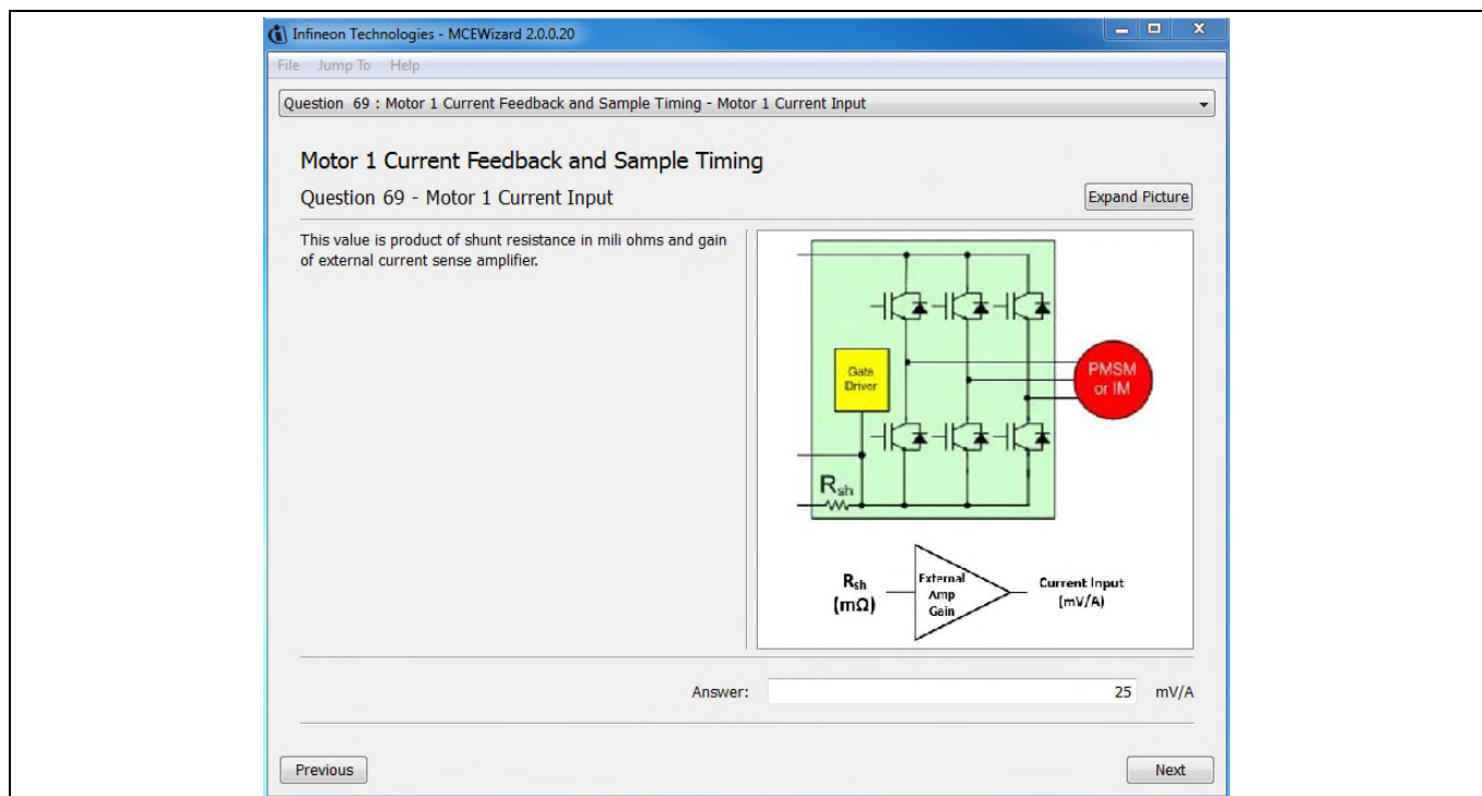
Figure 14 Current feedback configuration in MCEWizard for EVAL-M3-102T and EVAL-M3-CM615PN
