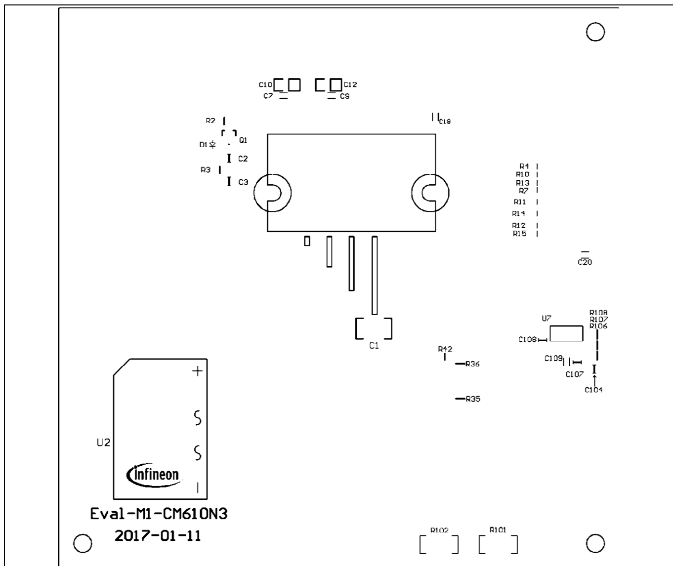
Figure 17 Bottom assembly print of the Eval-M1-CM610N3 evaluation board
