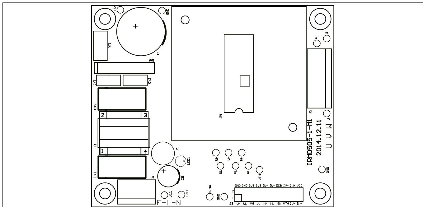
Figure 16 Top assembly print of the EVAL-M1-05-65D evaluation board
