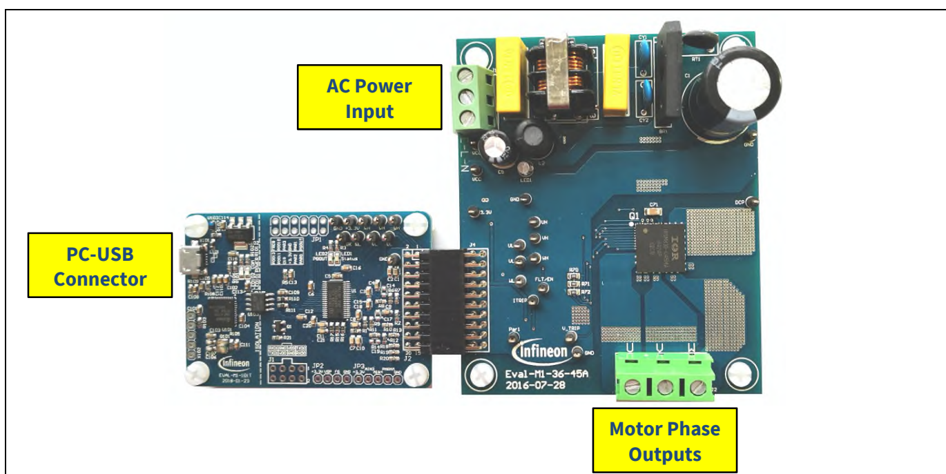
Figure 5 System connection example using EVAL-M1-101T and EVAL-M1-36-45A
