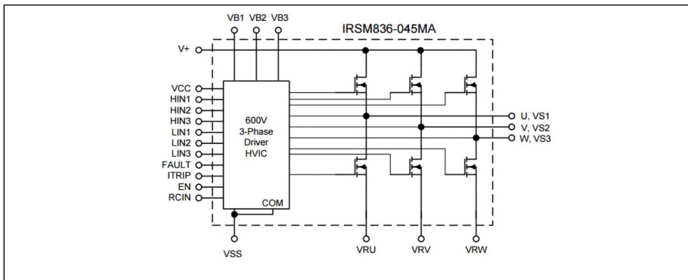
Figure 2 CIPOS™ Nano internal electrical schematic
