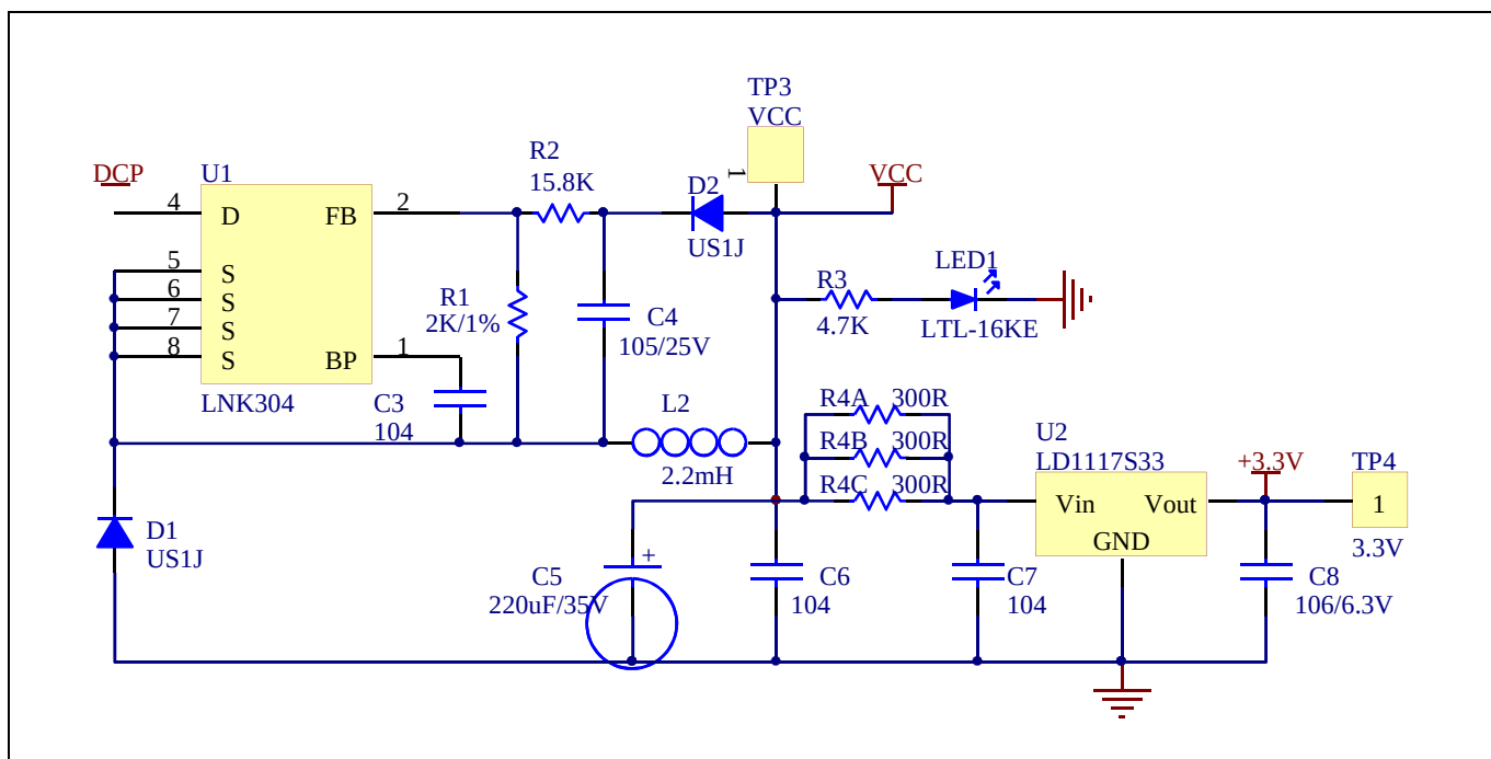
Figure 14 Power supply section of the EVAL-M1-36-45A evaluation board
