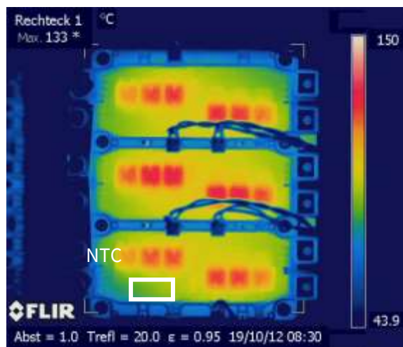
Figure 10: IR-picture of a module under load. DUT: FS450R17OE4P
