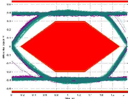
Figure 6. Edge Rate Change Due to 2 pF Capacitance
