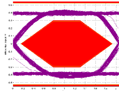
Figure 7. Signal near the USB Limits for Series Impedance
