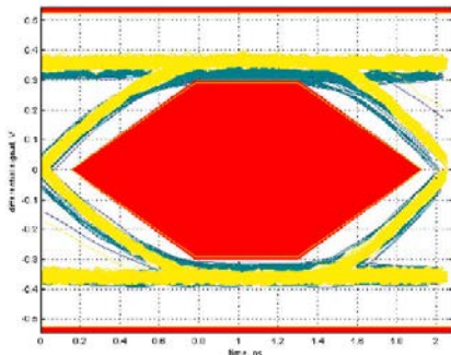
Figure 10. Differences from Probe Calibration
