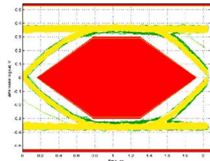
Figure 9. Extra Connector in the Test Path
