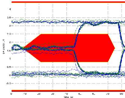
Figure 2. Measurement at Wrong End of Cable
