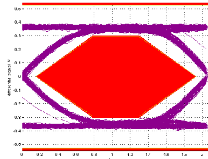
Figure 8. Standard 4-Inch Cable with Adaptor
