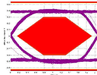
Figure 4. Proper Eye Measurement
