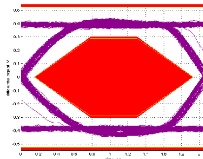
Figure 5. 2 pF Capacitance Added to Test Fixture
