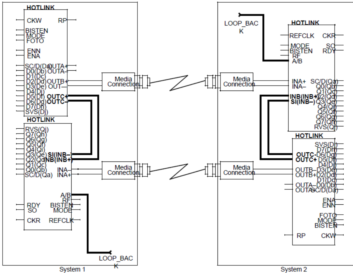
Figure 8. Example HOTLink Loop-Back System Connection
