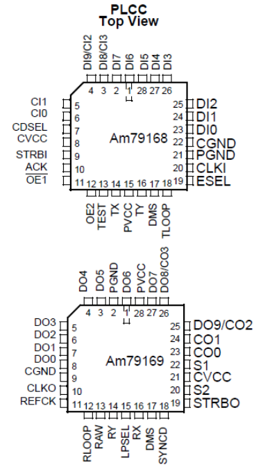
Figure 7. Am79168 and Am79169 Configurations
