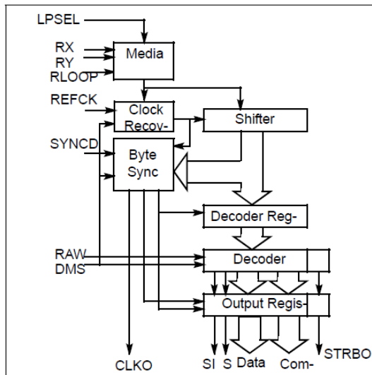
Figure 6. TAXI-275 Receiver Block Diagram
