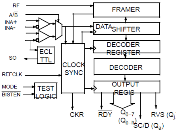
Figure 3. CY7B933 Receiver Logic Diagram
