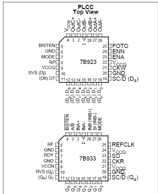
Figure 4. CY7B923 and CY7B933 Pin Configurations
