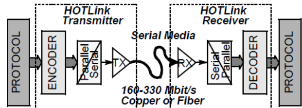
Figure 1. HOTLink System Diagram
