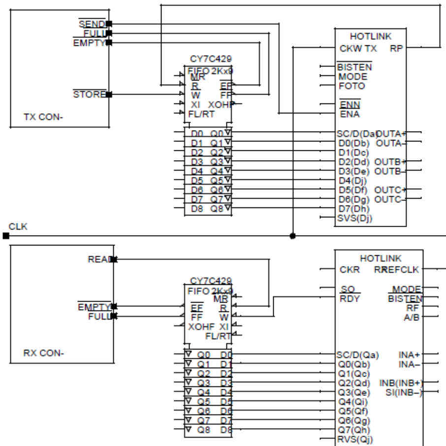
Figure 11. Asynchronous FIFO Interface (Note 1)
