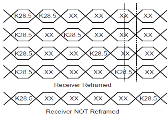
Figure 9. Double-Byte Reframing
