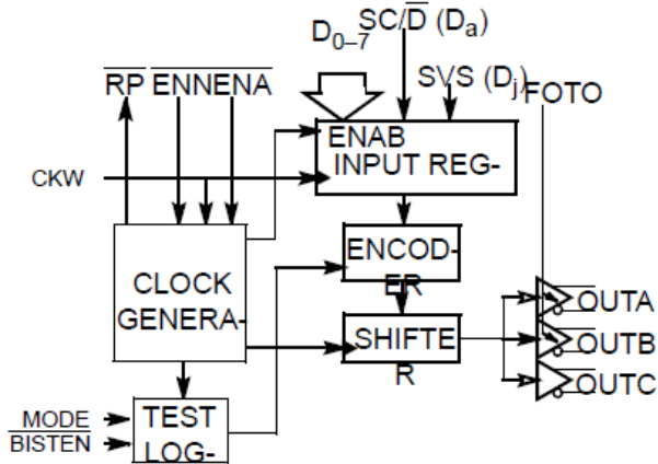
Figure 2. CY7B923 Transmitter Logic Diagram
