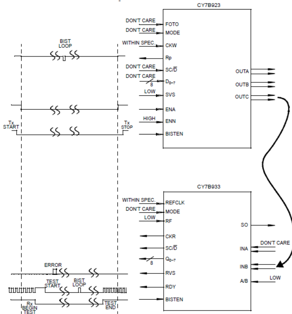
Figure 10. Built-In Self-Test
