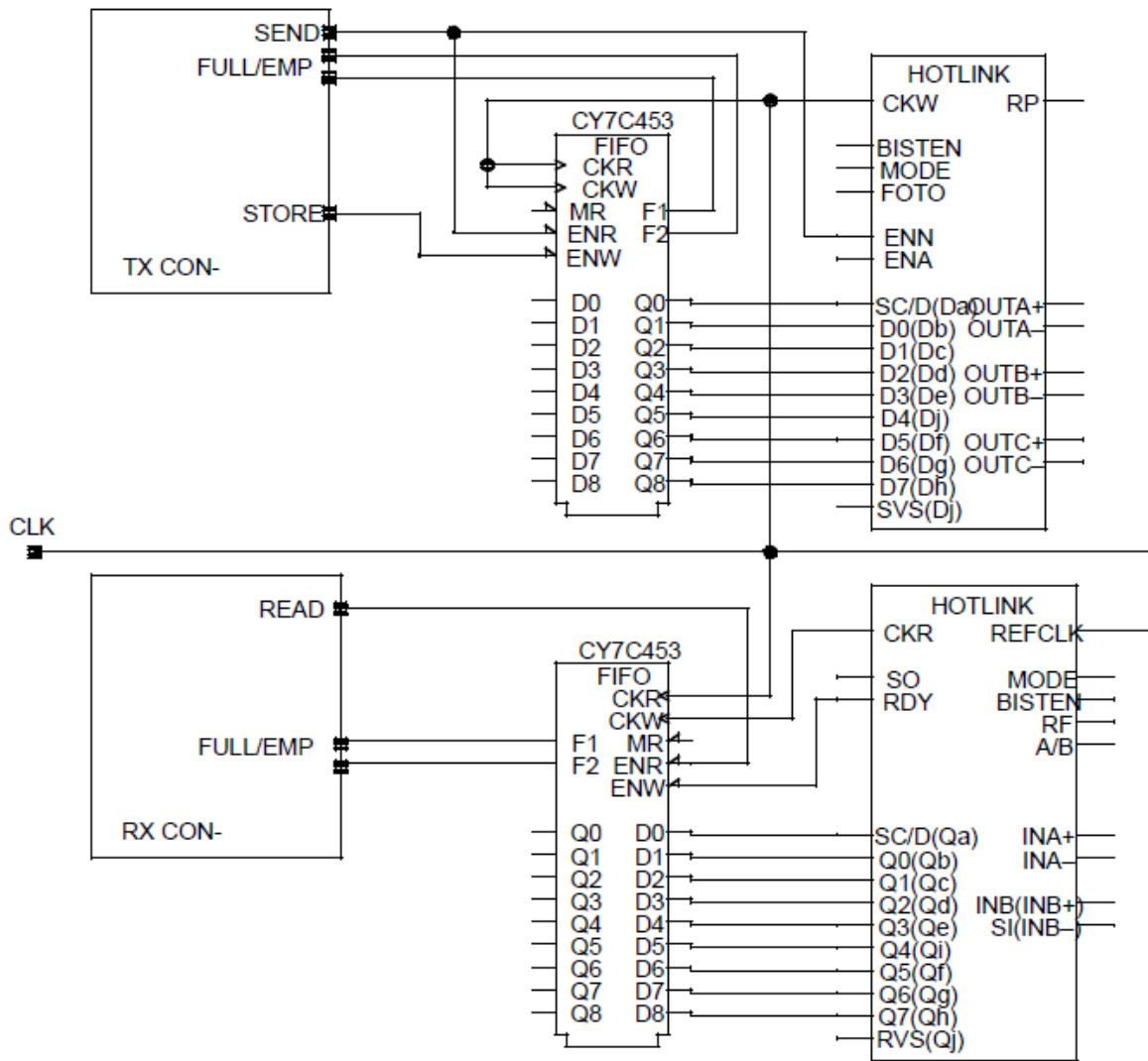
Figure 12. Clocked FIFO Interface (Note 2)
