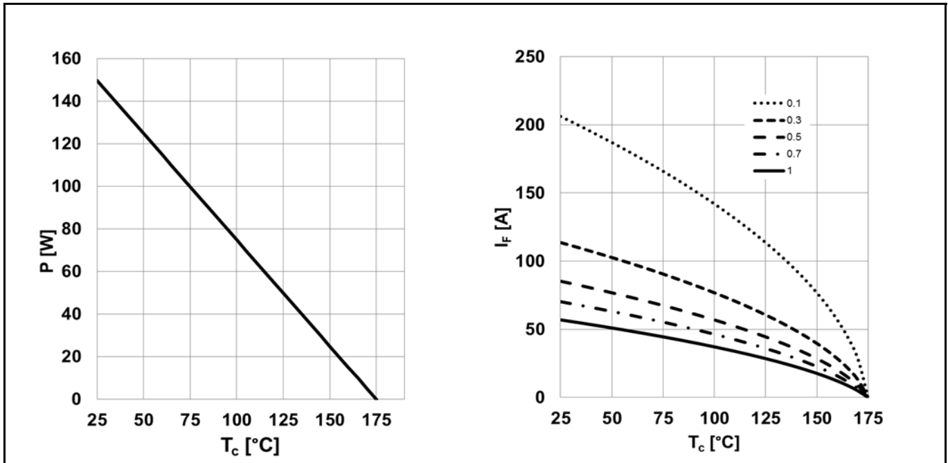
Figure 1 (LEFT) Power dissipation; P_{\text{tot}} = f(T_c) ; R_{\text{thJC,max}} (RIGHT) Diode forward current; I_F = f(T_c) ; T_j \leq 175\text{ °C} ; R_{\text{thJC,max}} ; parameter: D=duty cycle
