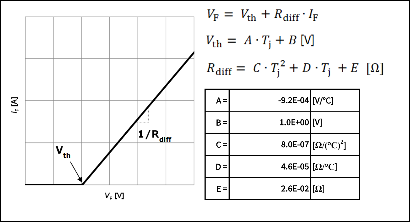
Figure 6 Simplified forward characteristics model V_F = f(I_F) ; -40^\circ\text{C} < T_j < 175^\circ\text{C} ; I_F < 32 A
