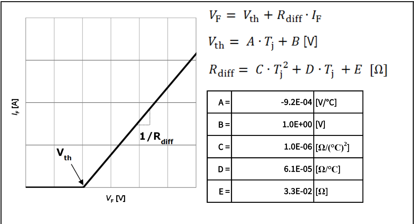
Figure 6 Simplified forward characteristics model V_F = f(I_F) ; -40^\circ\text{C} < T_j < 175^\circ\text{C} ; I_F < 24 A
