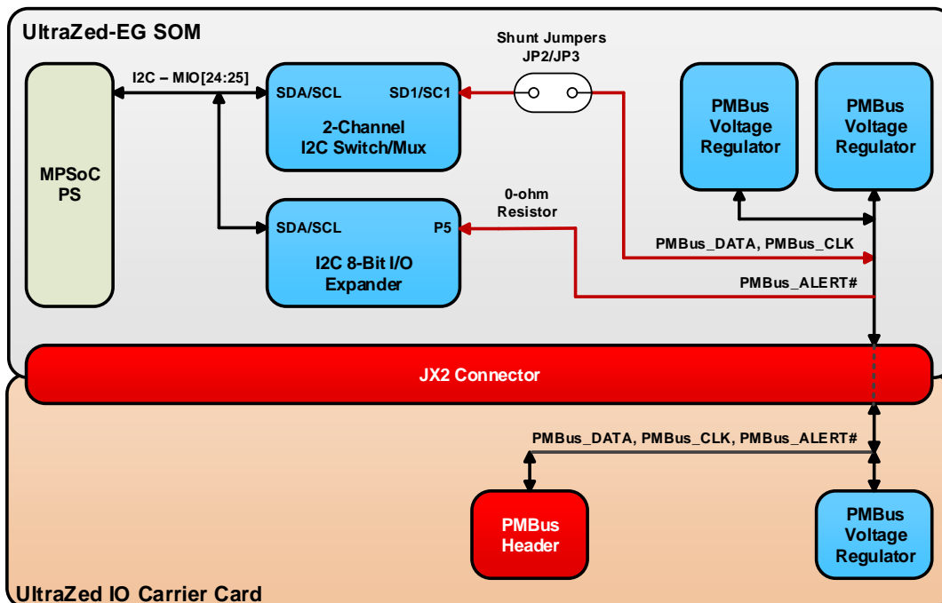
Figure 10 – PMBUS Connections
