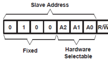
Figure 8 – I2C I/O Expander Addressing
