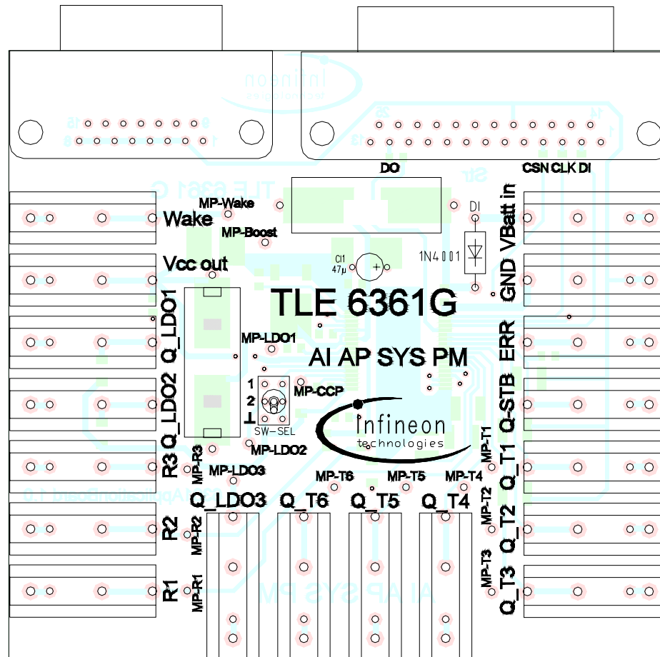
Mounting Diagram Upper Side:
