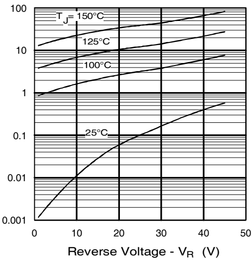
Fig. 2 - Typical Values of Reverse Current Vs. Reverse Voltage (Per Leg)
