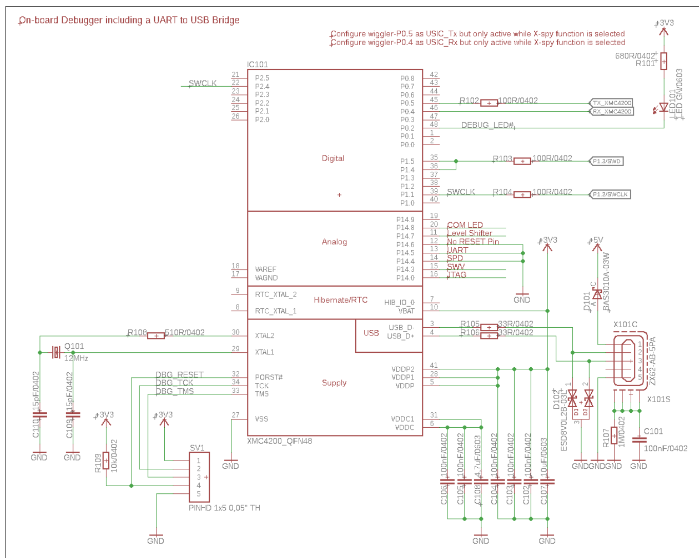
Figure 14 EvalBoard schematic: the XMC4200 microcontroller and micro USB connector
