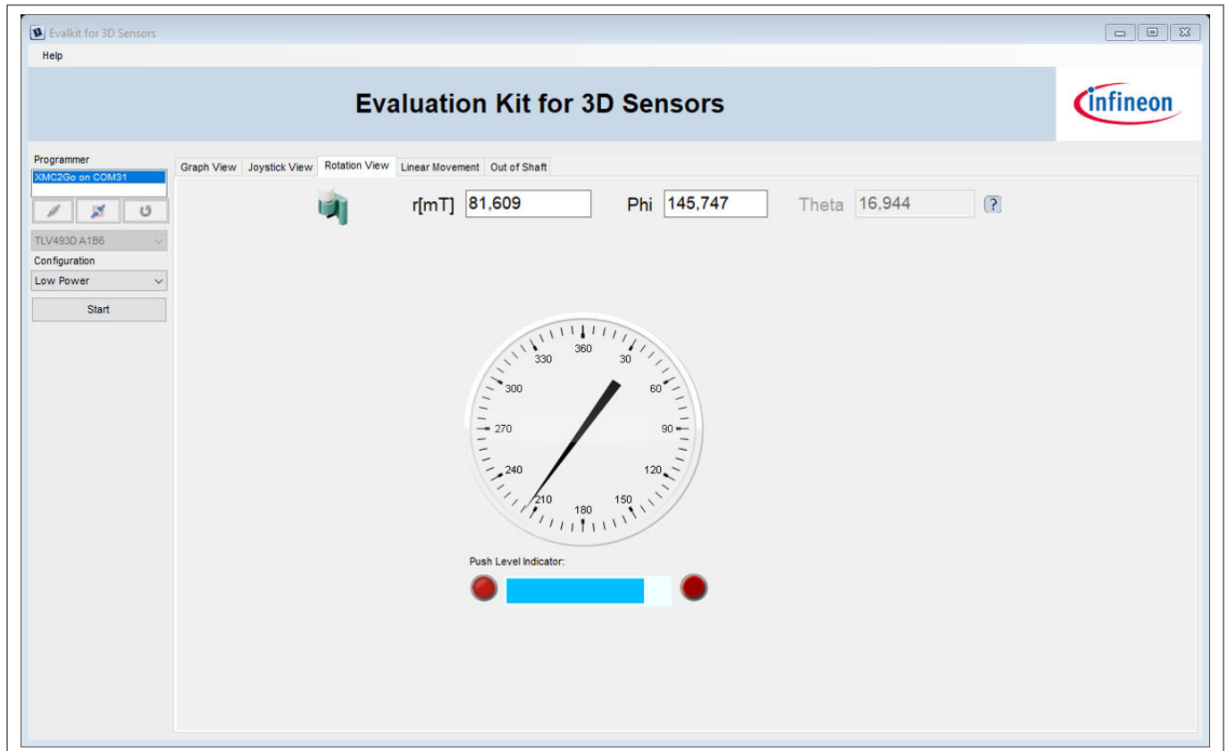
Figure 29 Polar coordinates
