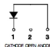
Case Outline and Dimensions - TO-254AA
