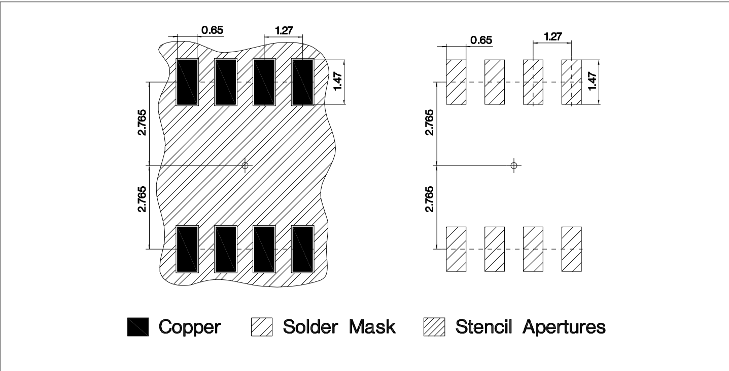
Figure 28 PG-DSO-8 footprint
