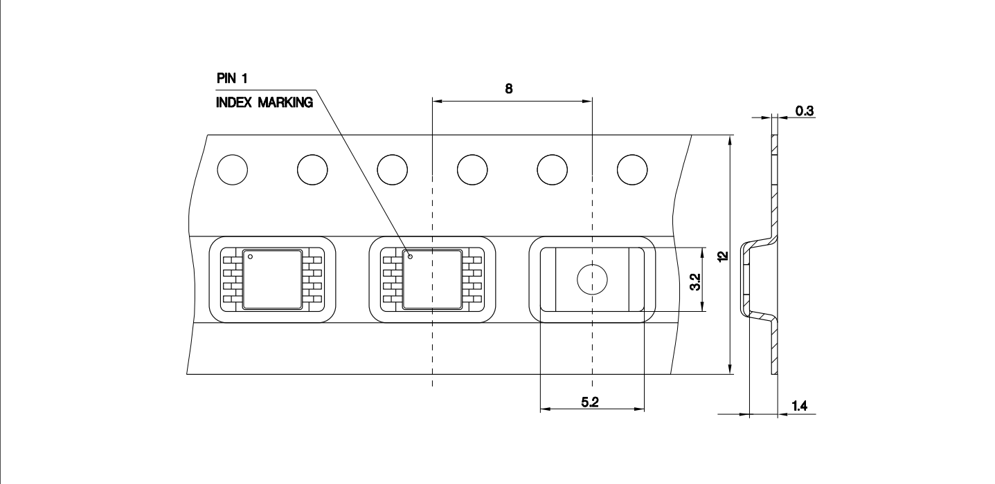
Figure 32 PG-TSSOP-8 packaging
