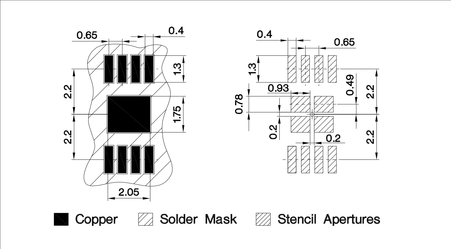
Figure 31 PG-TSSOP-8 footprint
