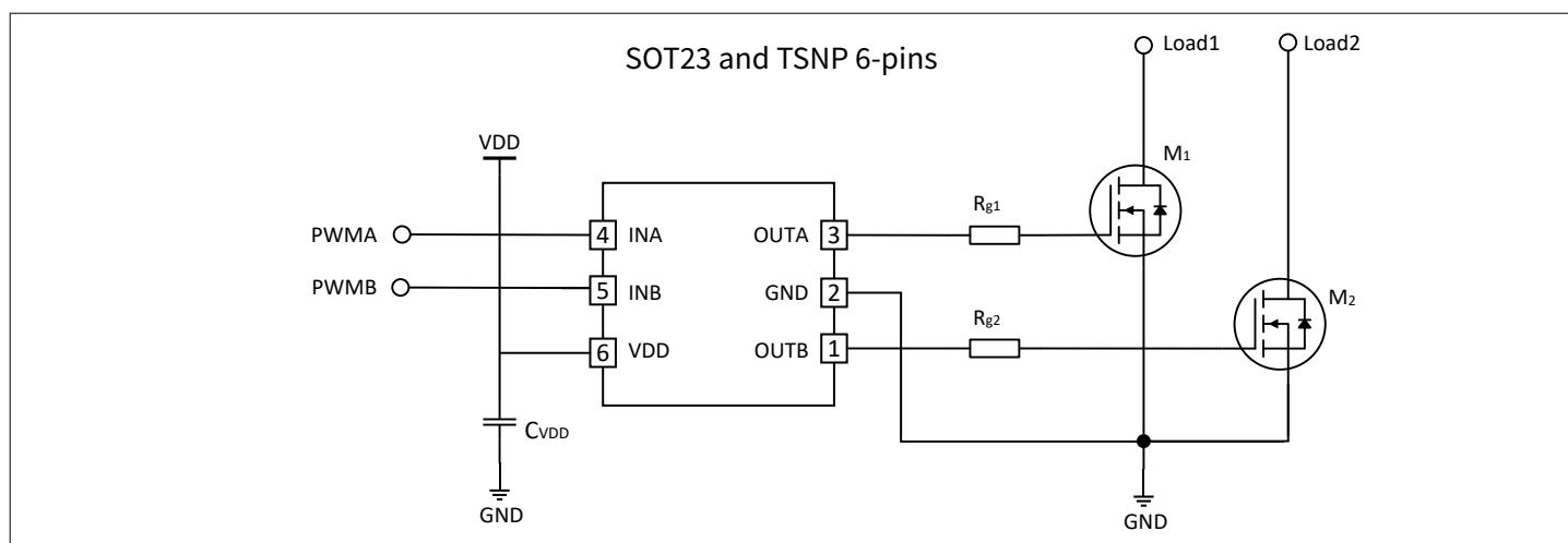
Figure 24 Typical application for 6-pin packages
