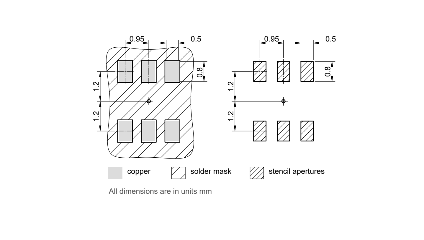
Figure 37 PG-SOT23-6 footprint
