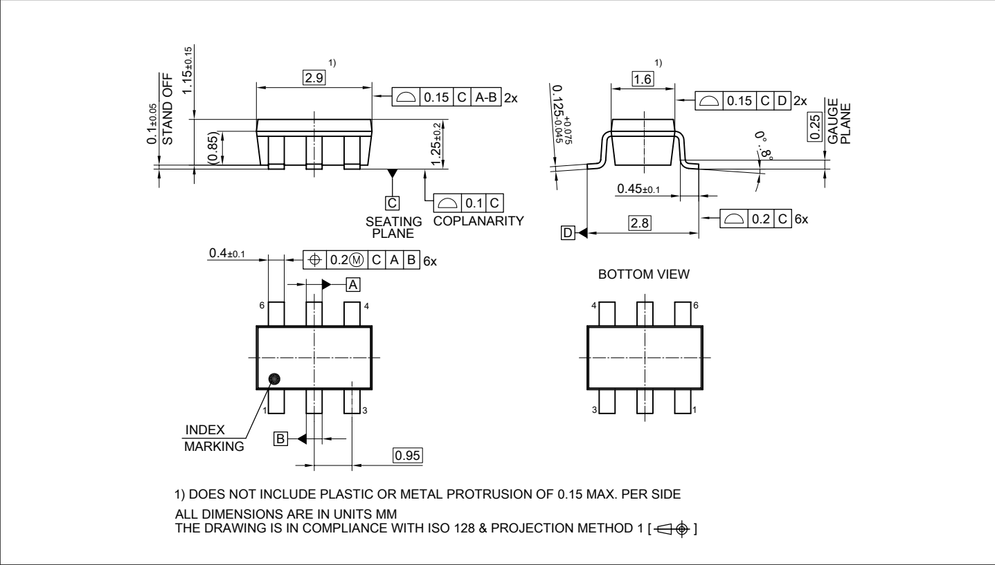
Figure 36 PG-SOT23-6 outline
