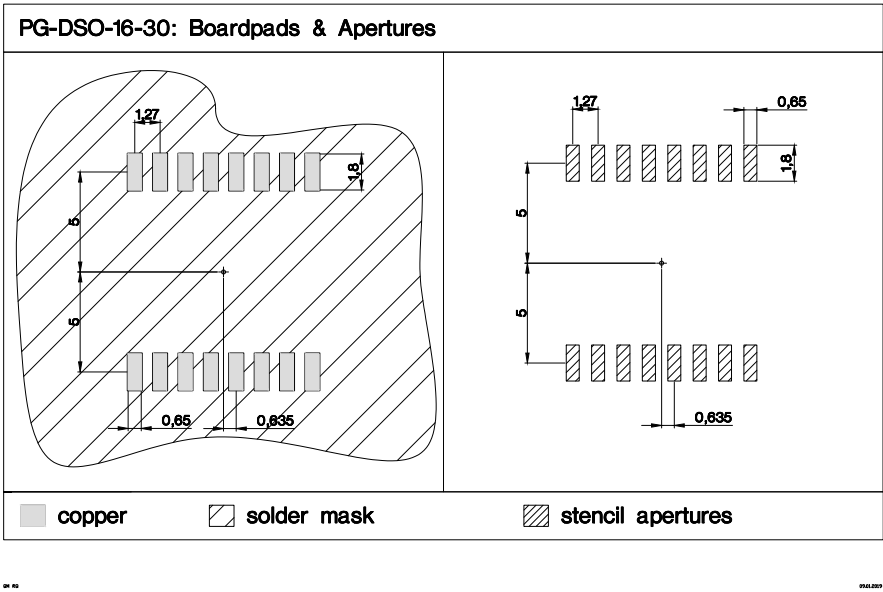
Figure 21 PG-DSO-16-30 footprint
