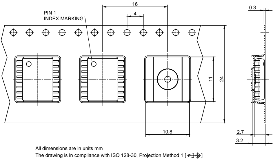
Figure 22 PG-DSO-16-30 packaging
