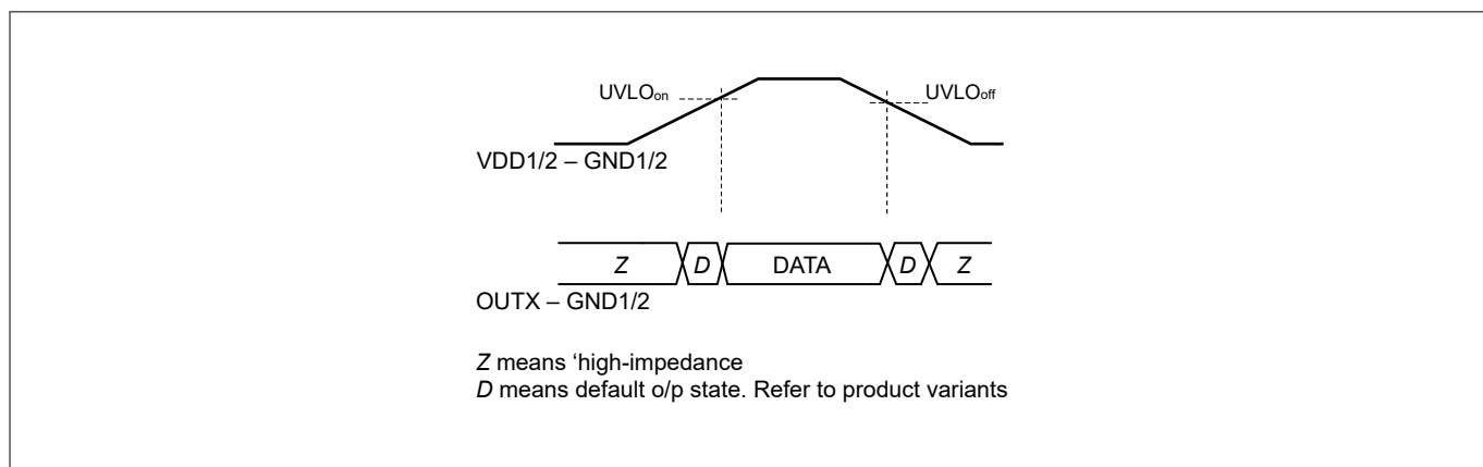
Figure 8 Under-voltage lockout
