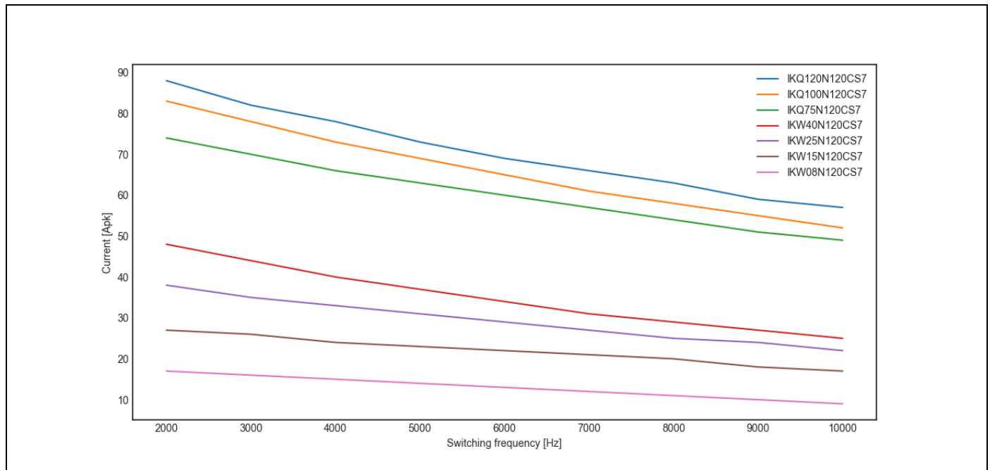
Figure 13 Derating curve of the discrete 1200 V TRENCHSTOP™ IGBT7 family, condition: 600 V DC , R_{thCH}=1\text{ K/W} , heat sink temperature=100°C, \cos(\phi)=1 , m_{index}=1 , f_{ele}=50\text{ Hz} , R_G as per datasheet value
