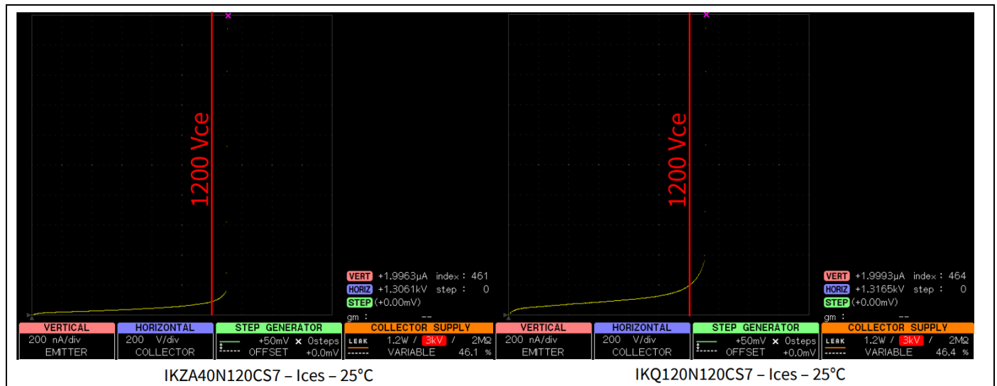
Figure 6 1200 V TRENCHSTOP™ IGBT7 S7 I_{CES} at 25°C
