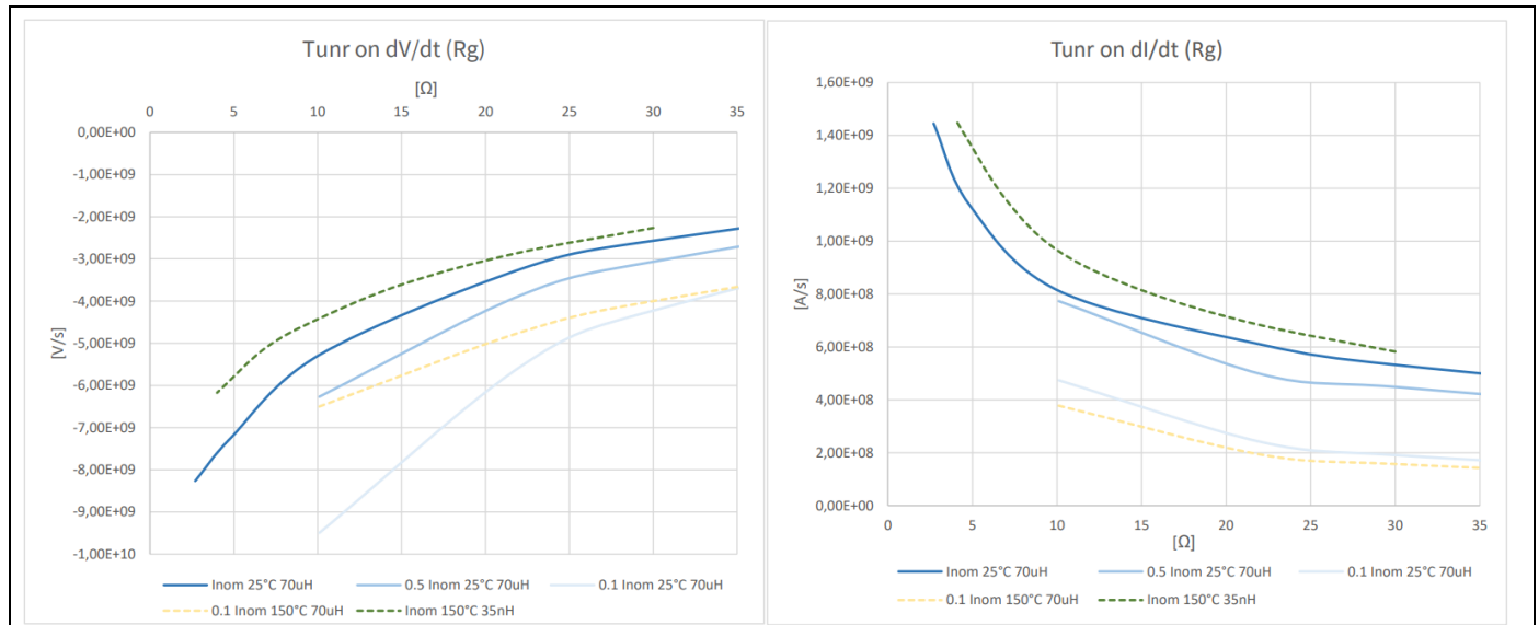
Figure 9 IKW40N120CS7 turn-on at 600 V V_{GE-} = 0 V V_{GE+} = 15 V, dV/dt (R_g) and dI/dt (R_g) with parasitic inductance, current and temperature influences
