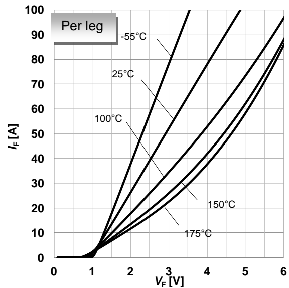
Figure 4. Typical forward characteristics in surge current per leg, I_F=f(V_F) , t_p=10 \mu s , parameter: T_j
