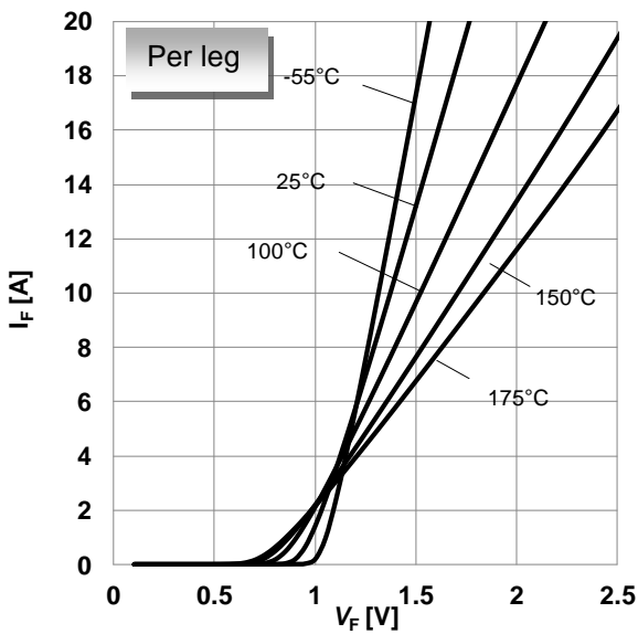
Figure 3. Typical forward characteristics per leg, I_F=f(V_F) , t_p=10 \mu s , parameter: T_j
