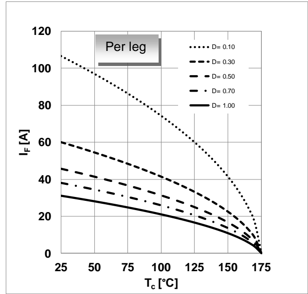
Figure 2. Diode forward current per leg as function of temperature, parameter: T_j \leq 175^\circ C , R_{th(j-c),max} , D =duty cycle, V_{th} , R_{diff} @ T_j=175^\circ C
