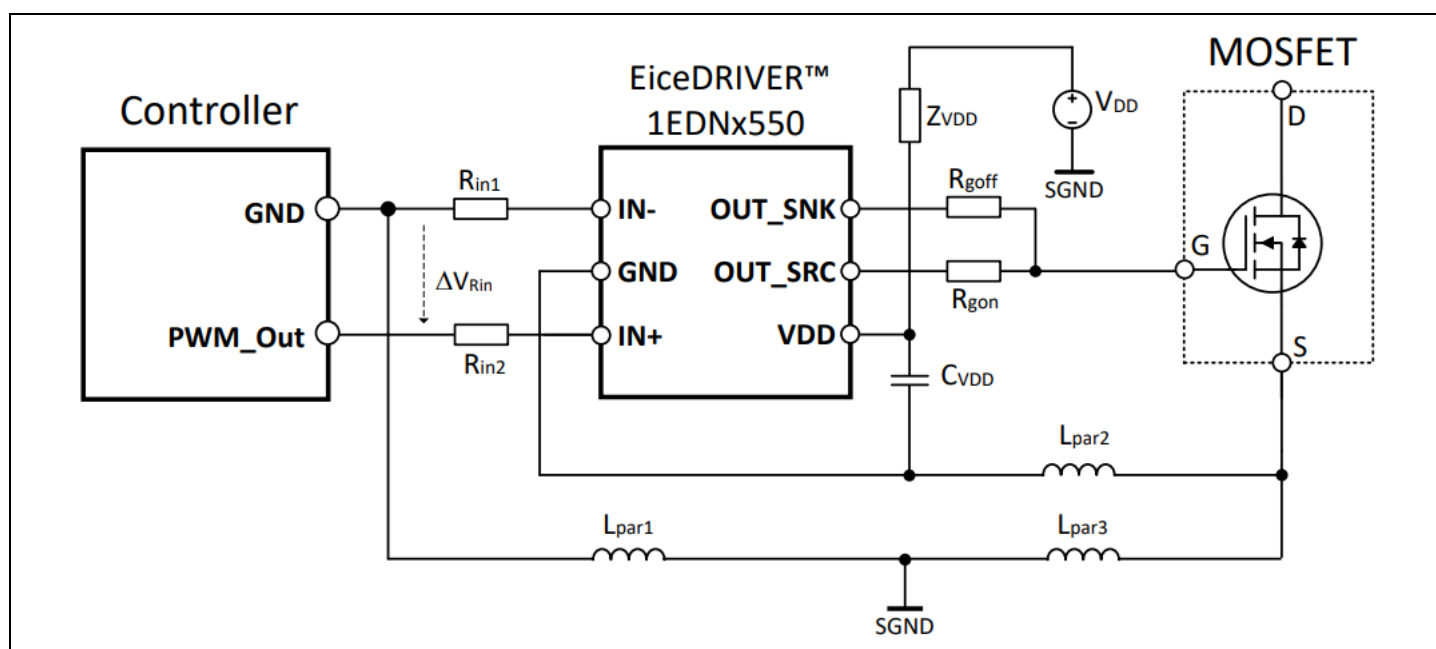
Figure 10 EiceDRIVER™ 1EDNx550 in applications with significant PCB inductances
