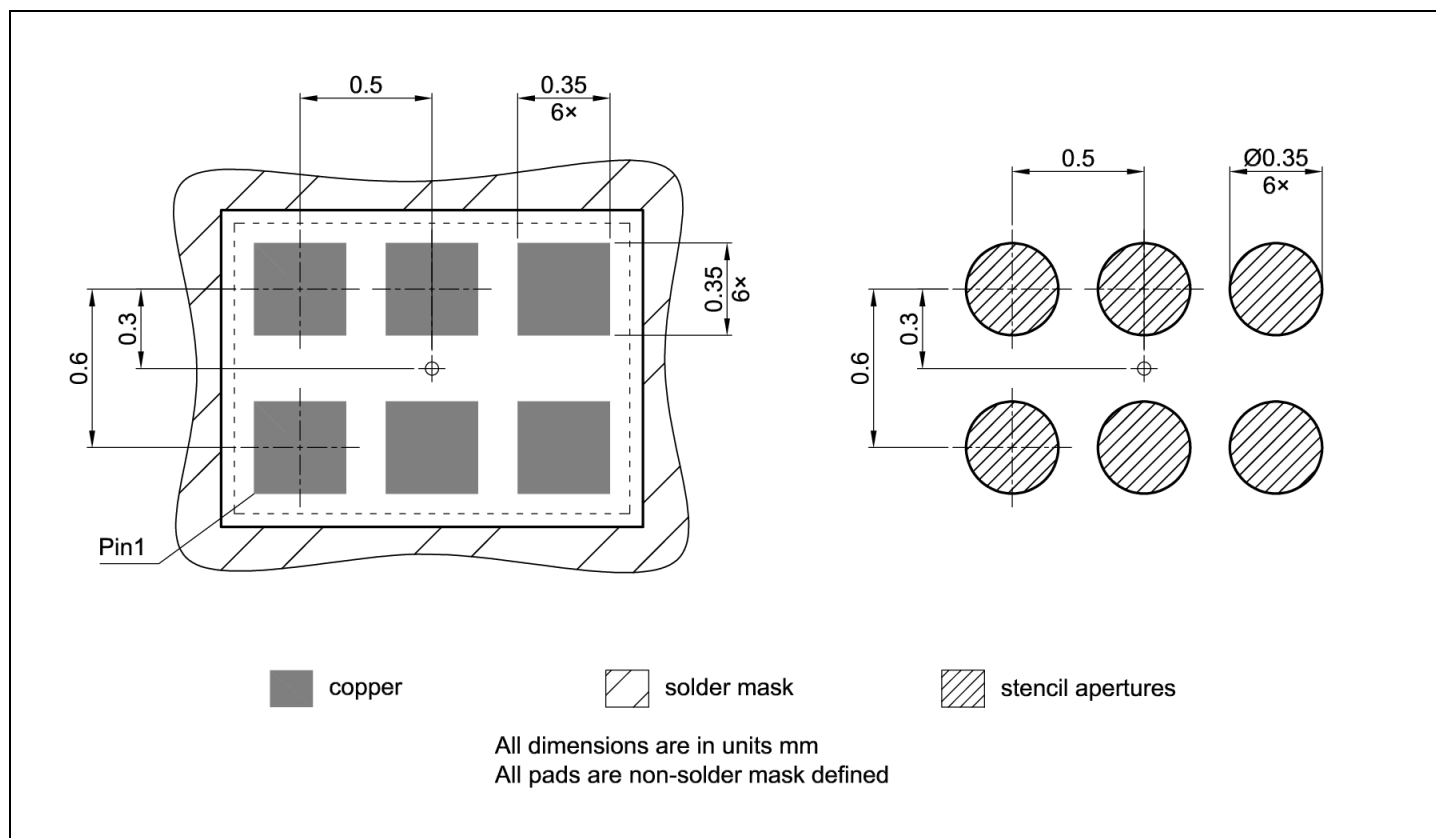
Figure 20 TSNP-6 footprint
