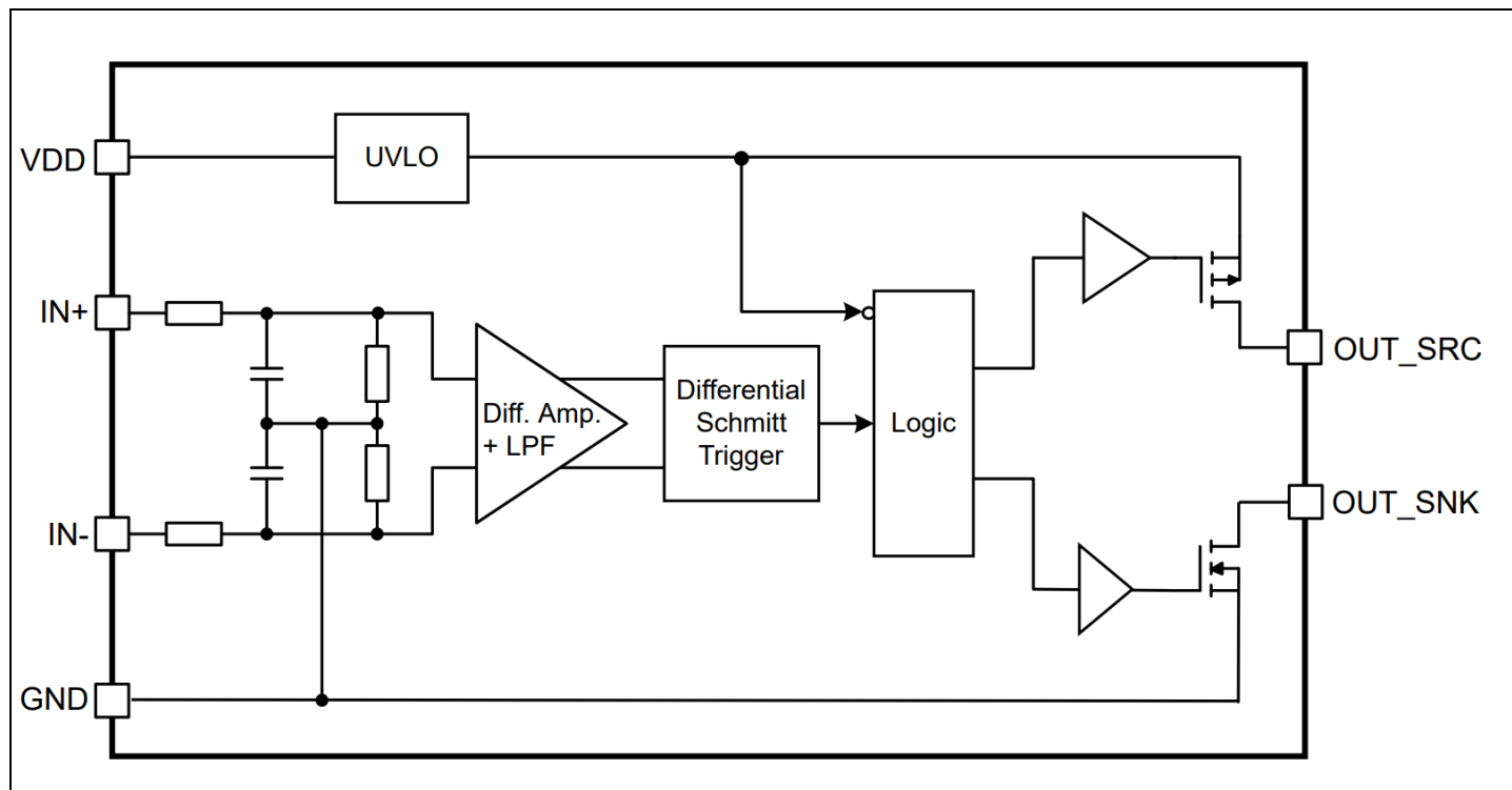
Figure 3 Simplified block diagram of EiceDRIVER™ 1EDNx550
