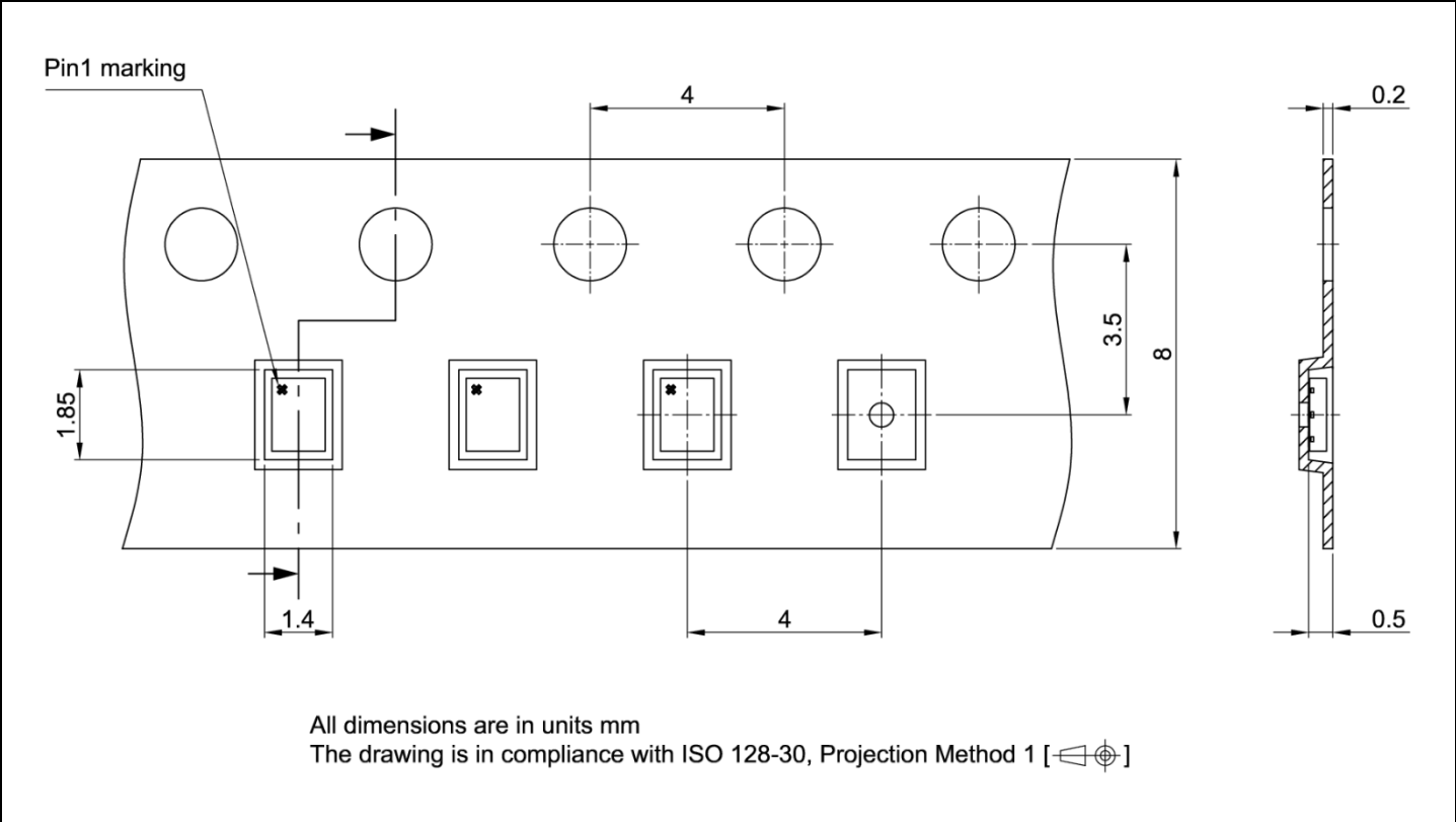
Figure 21 TSNP-6 packaging
