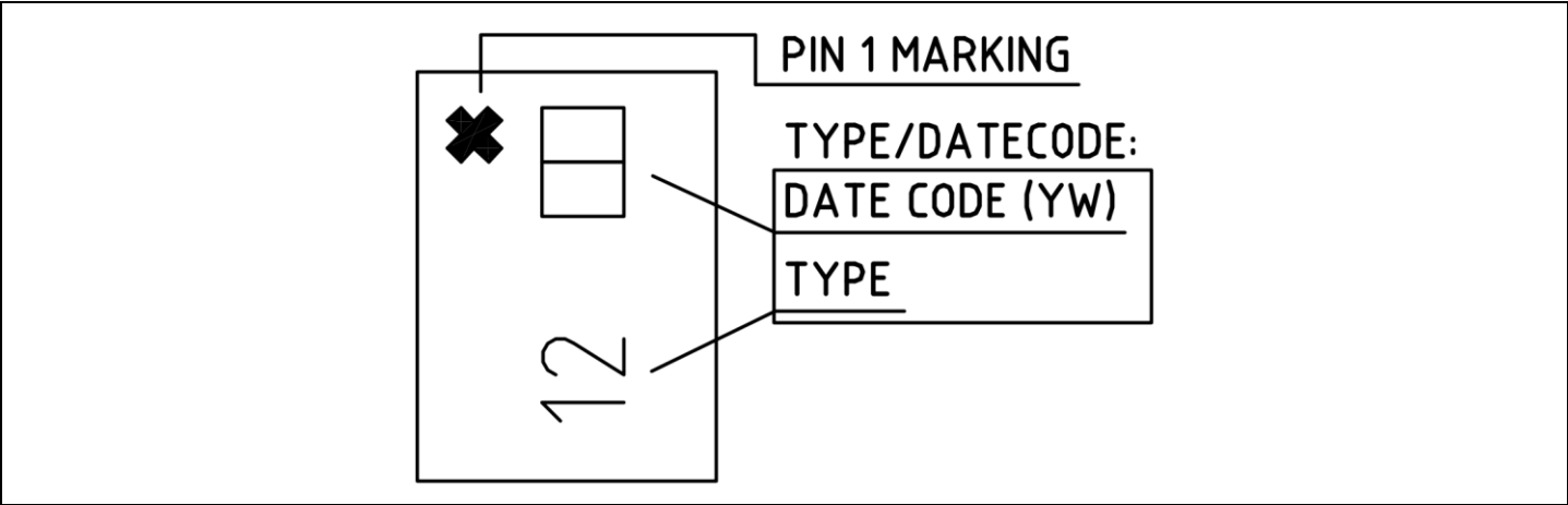
Figure 22 Package marking (TSNP-6)
