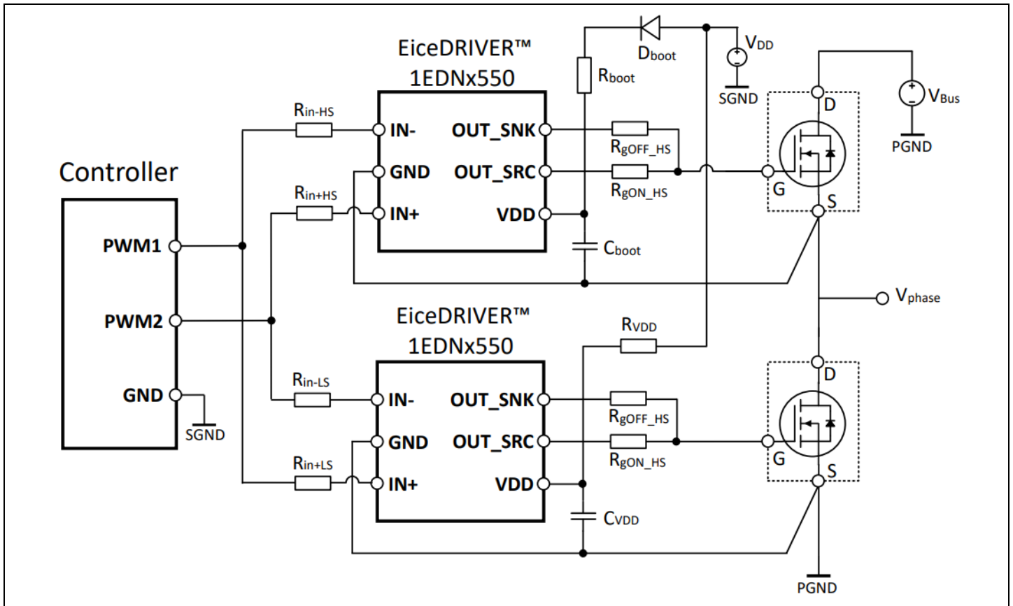
Figure 8 EiceDRIVER™ 1EDNx550 in half-bridge applications
