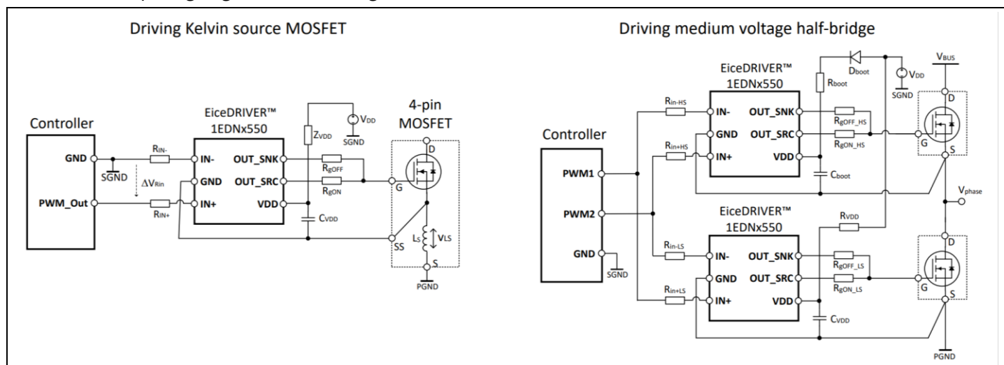
Figure 1 EiceDRIVER™ 1EDNx550 driving Kelvin-source MOSFET and half-bridge power stages
