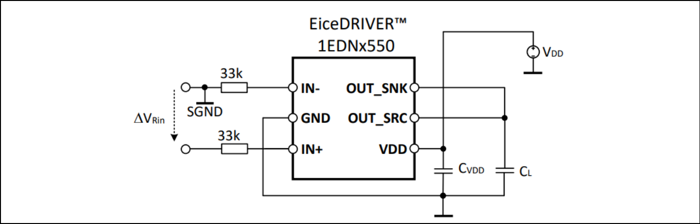
Figure 5 Test circuit
