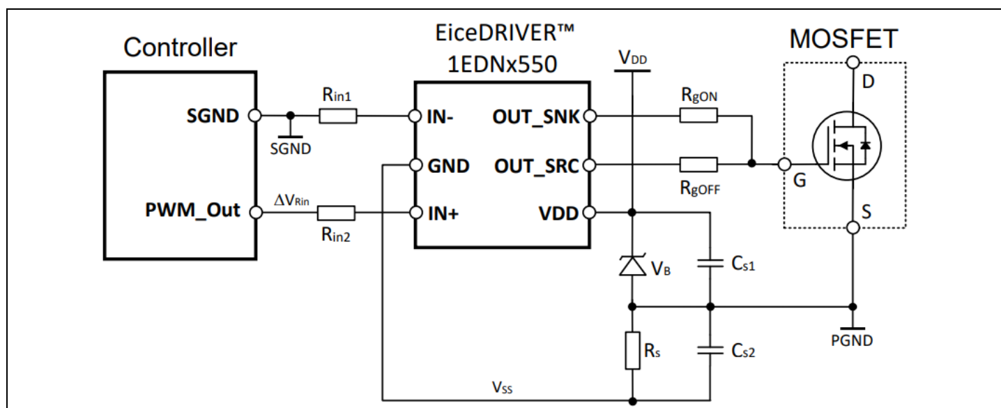
Figure 11 Bipolar gate drive for 3-pin MOSFET
