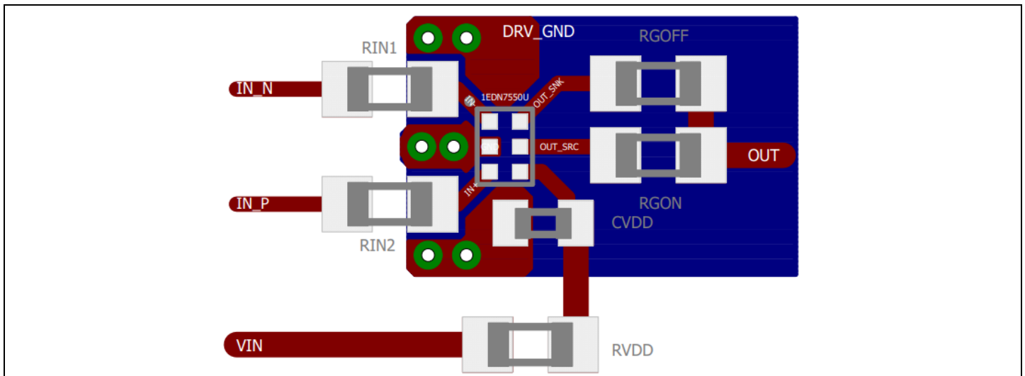
Figure 13 Layout recommendation for TSNP-6 package with SMD resistor 0603
