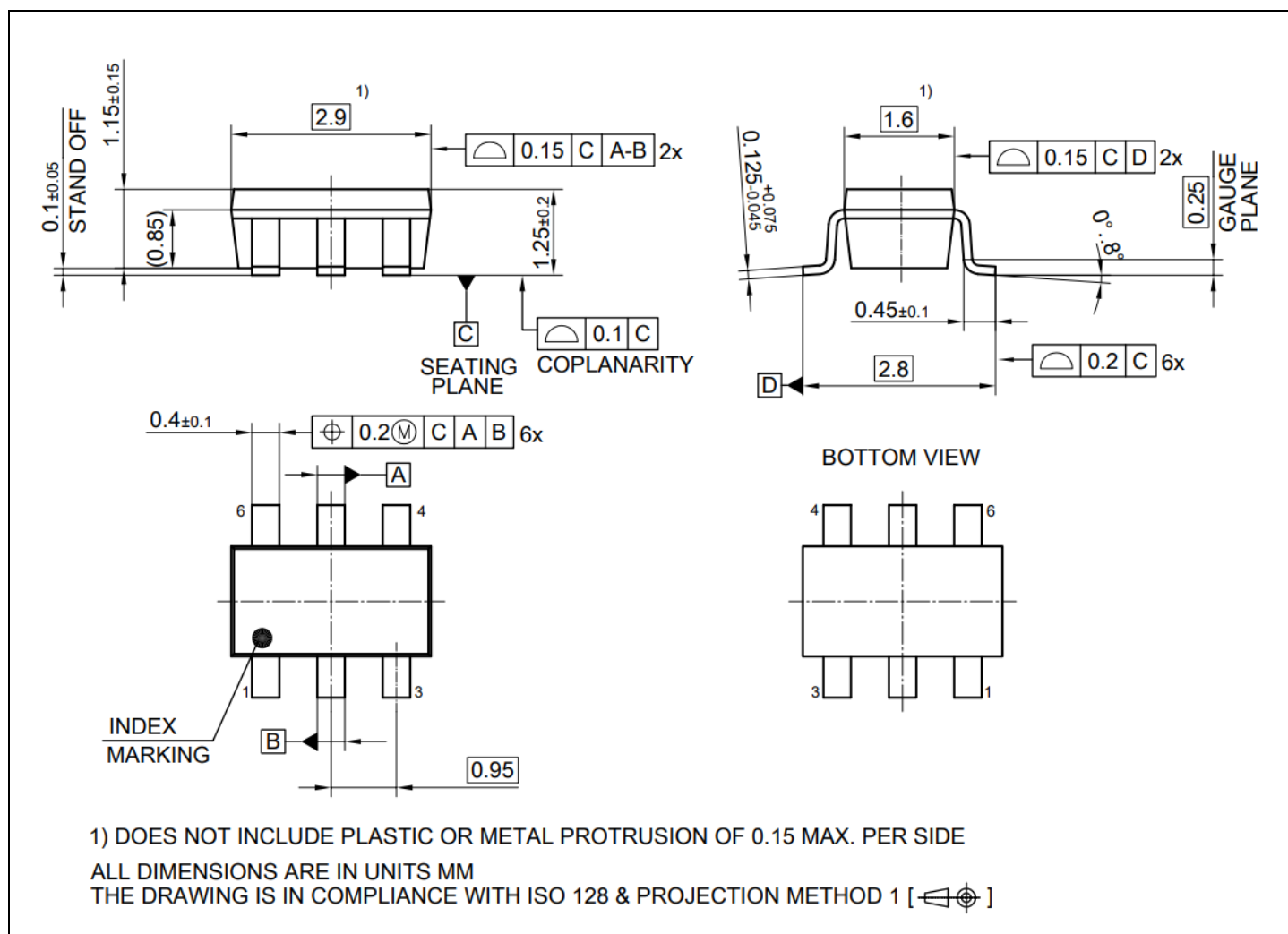
Figure 15 PG-SOT23-6 outline
