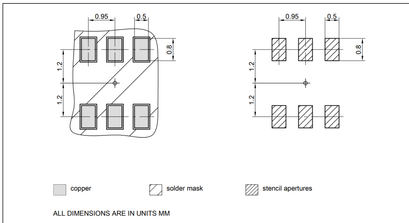
Figure 16 PG-SOT23-6 footprint
