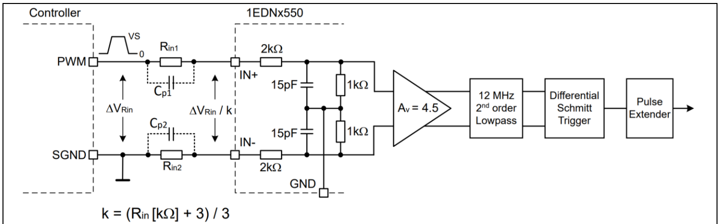
Figure 4 Functional principle of the EiceDRIVER™ 1EDNx550 with truly differential inputs (TDI)
