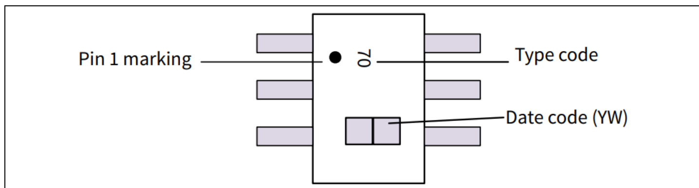
Figure 18 Package marking (PG-SOT23-6)
