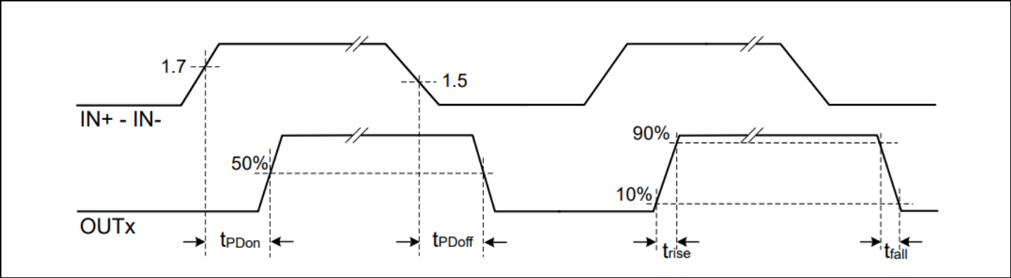
Figure 6 Propagation delay, rise and fall time
