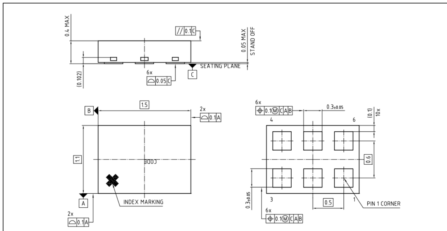
Figure 19 TSNP-6 outline
