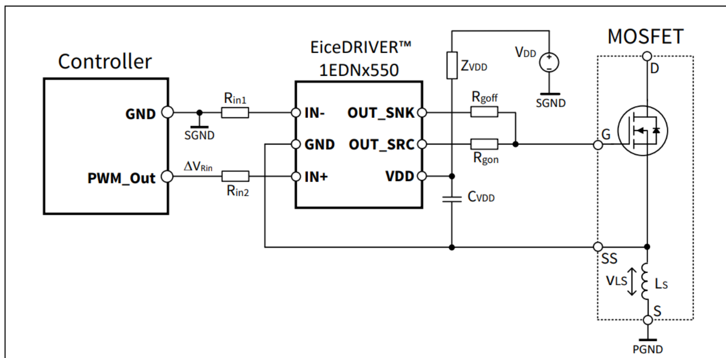
Figure 9 EiceDRIVER™ 1EDNx550 driving a Kelvin-source 4 pin MOSFET
