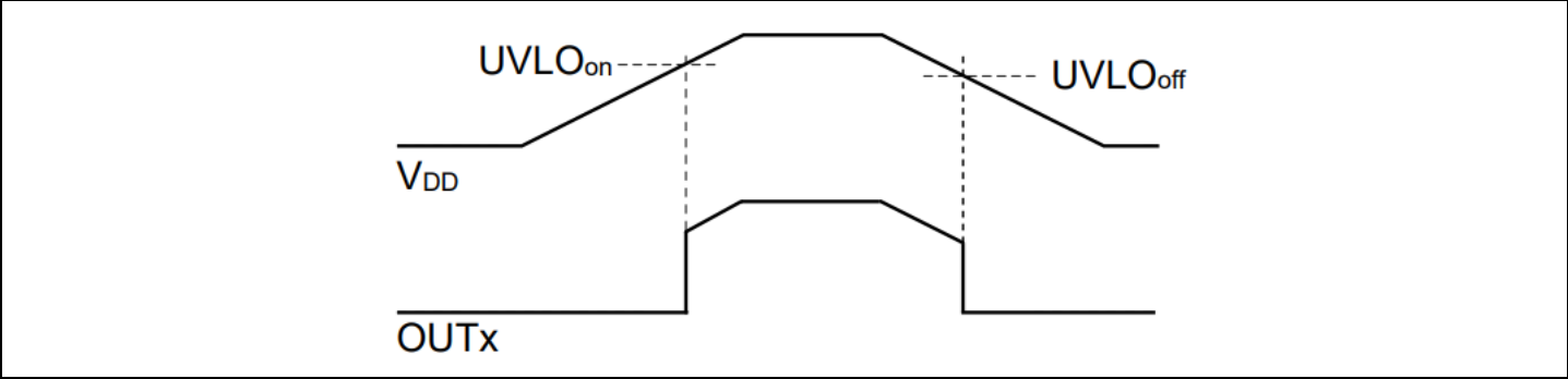
Figure 7 UVLO behavior (output state high)
