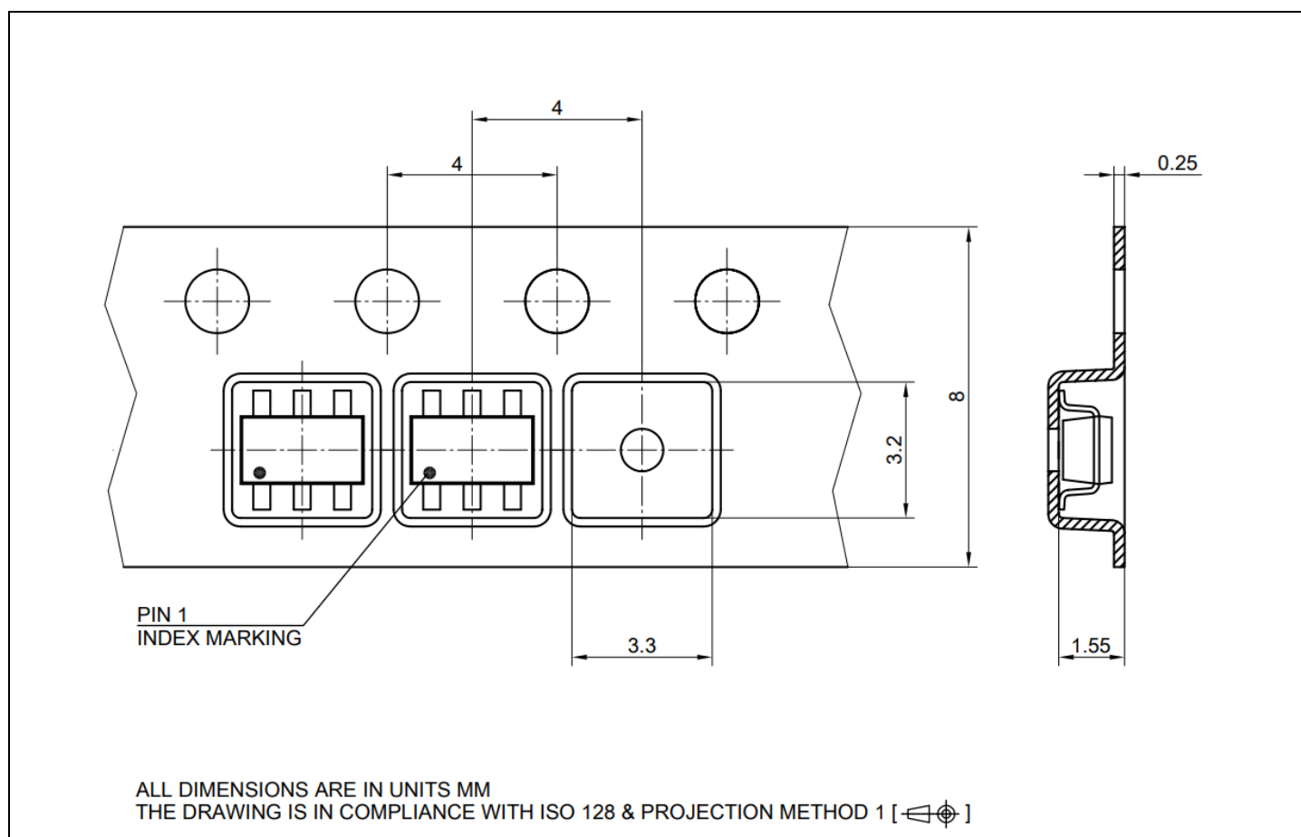
Figure 17 PG-SOT23-6 packaging
