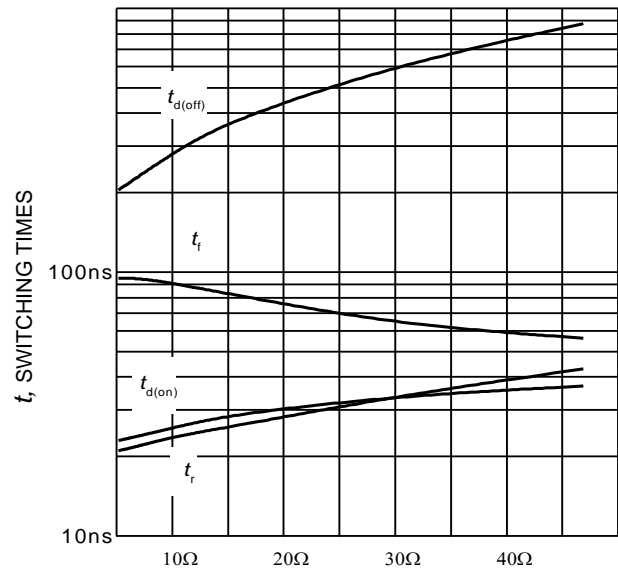
Figure 10. Typical switching times as a function of gate resistor (inductive load, T_J = 175^\circ\text{C} , V_{CE}= 400\text{V} , V_{GE} = 0/15\text{V} , I_C = 30\text{A} , Dynamic test circuit in Figure E)
