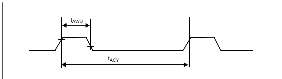
Figure 31 ALE Characteristic
