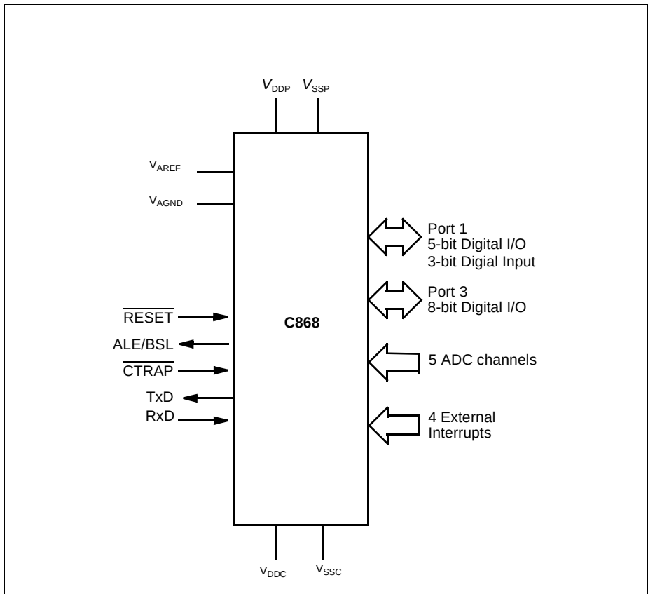
Figure 2 Logic Symbol
