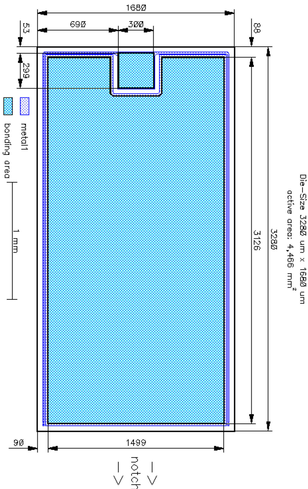
Figure 1 Outline Chip, dimensions in \mu\text{m}
