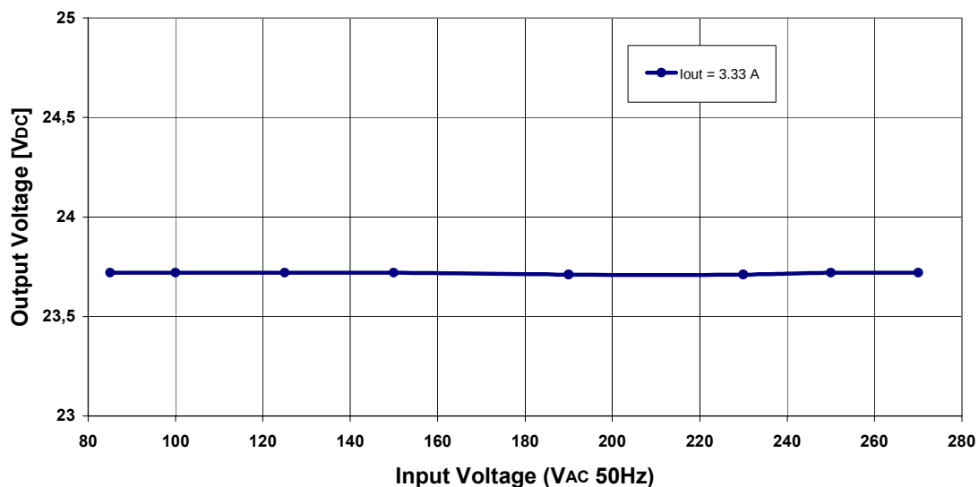
Figure 7 Regulation vs. Line Input Voltage
