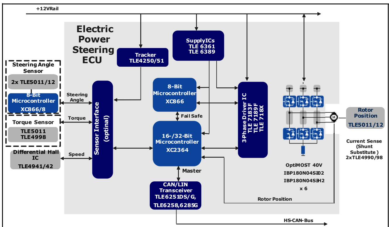
Figure 3 EPS Block Diagram
