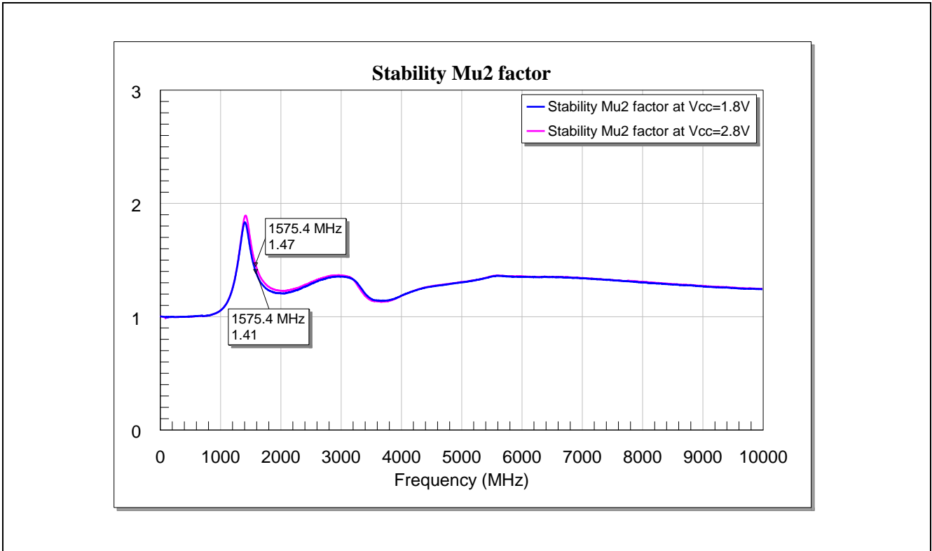
Figure 17 Stability factor \mu_2 of BGA925L6 upto 10GHz
