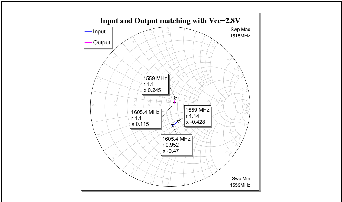
Figure 19 Input and output matching for COMPASS, Galileo, GPS and GLONASS bands with Vcc=2.8V
