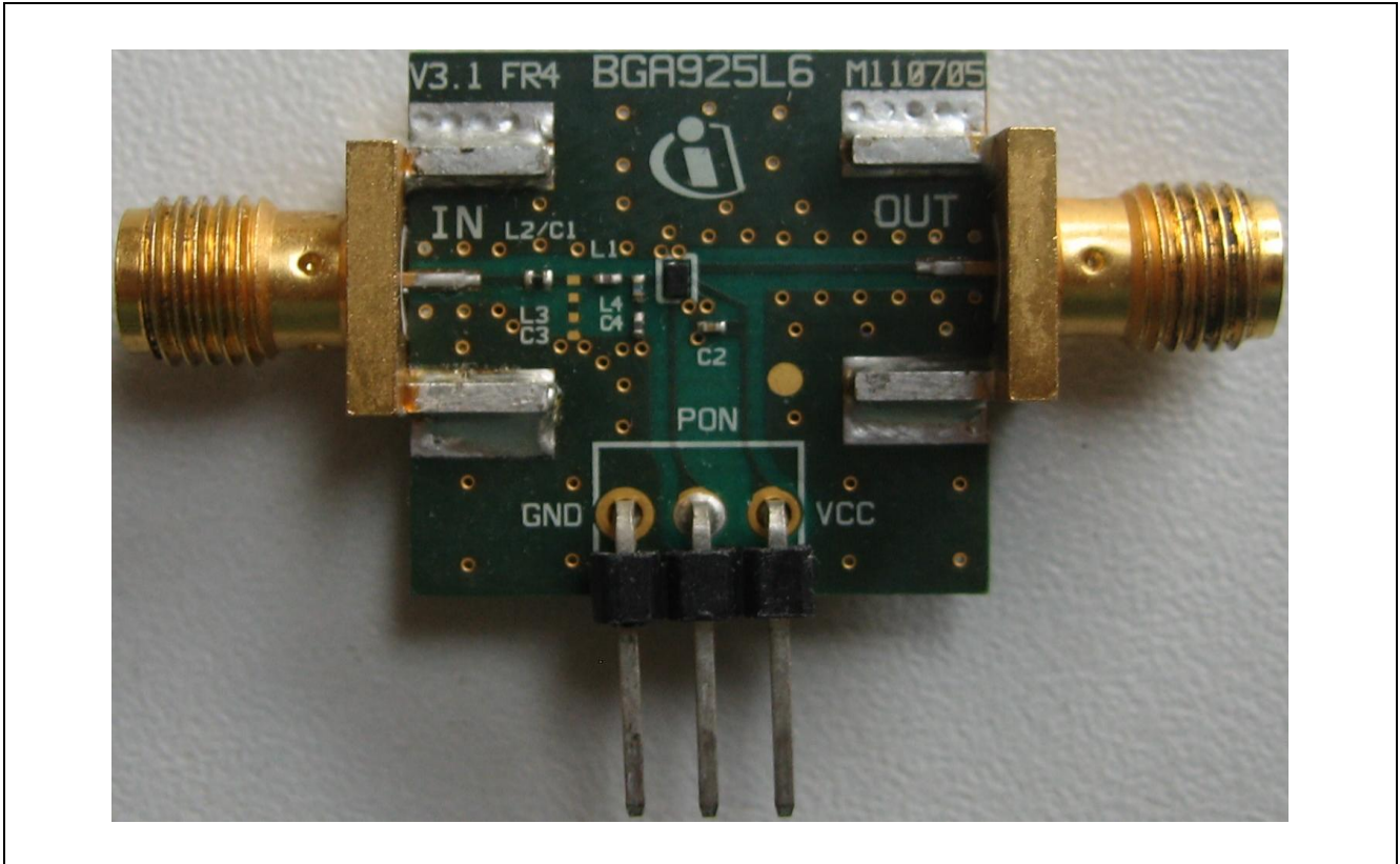
Figure 20 Populated PCB picture of BGA925L6
