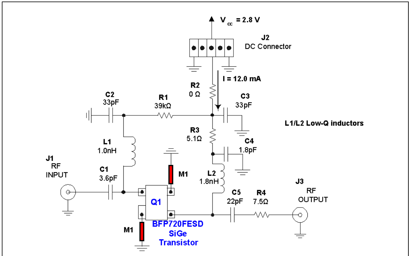
Figure 3 Schematic diagram of the application circuit
