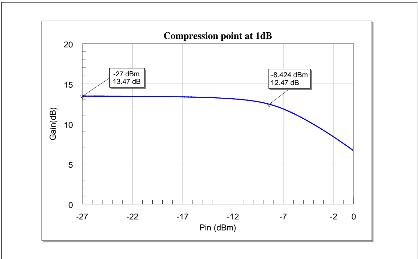
Figure 17 Input 1dB compression point of the BFP720FESD for WLAN/Wimax at 5-6GHz
