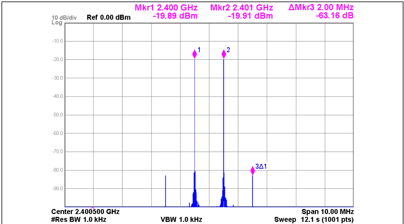
Figure 10 Output 3 rd order Intercept point of the BFP720FESD for WLAN/Wimax at 2.3-2.7GHz
