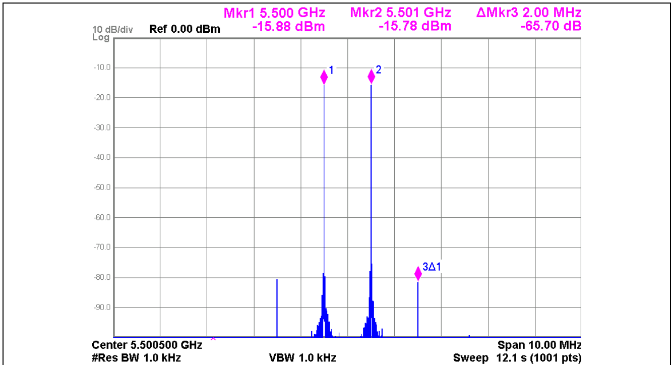
Figure 18 Output 3 rd order intercept point of the BFP720FESD for WLAN/Wimax at 5-6GHz
