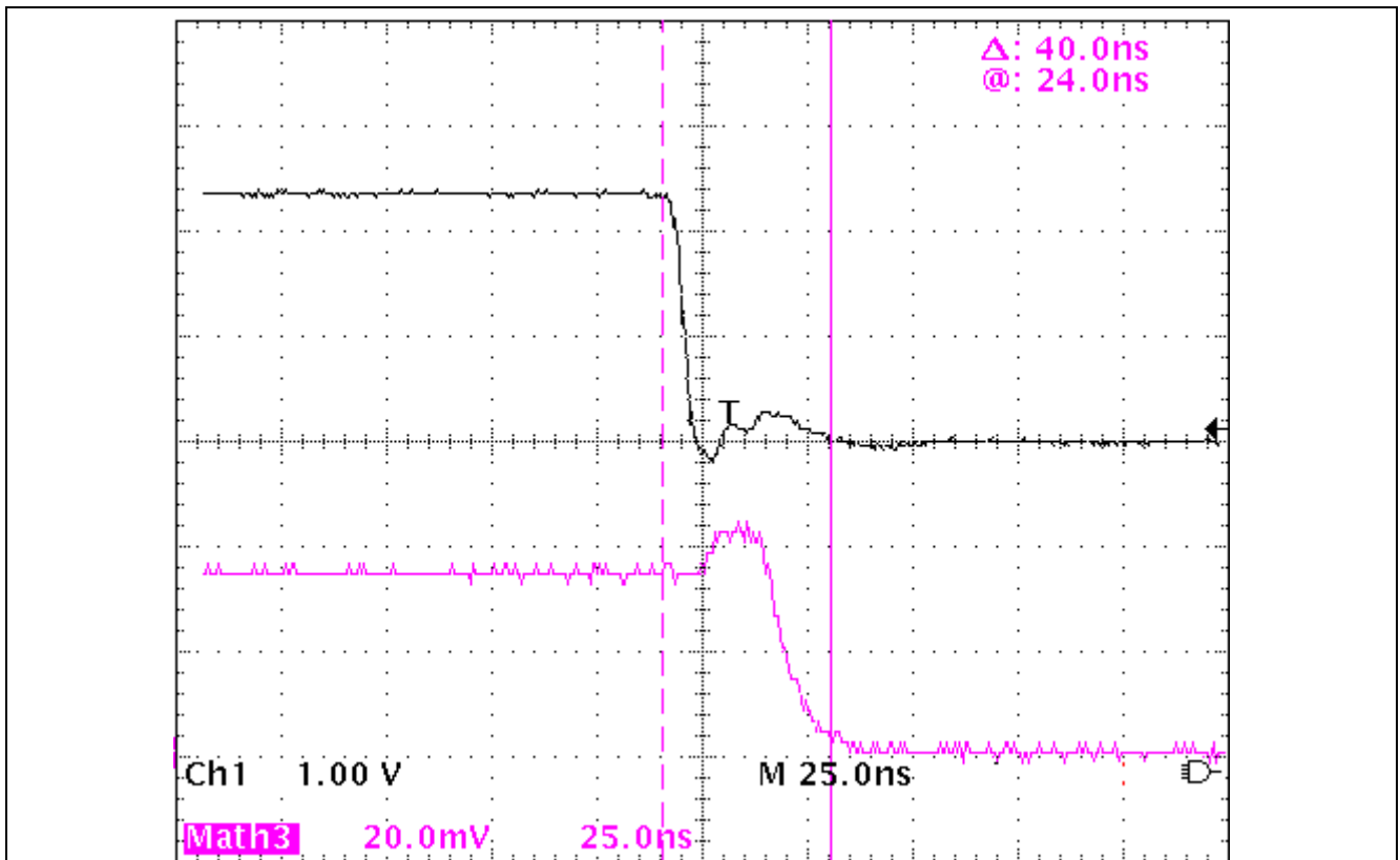
Figure 23 Fall switching time of the BFP720FESD for WLAN/Wimax 2.3-2.7&5-6GHz applications
