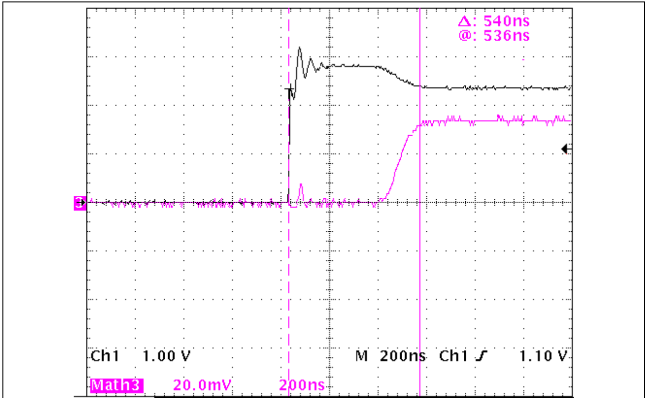
Figure 22 Rise switching time of the BFP720FESD for WLAN/Wimax 2.3-2.7&5-6GHz applications
