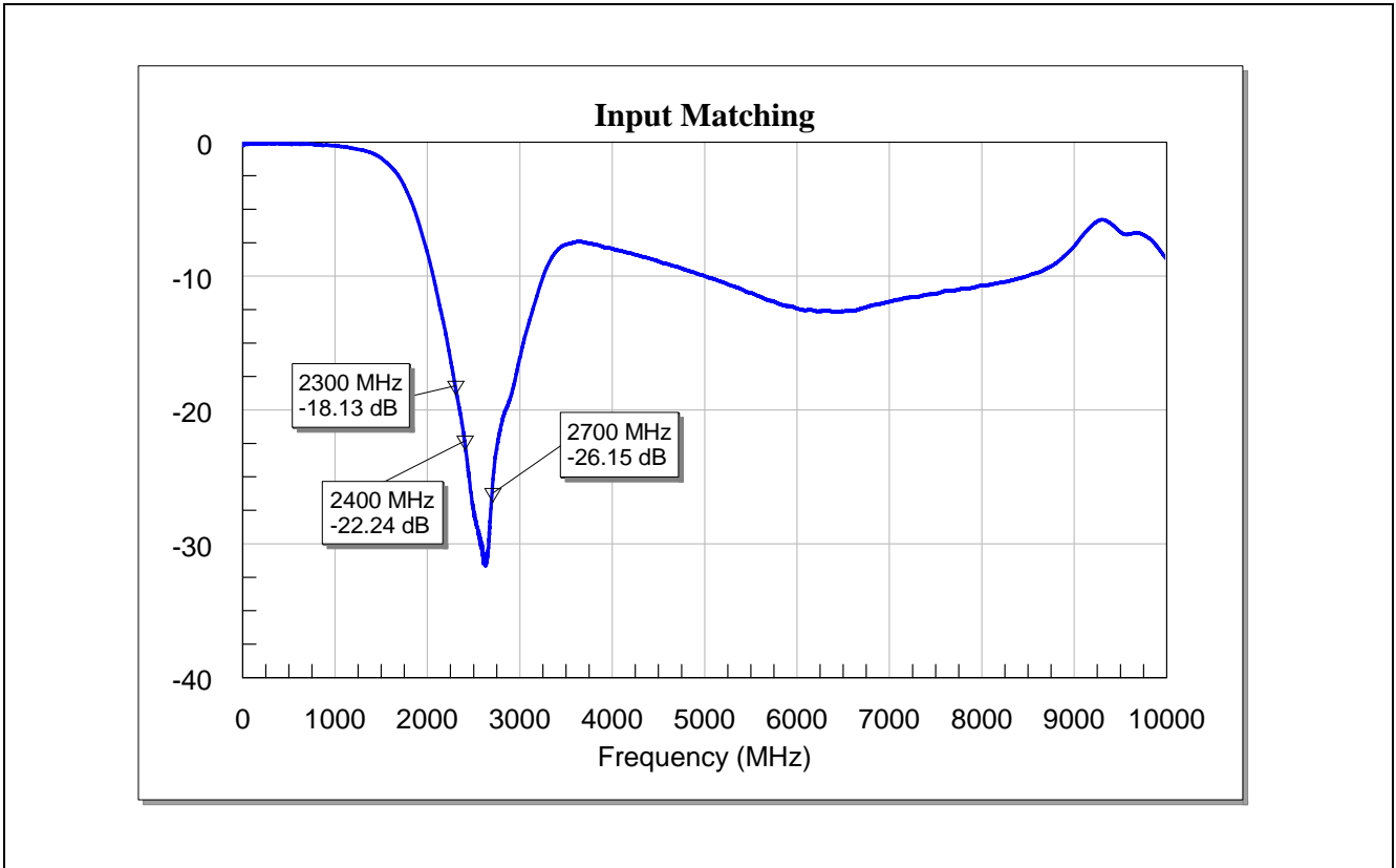
Figure 6 Input matching of the BFP720FESD for WLAN/Wimax at 2.3-2.7GHz
