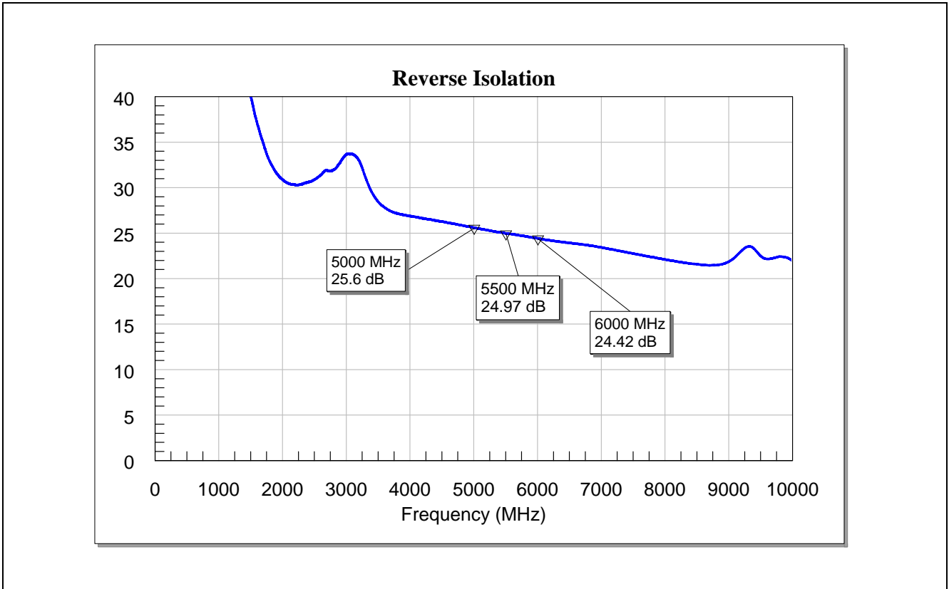
Figure 16 Reverse isolation of the BFP720FESD for WLAN/Wimax at 5-6GHz
