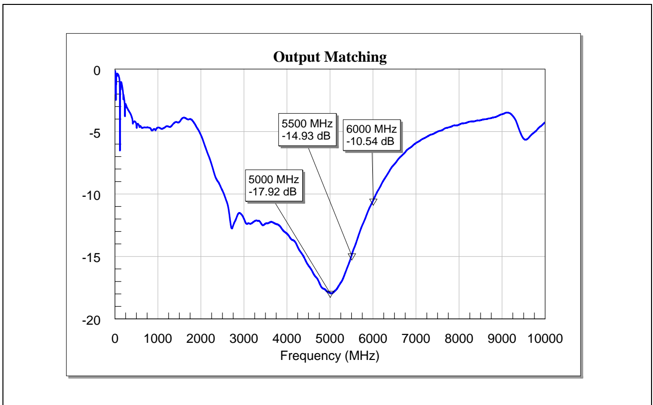
Figure 15 Output matching of the BFP720FESD for WLAN/Wimax at 5-6GHz
