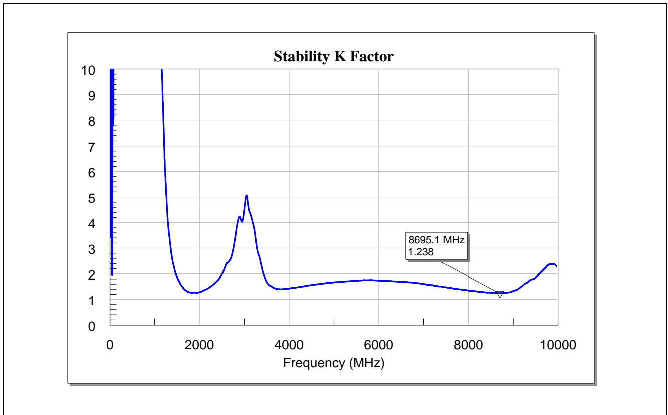
Figure 20 K-factor stability of the BFP720FESD for WLAN/Wimax 2.3-2.7&5-6GHz applications
