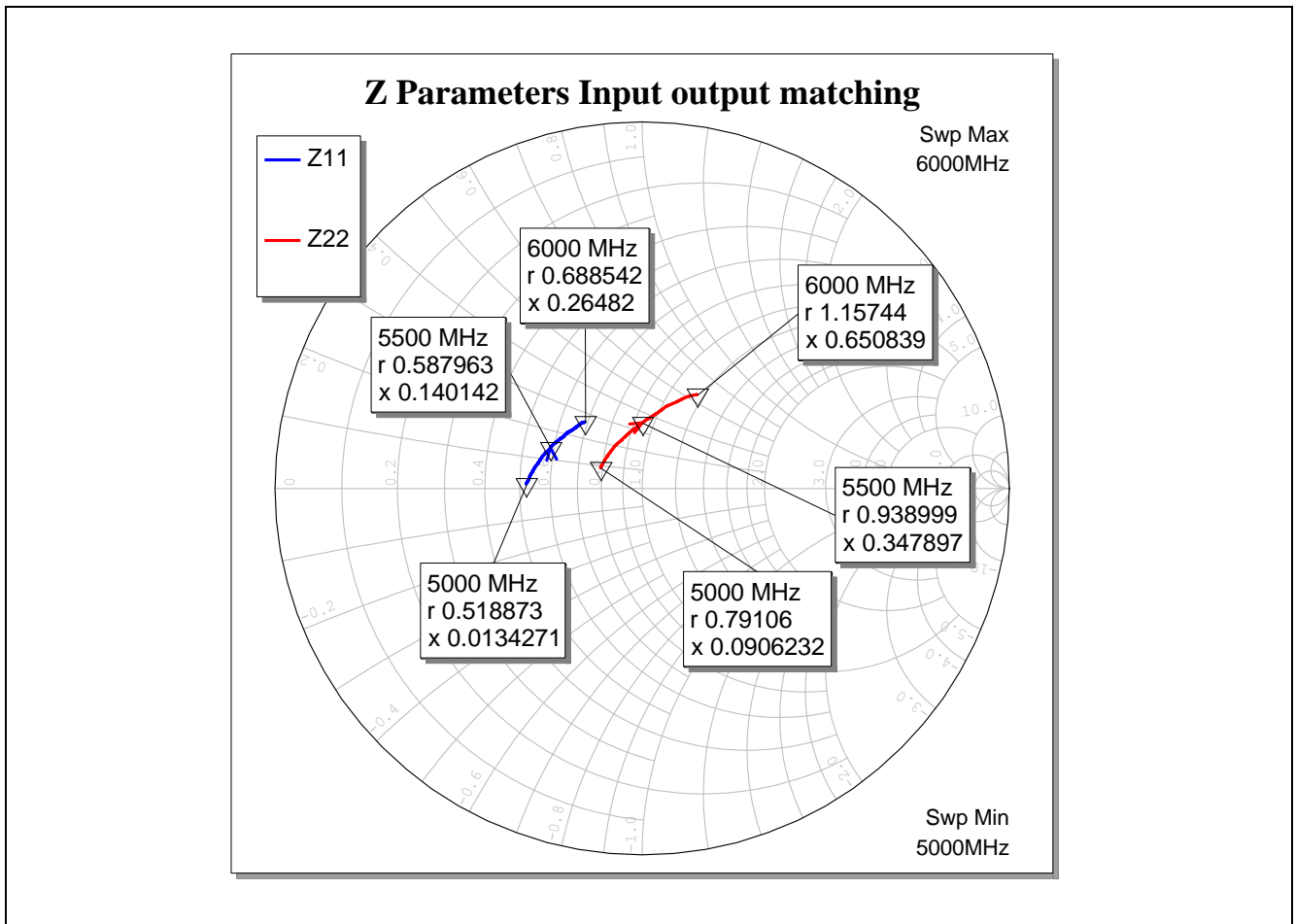
Figure 19 Input and Output impedance of the BFP720FESD for WLAN/Wimax at 5-6GHz
