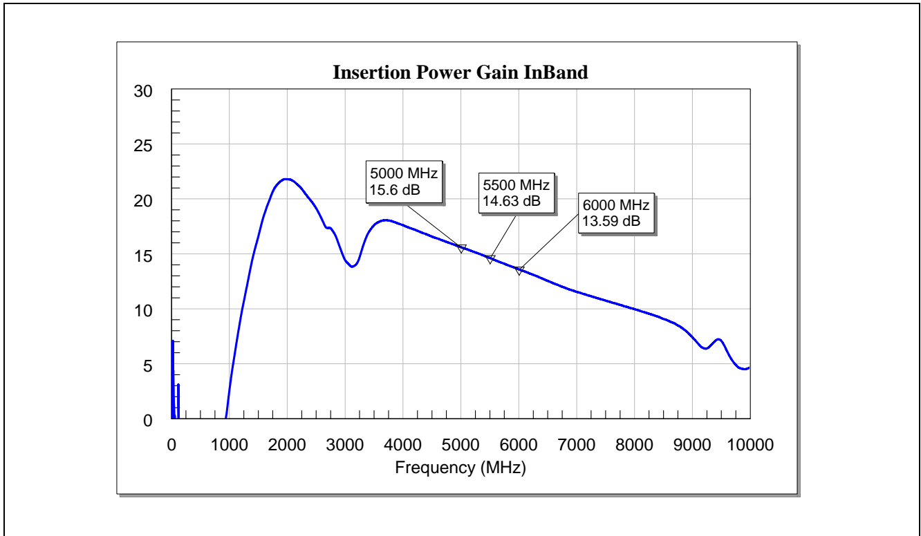
Figure 12 Insertion power gain of the BFP720FESD for WLAN/Wimax at 5-6GHz
