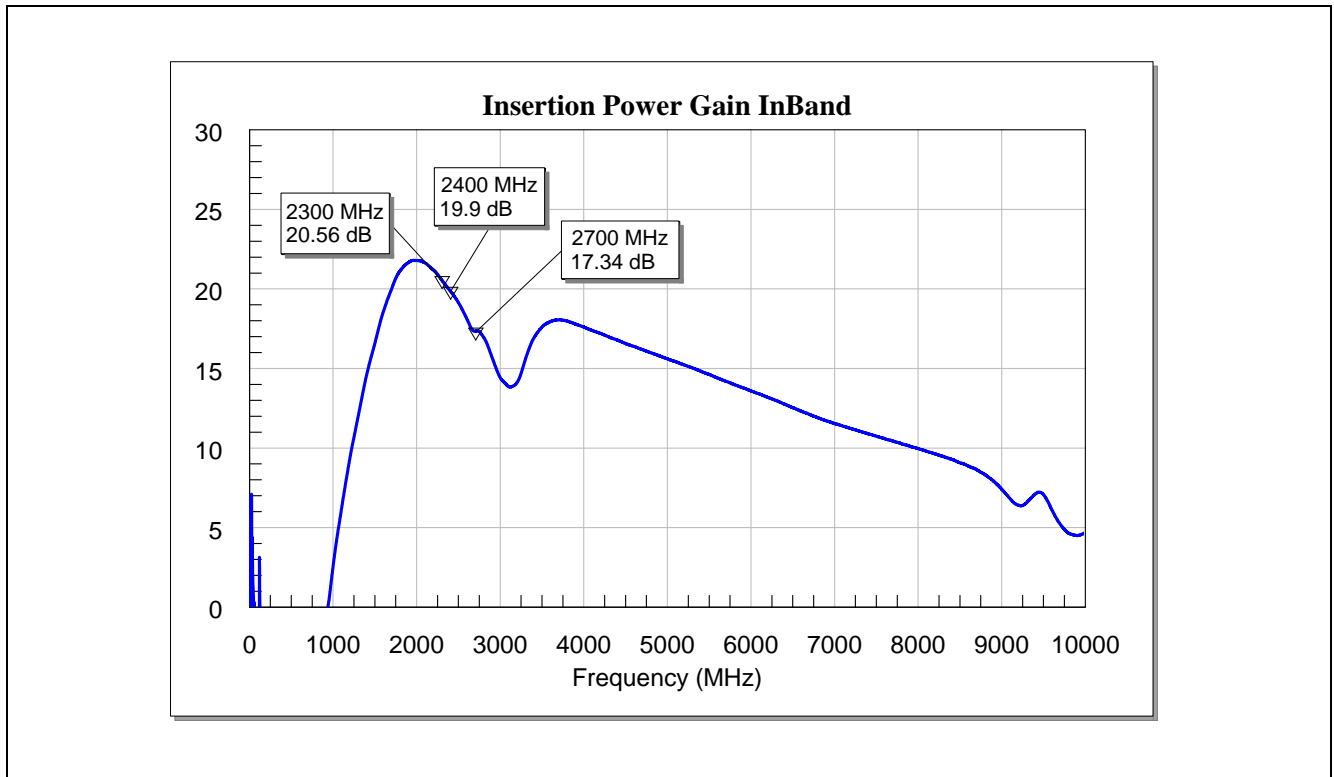
Figure 4 Insertion power gain of the BFP720FESD for WLAN/Wimax at 2.3-2.7GHz
