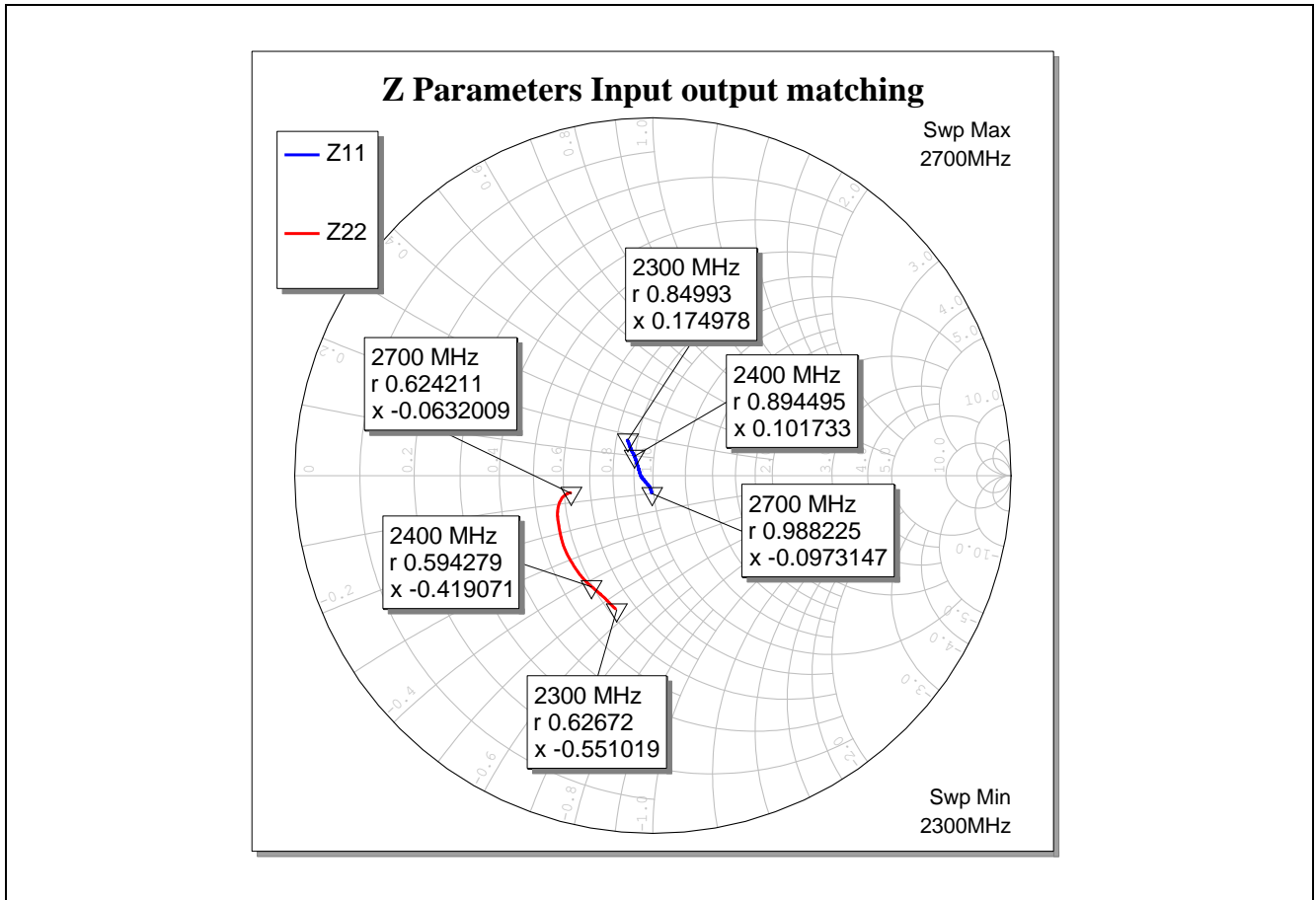
Figure 11 Input and Output impedance of the BFP720FESD for WLAN/Wimax at 2.3-2.7GHz
