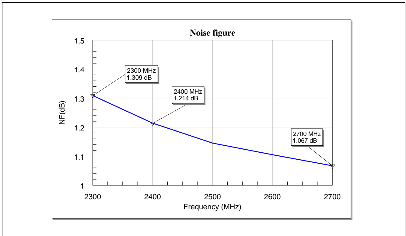
Figure 5 Noise figure of the BFP720FESD for WLAN/Wimax at 2.3-2.7GHz
