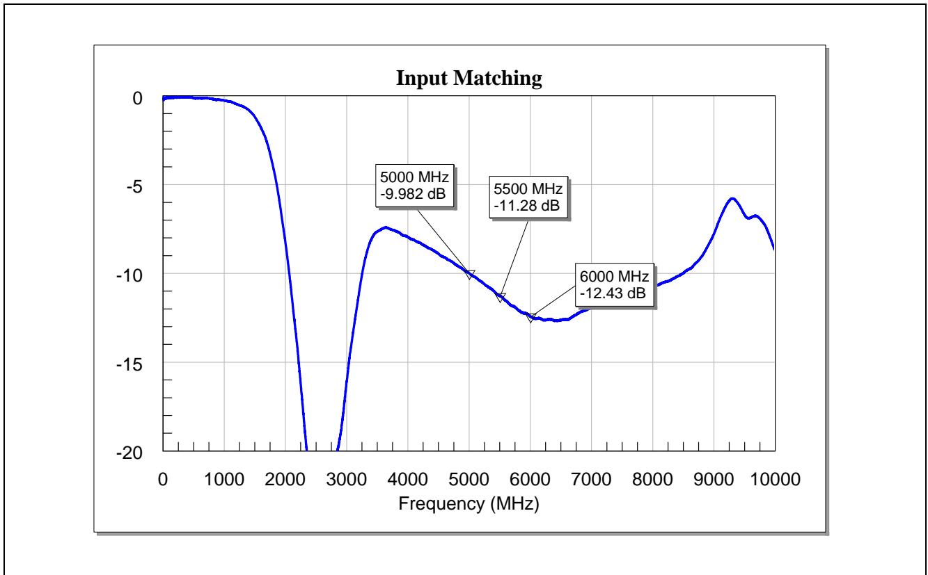
Figure 14 Input matching of the BFP720FESD for WLAN/Wimax at 5-6GHz
