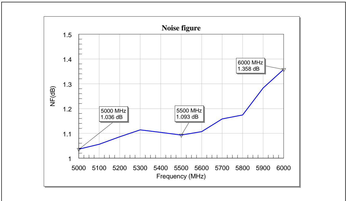
Figure 13 Noise figure of the BFP720FESD for WLAN/Wimax at 5-6GHz
