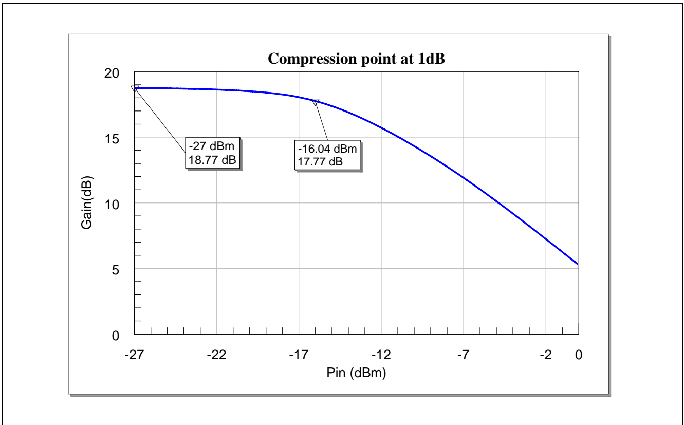
Figure 9 Input 1dB compression point of the BFP720FESD for WLAN/Wimax at 2.3-2.7GHz
