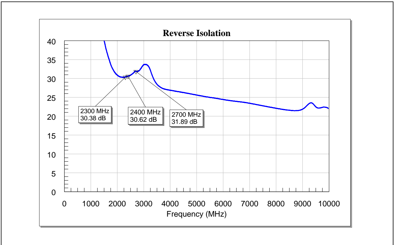
Figure 8 Reverse Isolation of the BFP720FESD for WLAN/Wimax at 2.3-2.7GHz
