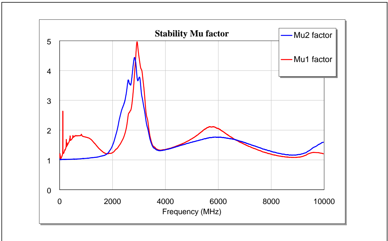
Figure 21 \mu -factor stability of the BFP720FESD for WLAN/Wimax 2.3-2.7&5-6GHz applications
