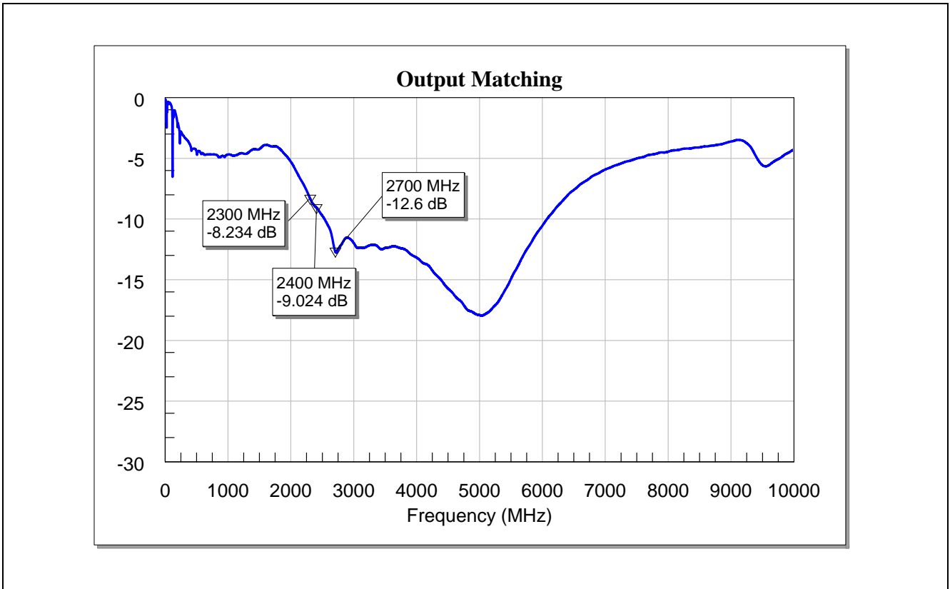
Figure 7 Output matching of the BFP720FESD for WLAN/Wimax at 2.3-2.7GHz
