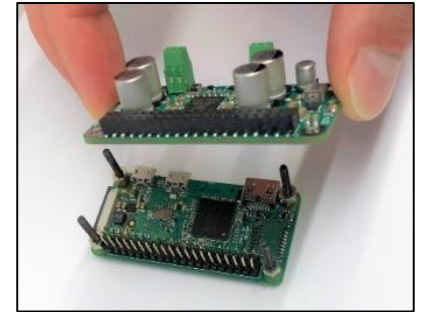
Figure 4. Assembly procedure of the Raspberry Pi + piHAT
