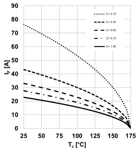
Figure 2. Diode forward current as function of temperature, parameter: T_{vj} \leq 175^\circ\text{C} , R_{th(j-c),max} , D =duty cycle, V_{th} , R_{diff} @ T_{vj}=175^\circ\text{C}
