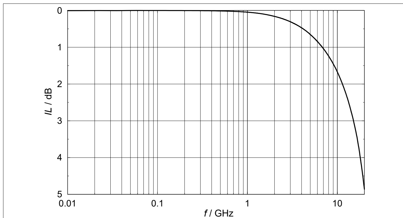
Figure 13 Insertion loss IL = f(f) , measured in a 50 \Omega system
