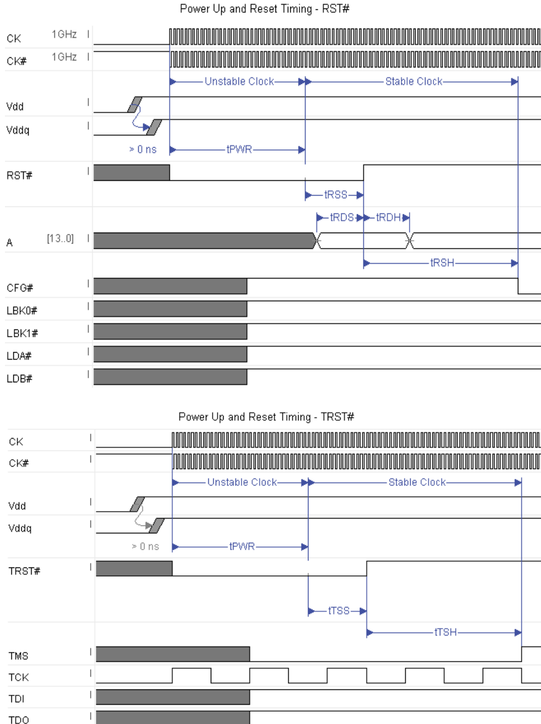
Figure 16. Reset Timings
