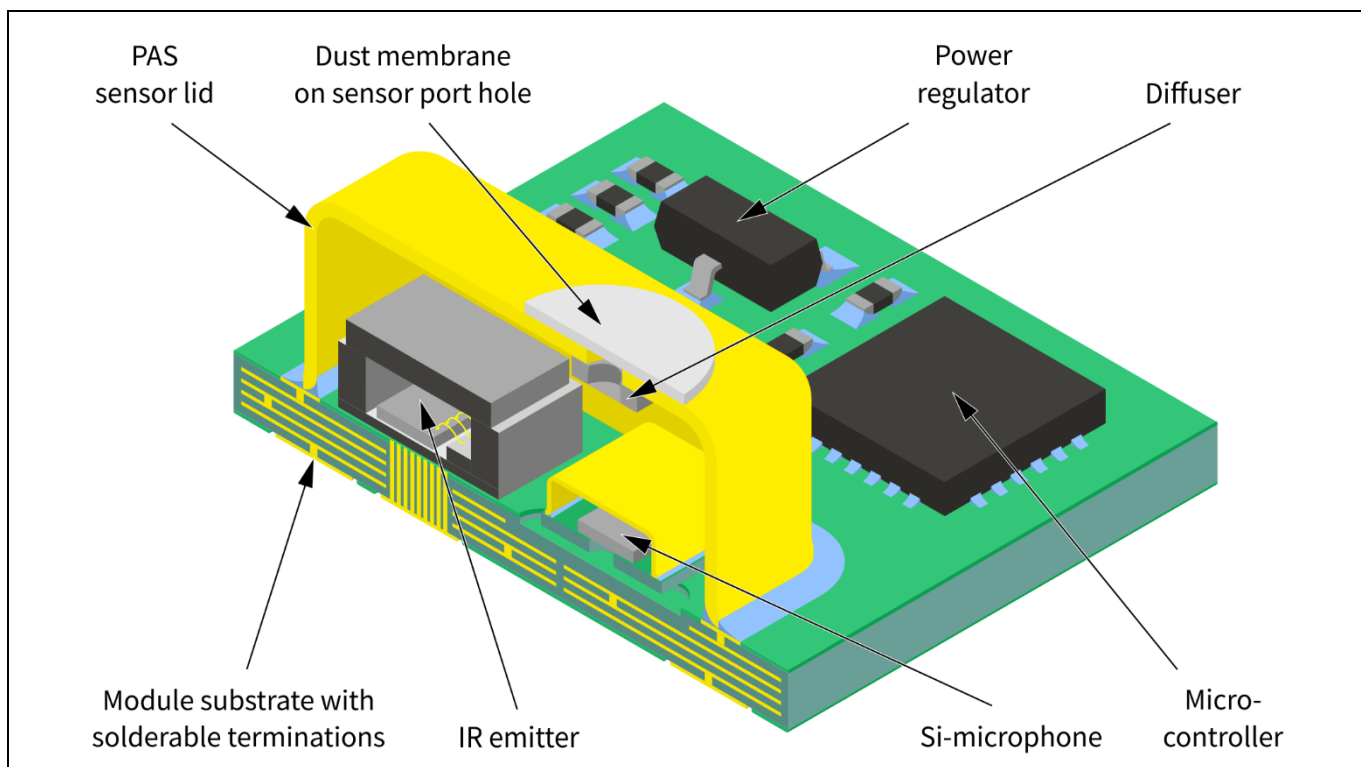
Figure 2 Schematic showing the inner setup of a PAS MLGA module.
