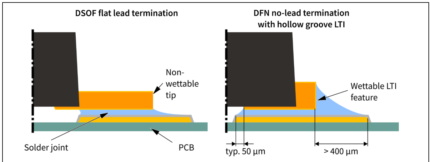
Figure 11 Schematic depictions of the DSOF flat lead solder joint (left) and the DFN no-lead solder joint with hollow groove LTI (right). The PCB pads for flat leads are mainly extended to their sidewall, whereas those for the no-lead terminations with hollow groove LTI are narrower and extended to the tip. The images are not to scale.
