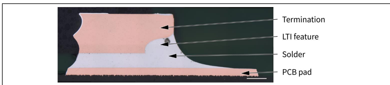
Figure 5 Cross section of a QFN component with "dimple" LTI termination.
