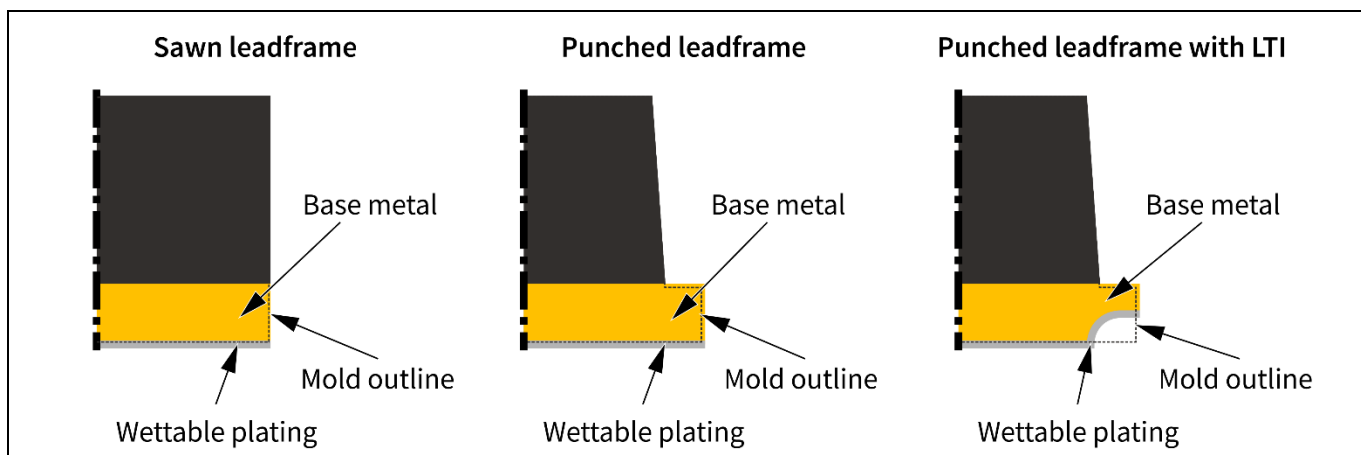
Figure 3 Schematic comparison of various QFN termination designs.
