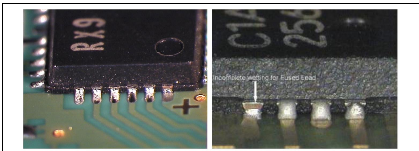
Figure 13 Photograph of terminations with (left) and without (right) LTI features that are fused with the pad.
