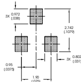
RECOMMENDED FOOTPRINT
