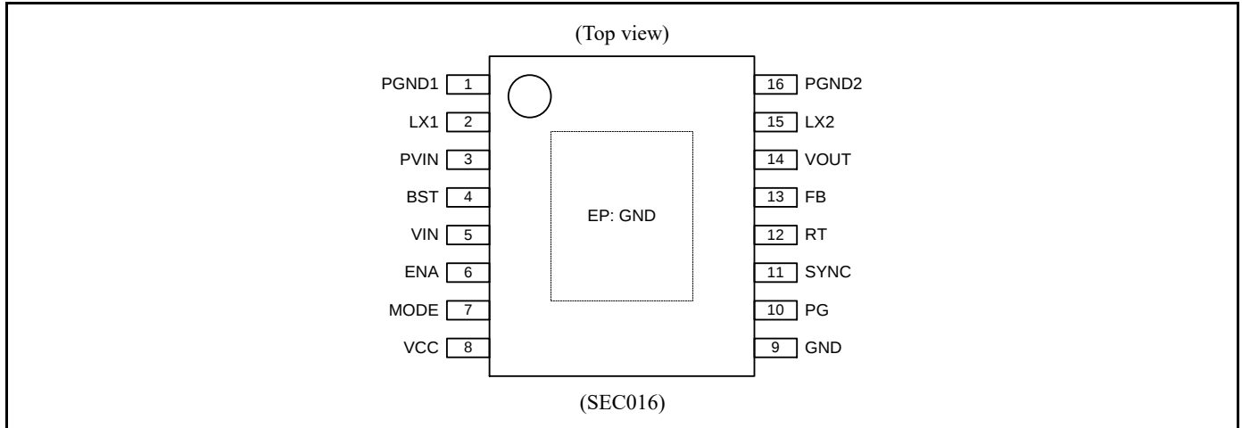
Figure 2-1 端子配列図
