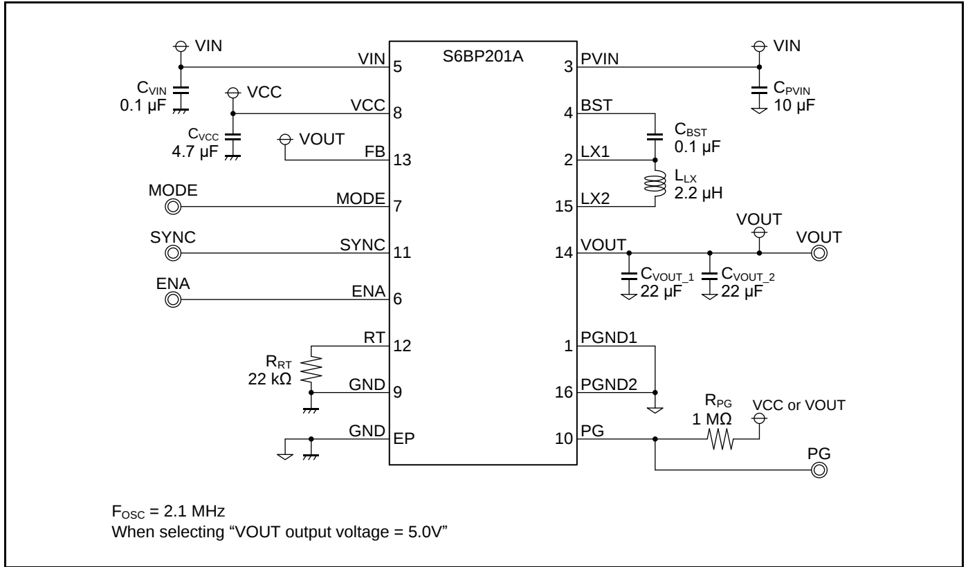
Figure 9-1 応用回路例
